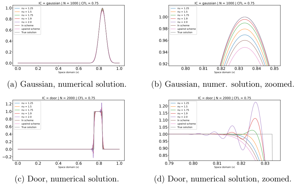
Figure 5.4 – Visualization of the numerical solutions associated to \nu -schemes, with smooth (Gaussian) and non smooth (door type) initial conditions.
