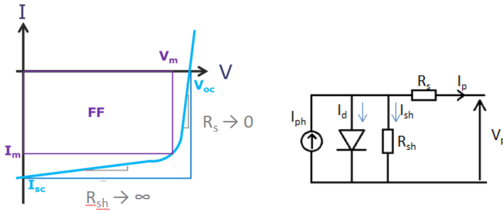
Fig.2-13: Current-voltage characteristics of solar cells under illumination which generates a photo-current I_{ph} ; I_d is the current of the diode, I_p is the current produced by the cell.
