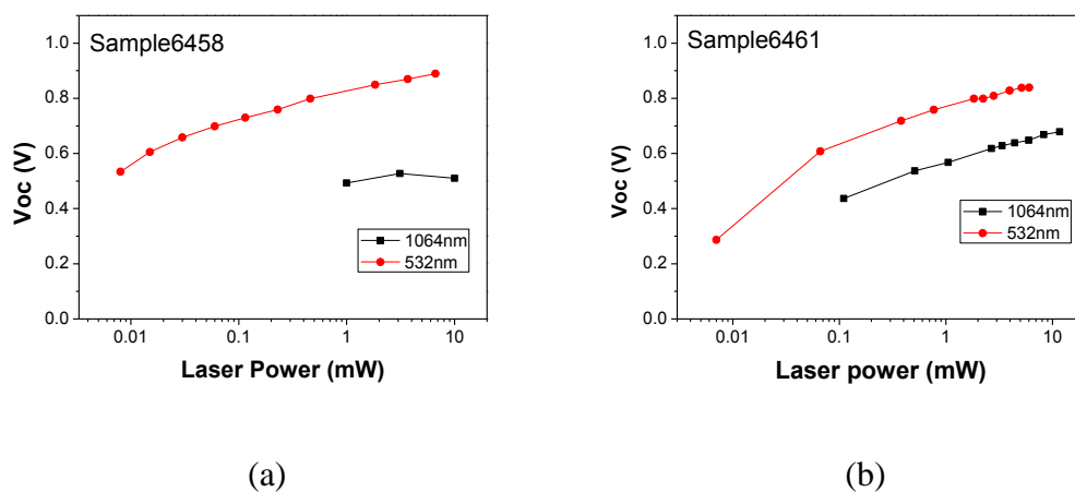
Fig. 4-29: V_{OC} values as a function of laser power under different wavelengths: (a) Sample-Barrier-6458; (b) Sample-SQW-6461.
