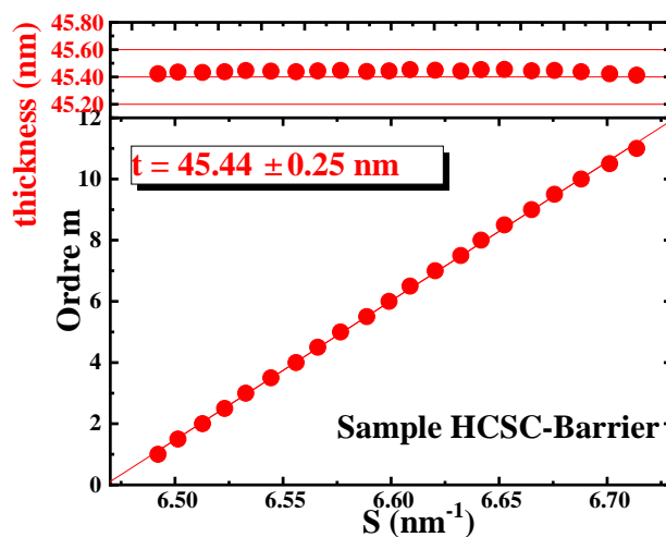
Fig. 4-17: Thickness fringes of Sample HCSC-Barrier.
