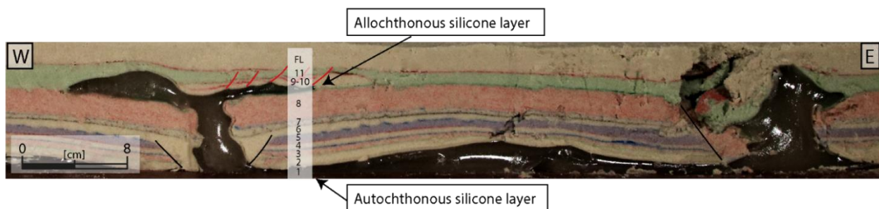
Figure 4.29: Section S01-03, at 7.2 cm from the southern limit of the box model. In black are interpreted the normal faults result of the simulated extensional tectonics and in red the normal faults above the overhang, result of the gravity gliding above the salt overhang. The numbers represent the layers deposited on the model (Table 4.1).
