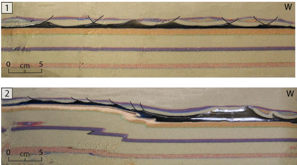
Figure 3.50: E-W sections A02-05 (1.) and A02-13 (2.), located respectively at 6.5 and 25.5 cm from the northern limit of the box model. In .1 the salt structures develop without the influence from the compressional stress, while in .2 the plateau uplift affects the silicone layer producing gravity gliding towards west.
