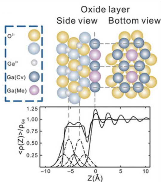
Figure 1-8 Schematic of the surface oxide of Ga, with the electron density profile plotted for the interface. Top: the projected atomic structure of gallium and gallium oxide layer where the atomic diameters for O^{2-} , Ga^{3+} , covalent (Cv) Ga and metal (Me) Ga is 2.64 Å, 1.24 Å, 2.44 Å and 2.50 Å, respectively. Bottom: the thin solid line represents the corresponding electron density profile with its different components; the underlying liquid Ga (large dash line) and the Gaussians representing the Ga^{3+} (dash-dotted line) and O^{2-} layers (short-dashed line) [176].
