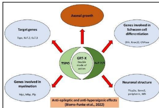
Scheme I. Representation of the GRT-X effects according to our results
