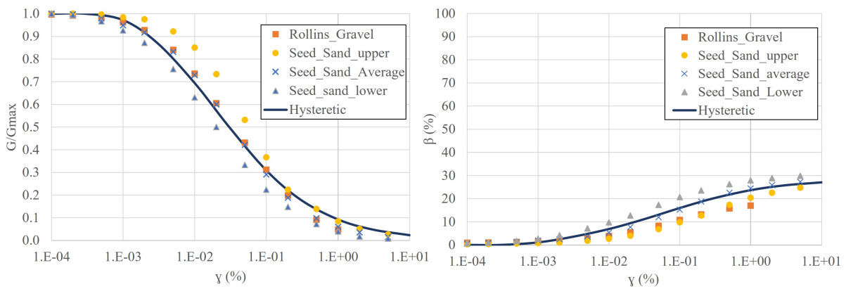
Fig. IV.6. Theoretical and numerical (Hysteretic) shear modulus degradation (left) and damping (right) curves for the moraine and alluvium
