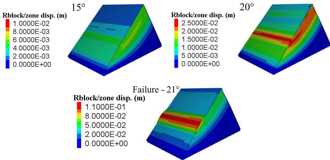
Fig. II.25. Displacement increments of the downstream pitching (composed of irregular blocks with bottom imperfection (20% contact)) at different tilting angles
