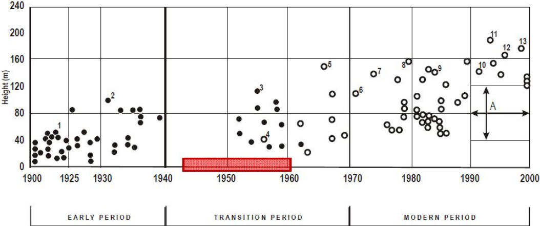
Fig. I.4. Development of the rockfill dam height throughout the 20th century: the red color represents the period when such dams were built in France [2]
