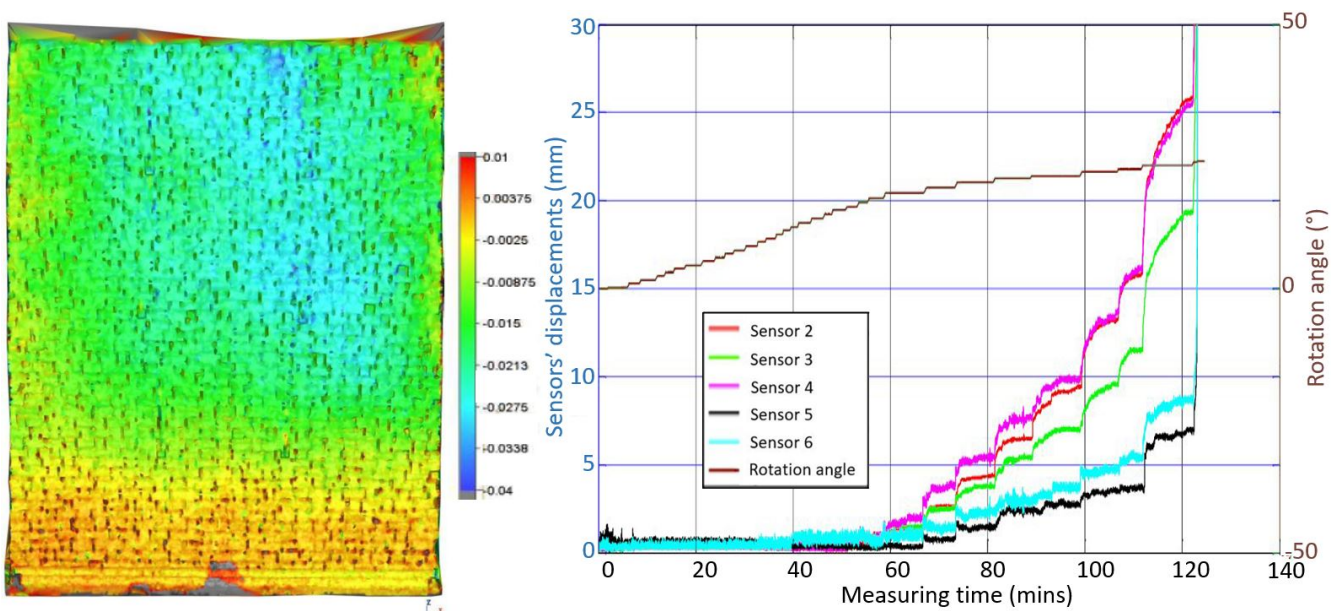
Fig. A.1. Dry stone pitching deformations of case 1 at bucket rotation angle of 23^\circ (just before failure) and sensor time displacements as a function of the bucket rotation angle
