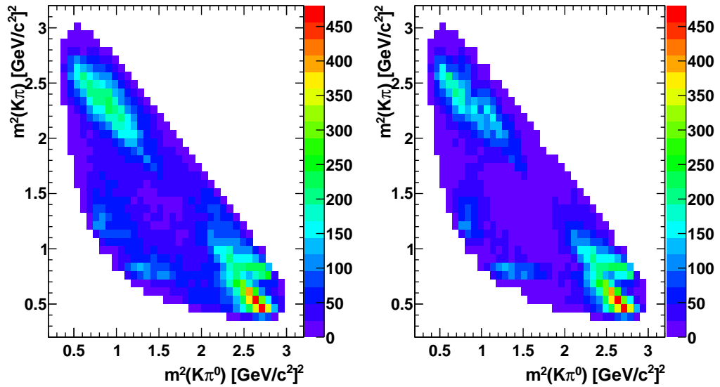
Figure 4.85: Distributions in the Dalitz plane ( m_{K\pi^0}^2, m_{K\pi}^2 ) of the candidates for Data Run 1 + Run 2, without the Dalitz Weight variable included in the five variables nominal MVA, and before selection (left) and after the selection cut on TMVA (85% efficiency applied).
