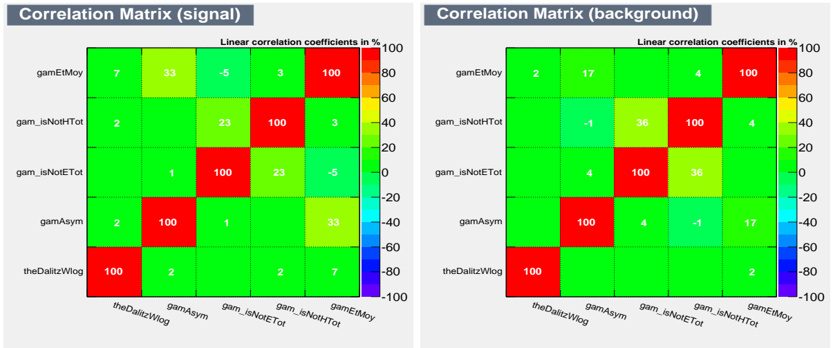
Figure 4.13: The correlation matrices of TMVA input variables for signal (left) and background (right).
