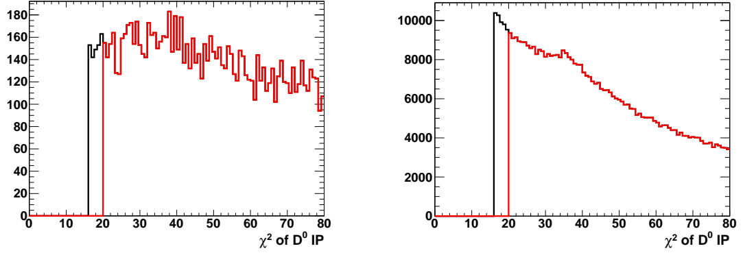
Figure 4.36: Selection on D^0 B PV IP \chi^2 for signal MC Run 2 (left) and background Data Run 2. Black curve represents before applying the D^0BPVIP\chi^2 and red curves are after the D^0BPVIP\chi^2 selection.
