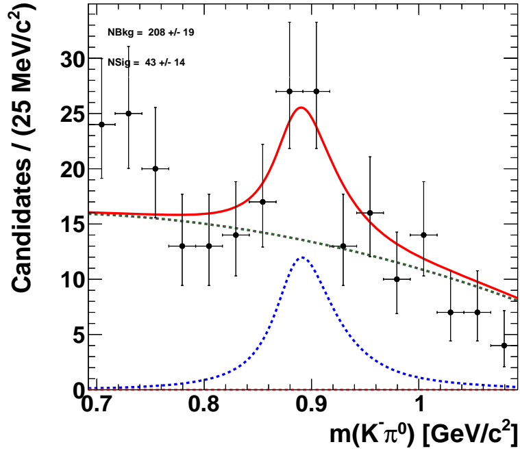
Figure 5.36: Fit to the invariant mass of K^{*0} \rightarrow K^- \pi^0 for DATA Run 1 and Run 2 in the sideband of the D .
