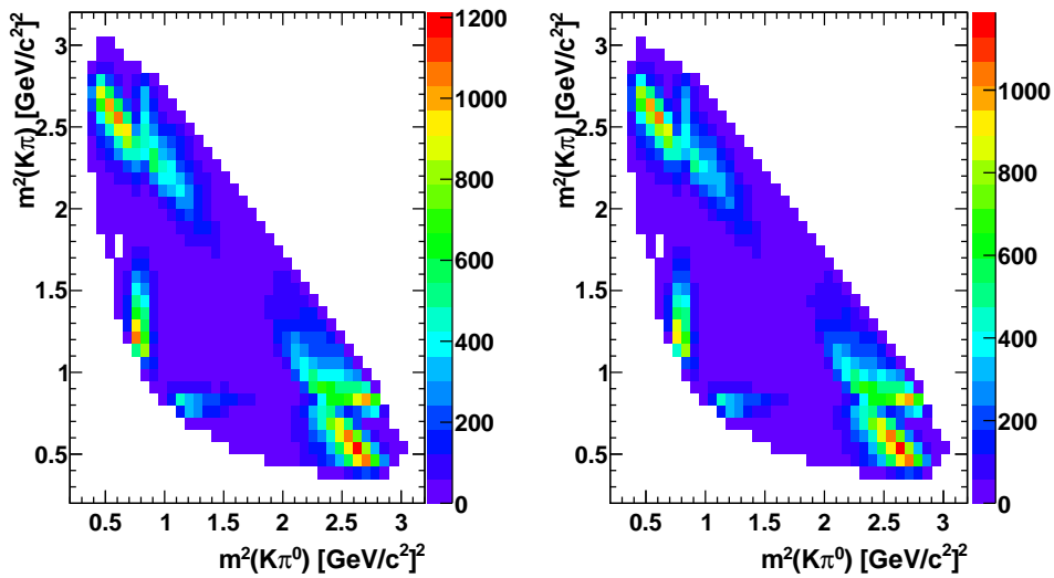
Figure 4.81: Distributions in the Dalitz plane ( m^2_{K\pi^0}, m^2_{K\pi} ) of the candidates for Run 1 + Run 2 MC simulation, without the Dalitz Weight variable included in the five variables nominal MVA, and before selection (left) and after the selection cut on TMVA (85% efficiency applied).
