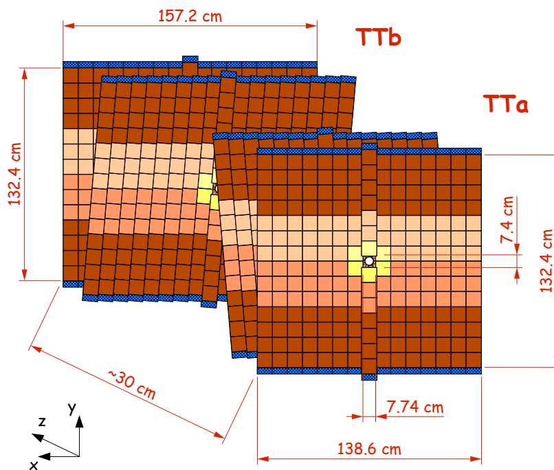
Figure 3.8: Layout of the four detection layers of the TT station. Figure is taken from [86].
