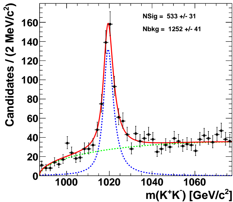
Figure 4.69: Fit to the invariant mass distribution of m(K^+K^-) for Run 1 + Run 2 Data with sPlot technique for D^0 \rightarrow K^+\pi\pi^0 (top) and D^0 \rightarrow K^-\pi\pi^0 (bottom). Data points are shown as black with error bars, the fitted total PDF is given with the red line. The component PDFs as dashed lines: (green) background and (blue) signal. PDFs parameters are fixed for Signal and Background.
