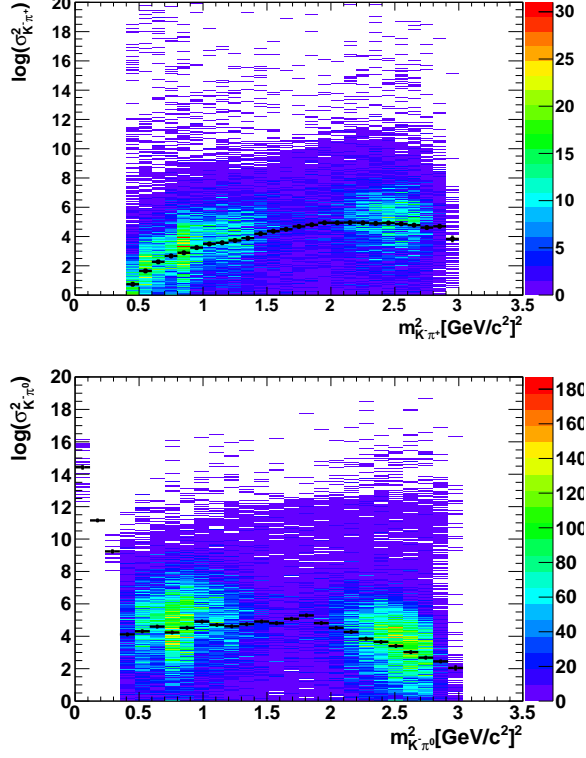
Figure 4.8: Resolution \sigma as a function of invariant mass squared of (a) m^2_{(K^-\pi^+)} (top) and (b) m^2_{(K^-\pi^0)} (bottom) for MC Run 2 signal.
