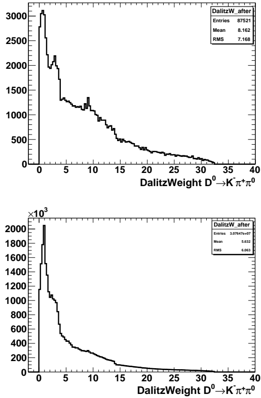
Figure 4.18: Dalitz Weight distribution after the BDT selection for Signal MC (top)(a) and Background Data Run 2 (bottom)(b).
