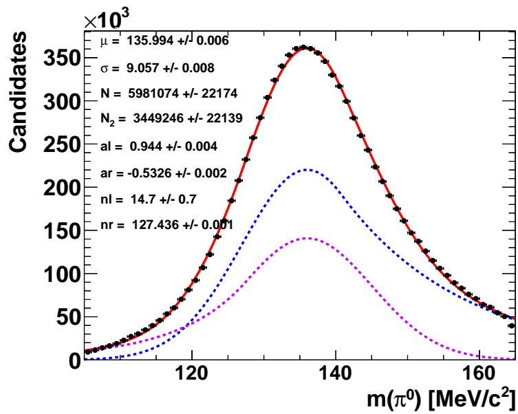
Figure 4.23: Optimisation the mass of \pi^0 for signal Data Run 2. The \pi^0 signal is fitted with a Right (R) and Left (L) side Crystal Ball function, while the two function share the same resolution ( \sigma ) and central value ( \mu ).
