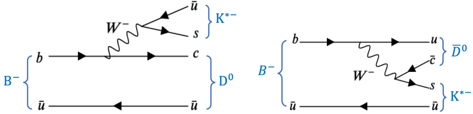
Figure 2.9: Feynman diagrams for B^- \rightarrow D^0 K^{*-} ( K^-\pi^0 ) decay (left) and B^- \rightarrow \bar{D}^0 K^{*-} ( K^-\pi^0 ). The interference between tree amplitudes favored b \rightarrow c (Vcb) and color suppressed b \rightarrow u (Vub).
