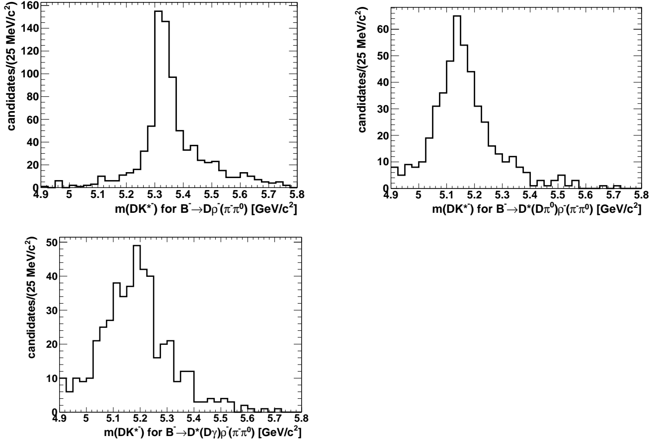
Figure 5.22: Mass distributions for the B^- \rightarrow D^{(*)}\rho^- background components for MC simulation. Upper left side distribution is for the B^- \rightarrow D^0\rho^-(\pi^-\pi^0) , upper right side is for the B^- \rightarrow D^*(D\pi^0)\rho^-(\pi^-\pi^0) and bottom distribution is for the B^- \rightarrow D^*(D\gamma)\rho^-(\pi^-\pi^0) .
