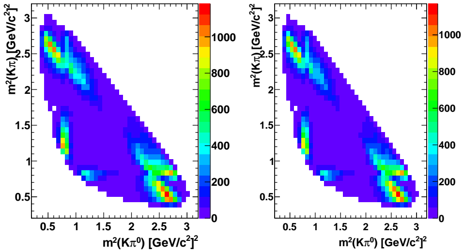
Figure 4.80: Distributions in the Dalitz plane ( m^2_{K\pi^0}, m^2_{K\pi} ) of the candidates for Run 1 + Run 2 MC simulation, with the Dalitz Weight variable included in the five variables nominal MVA, and before selection (left) and after the selection cut on TMVA (85% efficiency applied).
