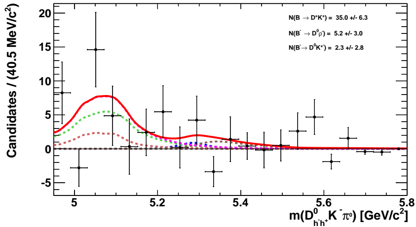
Figure 5.37: Fit to the invariant mass distribution to the B^- \rightarrow DK^{*0} ( K^- \pi^0 ) where D^0 decays D^0 \rightarrow K^+ \pi^- for DATA Run 1 and Run 2 in the sideband of the D .
