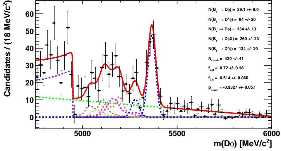
Figure 4.79: Fit to the invariant mass distribution of B_s^0 mass ( D\phi ) in the full Run 1 + Run 2 Data, mass range m_{DKK} \in [4750, 6000] \text{ MeV}/c^2 with sPlot technique. Data points are given in black with error bars, total PDF is displayed with the red line. The different contributions PDFs are given as dashed lines: (green) combinatorial background and (blue) signal B_s^0 \rightarrow D\phi , where D^0 \rightarrow K\pi\pi^0 . Small blue dashed B^0 \rightarrow D\phi , purple dashed is for B_s^0 \rightarrow D\phi X signal decay, the peaking contribution B_s^0 \rightarrow D^*\phi decay with magenta is for transverse and brown dashed longitudinal polarization.
