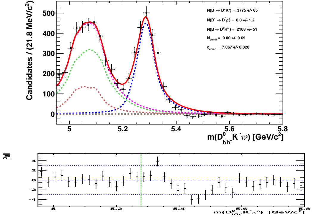
Figure 5.28: Fit to the invariant mass distribution of B^- \rightarrow D^0 K^{*-} (K^- \pi^0) , where D^0 decays to D^0 \rightarrow K^- \pi^+ (RS) for DATA Run 1 and Run 2 after sWeight subtraction. Signal shown in blue dashed curve and Data shown in black dots, partially reconstructed background shown B^- \rightarrow D^* K^* in green dashed curve, the peaking background B^- \rightarrow D^0 \rho^- is indicated with brown dashed curve and the overall fit is represented by the solid red line. The distribution of the pull shown beneath the fit distribution and represent the good agreement between the data and the fit functions.
