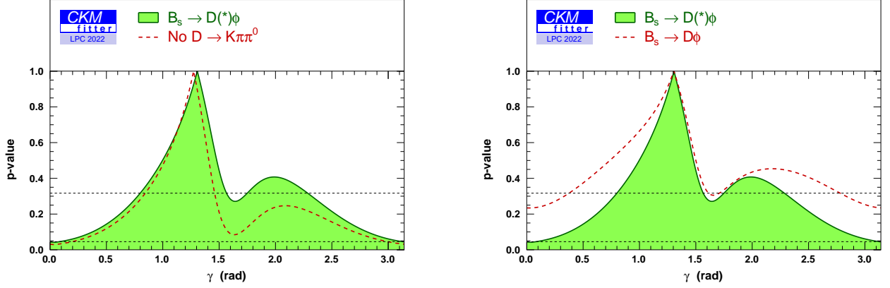
Figure 4.94: Profile of the p-value distribution of the global \chi^2 fit to \gamma after observables are computed, where the decay mode B_s^0 \rightarrow \tilde{D}^{(*)0}\phi is considered, where the D^0 decays to five sub-decay modes: KK , \pi\pi , K\pi , K3\pi , K\pi\pi^0 are taking into account. (Left) For the green curve fitted parameters: \gamma value at maximum is \gamma = 1.31_{-0.51}^{+0.26} rad and r_B = 0.19 , \delta_B = 0.86 rad ( 49.27^\circ ), r_B^* = 0.52 , \delta_B^* = 1.93 rad ( 111^\circ ). The B_s^0 \rightarrow \tilde{D}^{(*)0}\phi decay without sub-decay mode K\pi\pi^0 is shown with the dashed red line superimposed to the same distribution. The fitted parameters: \gamma value at maximum is \gamma = 1.27_{-0.43}^{+0.19} rad, r_B = 0.21 , \delta_B = 0.56 rad ( 32^\circ ), r_B^* = 0.56 , \delta_B^* = 1.96 rad ( 112^\circ ). (Right) The B_s^0 \rightarrow \tilde{D}^{(*)0}\phi decay without B_s^0 \rightarrow D^*\phi is shown with the dashed red line superimposed to the same distribution. Fitted parameters for the B_s^0 \rightarrow D\phi : \gamma = 1.30_{-0.93}^{+0.31} rad, r_B = 0.19 , \delta_B = 0.85 rad ( 49^\circ ). The horizontal two dashed black lines refer to 68.3 % ( 1\sigma ) and 95.4 % CL ( 2\sigma ).
