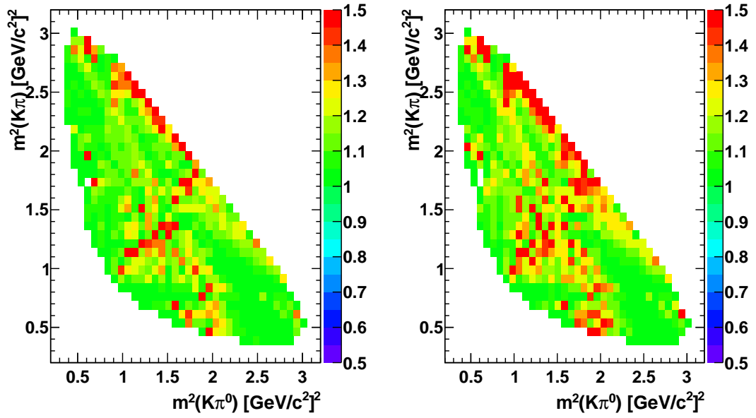
Figure 4.82: Distributions in the Dalitz plane ( m^2_{K\pi^0} , m^2_{K\pi} ) of the candidates for Run 1 + Run 2 MC simulation, with (left) and without (right) Dalitz weight.
