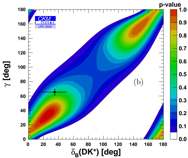
Figure 5.57: Two-dimension contour plots of the fitted physics parameters r_B (a) and \delta_B (b) as a function of \gamma . LHCb \gamma combination [2] is shown with the straight black line.
