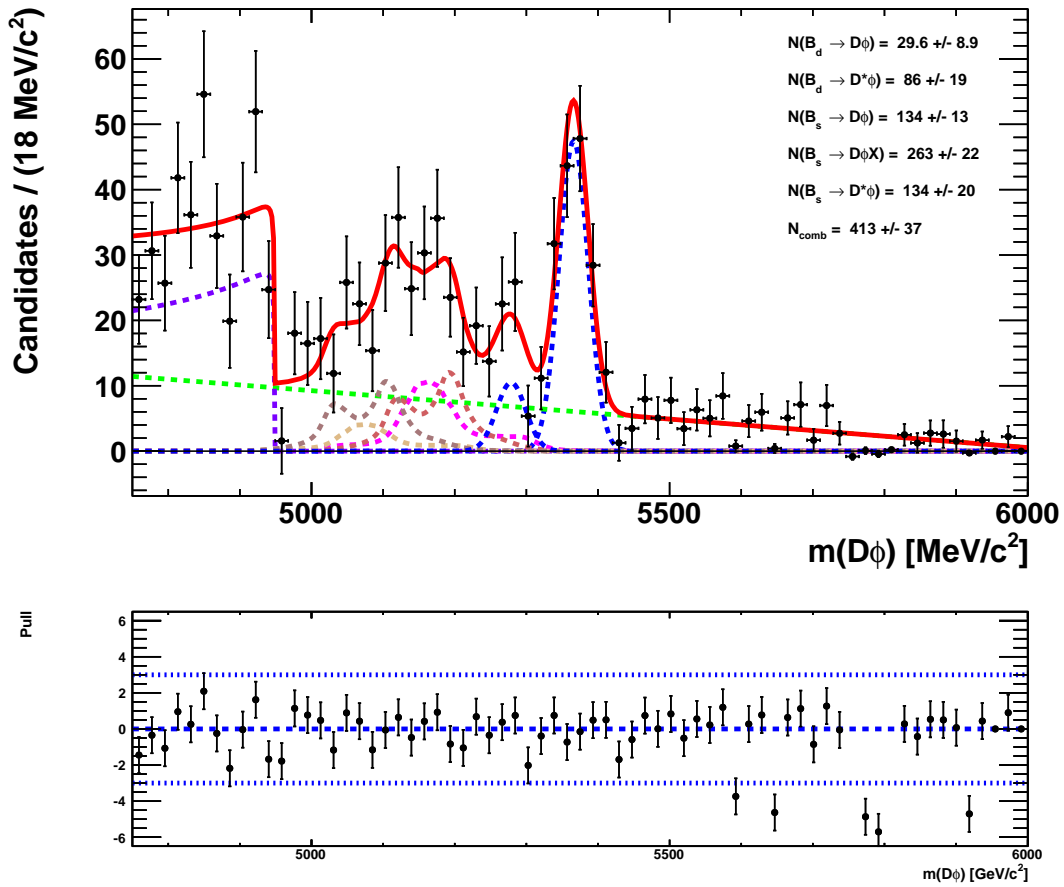
Figure 4.71: Fit to the invariant mass distribution of B_s^0 mass ( D\phi ) in the full Run 1 + Run 2 Data, mass range m_{DKK} \in [4750, 6000] MeV/c 2 with sPlot technique. Data points are shown as black with error bars, total PDF is displayed with the red line. The different contributions PDFs are given as dashed lines: (green) combinatorial background and (blue) signal B_s^0 \rightarrow D\phi , where D^0 \rightarrow K\pi\pi^0 . Small blue dashed B^0 \rightarrow D\phi , purple dashed is for B_s^0 \rightarrow D\phi X signal decay, the peaking contribution B_s^0 \rightarrow D^*\phi decay with magenta is for transverse and brown dashed longitudinal polarization.
