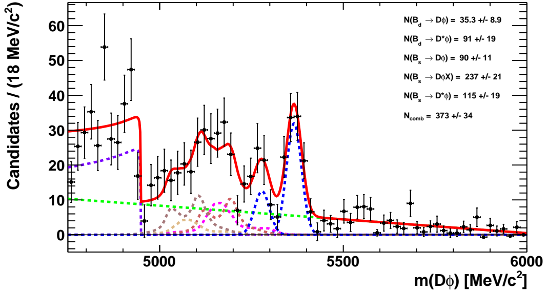
Figure 4.89: Fit to the invariant mass distribution of B_s^0 mass ( D\phi ) in the full Run 1 + Run 2 Data, mass range m_{DKK} \in [4750, 6000] \text{ MeV}/c^2 with sPlot technique. Data points are shown as black with error bars, total PDF is displayed with the red line. The different contributions PDFs are given as dashed lines: (green) combinatorial background and (blue) signal B_s^0 \rightarrow D\phi , where D^0 \rightarrow K\pi\pi^0 . Small blue dashed B^0 \rightarrow D\phi , purple dashed is for B_s^0 \rightarrow D\phi X signal decay, the peaking contribution B_s^0 \rightarrow D^*\phi decay with magenta is for transverse and brown dashed longitudinal polarization.
