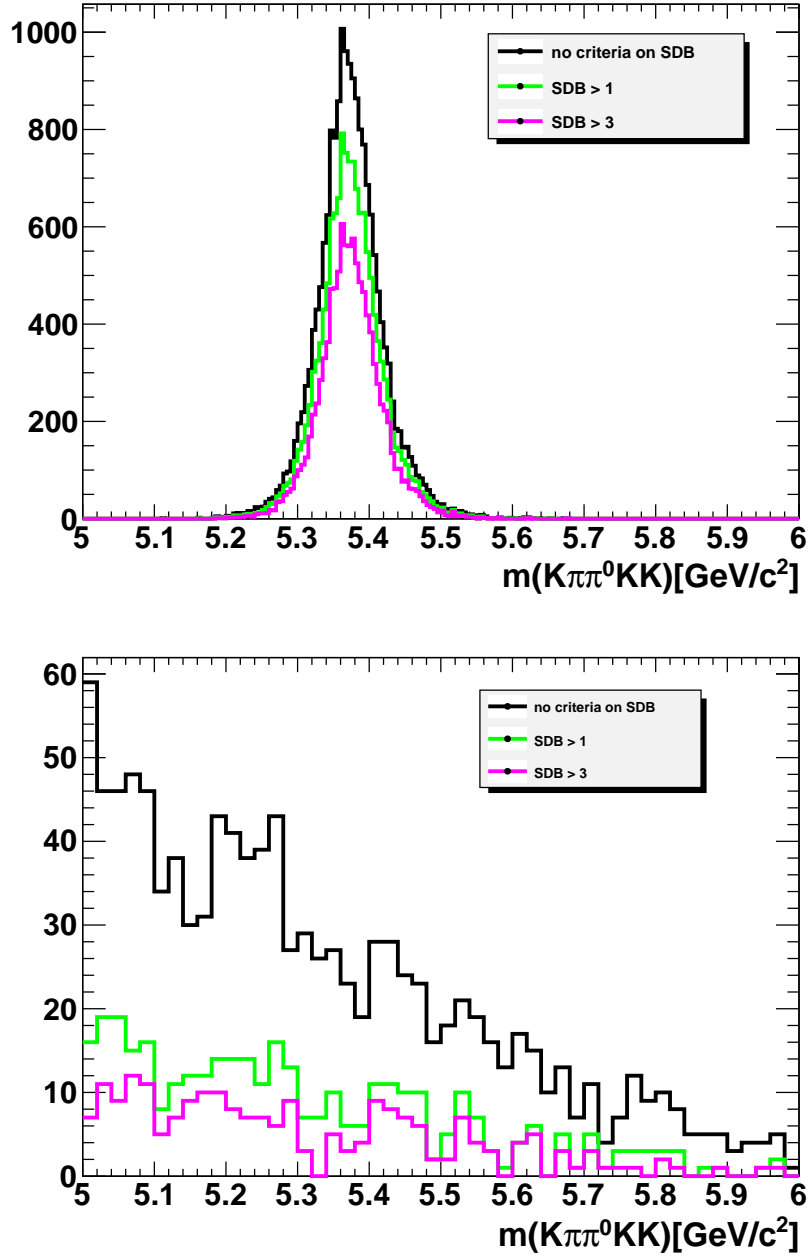
Figure 4.47: SDB selection on the invariant mass distribution of B_s^0 in the D sidebands and m_{KK} < 1080 MeV for signal MC Run 1 (top) and background Data Run 1 (bottom).
