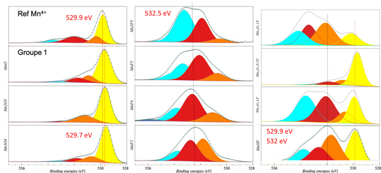
Figure 167. Spectre O1s.
