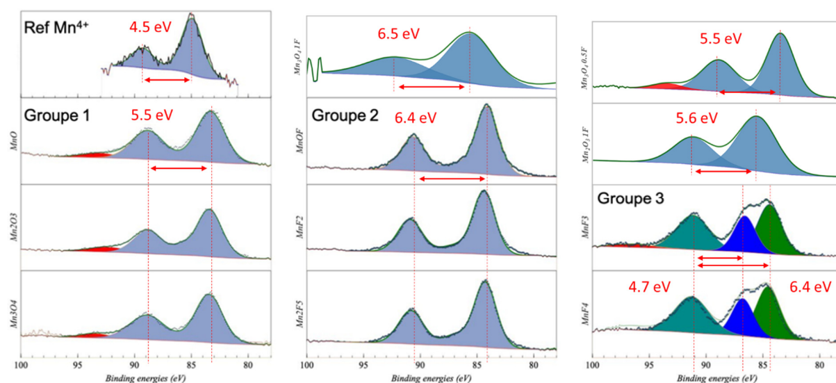
Figure 169. Spectres Mn3s.
