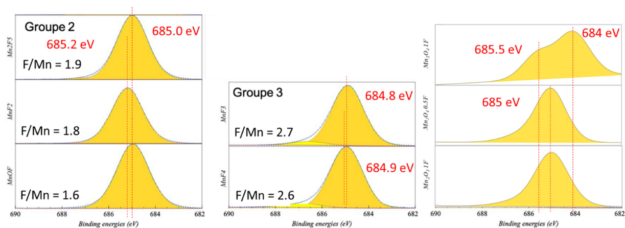
Figure 168. Spectres F1s.
