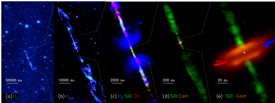
FIGURE 1.9: Different scales of the HH212 protostellar jet (Lee, 2020). (a): Reipurth et al., 2019, (b) and (c): Lee et al., 2015; McCaughrean et al., 2002, (d) and (e): Lee et al., 2017. The observed molecules and their associated colors are at the bottom.
