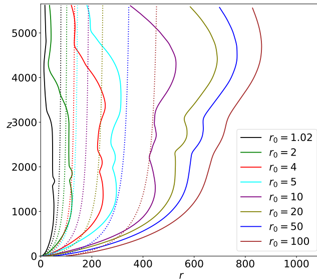
FIGURE 6.6: Evolution of several magnetic field lines during the simulation computation, for different anchoring radii r_0 . The field lines at the first output of the simulation (initial conditions) are shown in dotted lines. The field lines at the last output of the simulation (final state) are shown as full lines.
