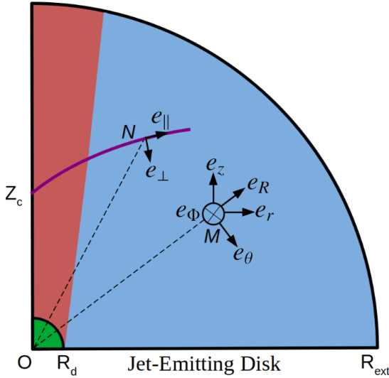
Fig. 1. Sketch of our computational domain. The central object and its interaction with the innermost disk are located below the inner boundary at R_d (green region), the near-Keplerian jet-emitting disk (JED) being established from R_d to the end of the domain R_{\text{ext}} . An axial outflow (the spine) is emitted from the central regions (in red) and the jet is emitted from the JED (in blue). The solid purple line represents a recollimation shock surface starting on the axis at a height Z_c . For each point N lying on this surface, we use local poloidal unit vectors ( \mathbf{e}_\perp, \mathbf{e}_\parallel ), respectively perpendicular and parallel to the shock surface. Also, at any point M inside the domain, we either use spherical ( \mathbf{e}_R, \mathbf{e}_\theta, \mathbf{e}_\phi ) or cylindrical ( \mathbf{e}_r, \mathbf{e}_\theta, \mathbf{e}_z ) coordinates.
