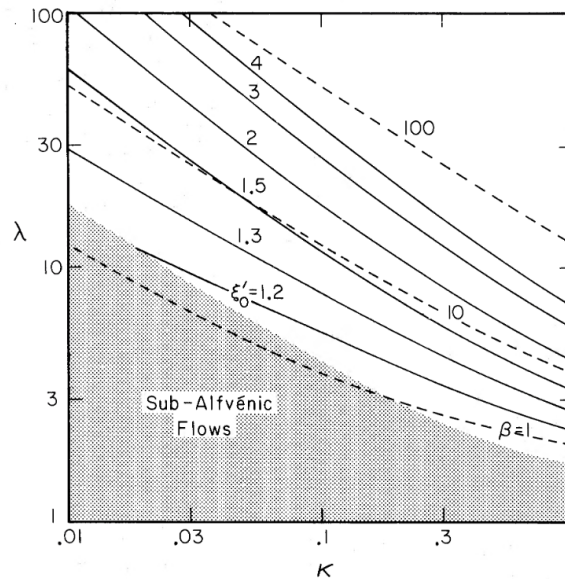
FIGURE 2.3: Values of \lambda and \kappa for the solutions of Blandford and Payne, 1982. The parameter \zeta'_0 \equiv B_r/B_z is the inclination of the magnetic field lines on the disk surface. The parameter \beta \equiv \kappa(2\lambda - 3)^{3/2} relates to the asymptotic collimation of the solution.
