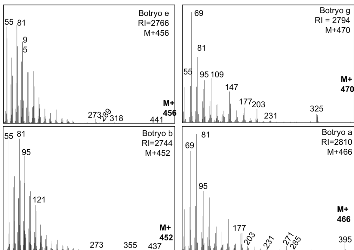
Figure 54: Mass spectrum of the four most abundant botryococcenes. The molecular ion ( M^+ ) usually presents a really low intensity but was detectable in some of the samples. We indicate the Kovat retention index for each compound.
