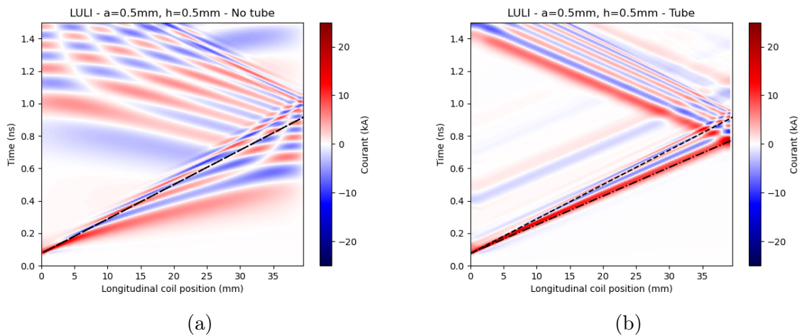
Figure 5 – PIC simulation of the current pulse intensity in kA for a helical coil (a) without tube and (b) with tube as a function of time and along the HC axis. The particles features are defined in Table 2.2 for LULI. The HC parameters are: length L = 40 mm, radius in the heart of the coil a = 0.5 mm, external radius 0.6 mm and step h = 0.5 mm with a tube of radius b = 0.9 mm. The dashed line corresponds to V_{HC} , the geometrical speed of the HC, the dash-dotted line corresponds to V = 1.2 V_{HC} .
