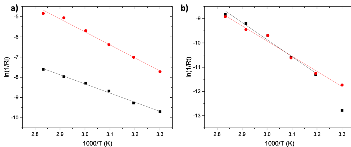
Figure SI.IV-3. Arrhenius plot of the interfacial resistance (a) R_i and (b) R_t for (■) in-situ LiTFSI-Multilayer and (●) ex-situ LiTFSI-Multilayer.
