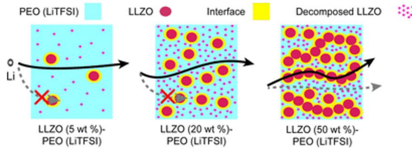
Figure I-18. Schematics of Li-ion diffusion pathways in PEO(LiTFSI)/LLZO SCEs for different LLZO weight proportion 98 .
