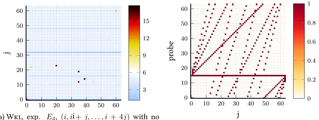
(a) WKL, exp. E_4, (i, i+j, \dots, i+4j) with no prefetcher: average number of hit in the page for i and j . (b) WKL, exp. E_4, (i, i+j, \dots, i+4j) with no prefetcher: hit rate in each line in the page for j , with i = 15 .
