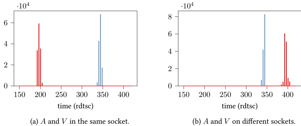
Figure 5.5.: Histograms of hit (red) and miss (blue, around 340) c1flush timing distributions for two different (A, V) pairs on a 2x Intel Xeon E5-2630 v3 machine.
