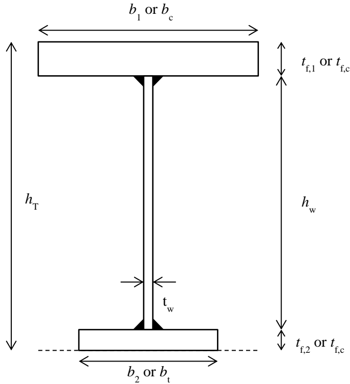
Figure VII-20: Cross-section dimensions
