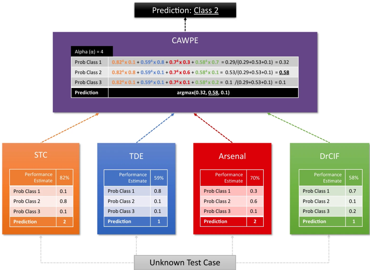
Figure 2.6: How the HIVE-COTE 2 ensemble predict the class of a time series. Image from the original paper of [58]
