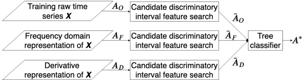
Figure 2.2: Overview of the approach taken by the Supervised Time series Forest. Image from the original paper of [14]. A_O, A_F, A_D are the spaces of possible interval features for each representation. \bar{A}_O, \bar{A}_F, \bar{A}_D are the feature spaces after a feature selection step.
