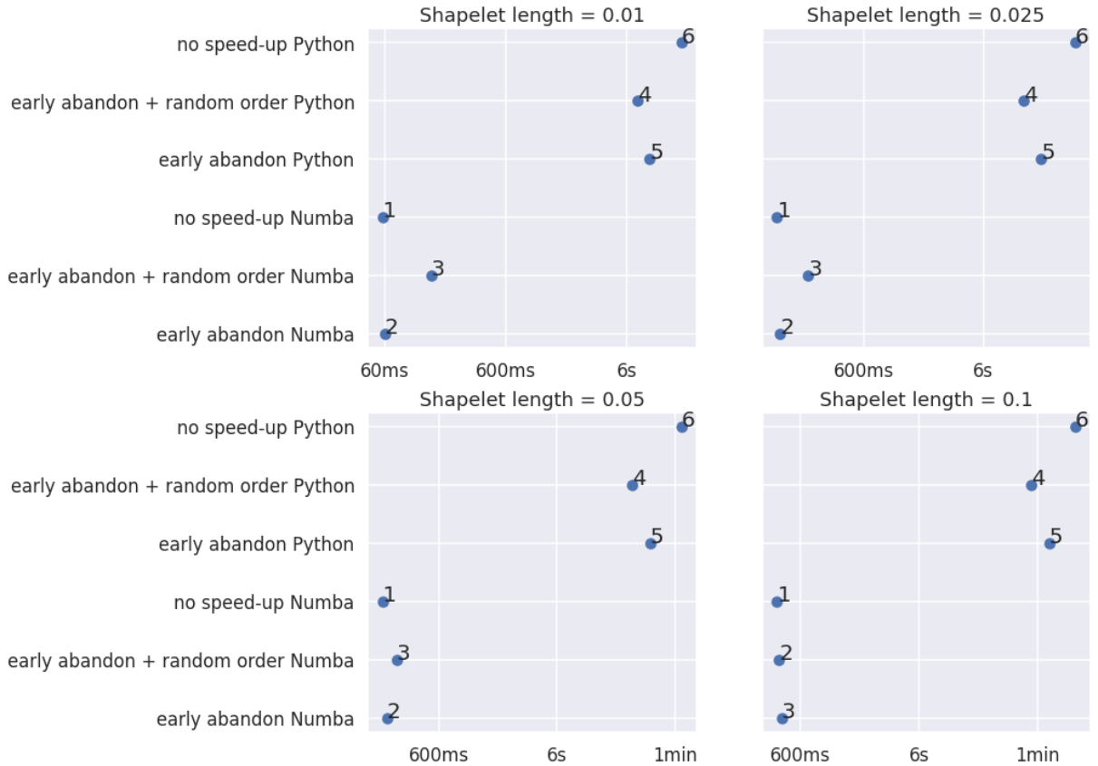
Figure 3.32: Total time to slide a randomly sampled shapelet, for different shapelet sizes (relative to the input length as [m \times l] ), on 43 datasets of the UCR archive, averaged over 10 runs for 100 different shapelets. The number next to each point is its rank.
