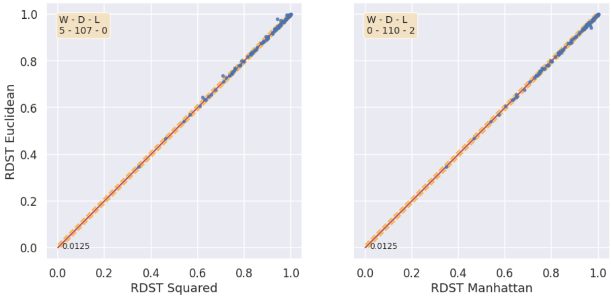
Figure 3.18: Pairwise accuracy plot for RDST using the Euclidean distance against RDST with the squared Euclidean and Manhattan distances, a margin of \pm 1.25\% of accuracy to count draws. Both figures share the y-axis.
