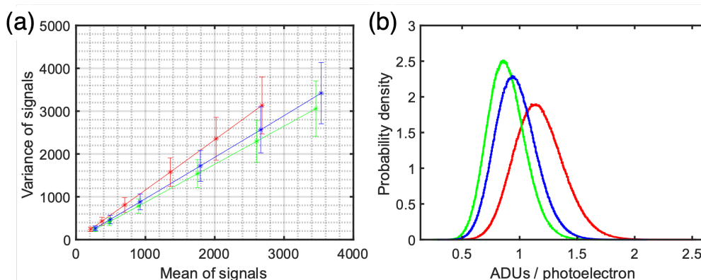
Figure 3.13 (a) The linear model (3-10) for 2064×1544 pixels. The error bars represent the standard deviation. (b) The histogram of the conversion factor for 2064×1544 pixels.
