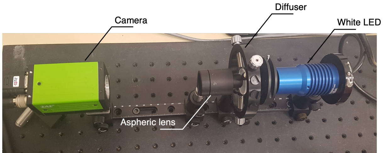
Figure 3.12 The experimental configuration for the measurement of the conversion factor. A wide gaussian beam created by the diffuser and lens is illuminated on the camera. The images were acquired without the objective lens.
