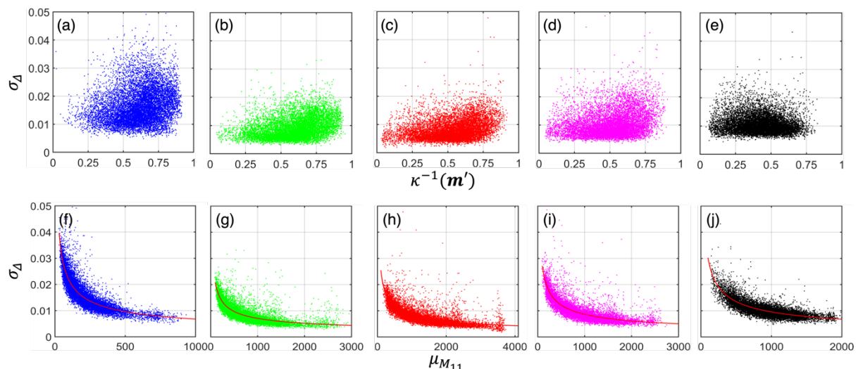
Figure 4.14 (a-e) the condition number of m' is not related to the standard deviation of depolarization \sigma_{\Delta} . (f-j) \sigma_{\Delta} is a function of intensity \mu_{M_{11}} . \sigma_{\Delta} can be fitted by the nonlinear model (4-1).
