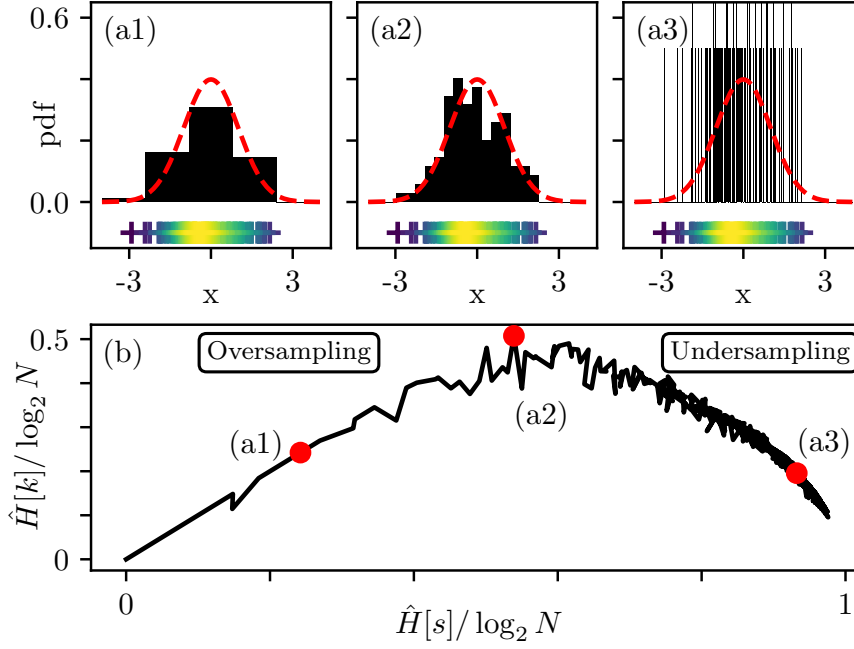
Figure 2.1: Relevance analysis of a Gaussian distribution sample ( N = 100 ). (a) Influence of the number of bins n on the normalized histogram (black bars), for (a1) n = 5 , (a2) n = 23 and (a3) n = 400 . The red curve corresponds to the underlying distribution. The bottom markers (+) represent the initial sample data points with color indicating local data density. (b) Resolution/Relevance curve.
