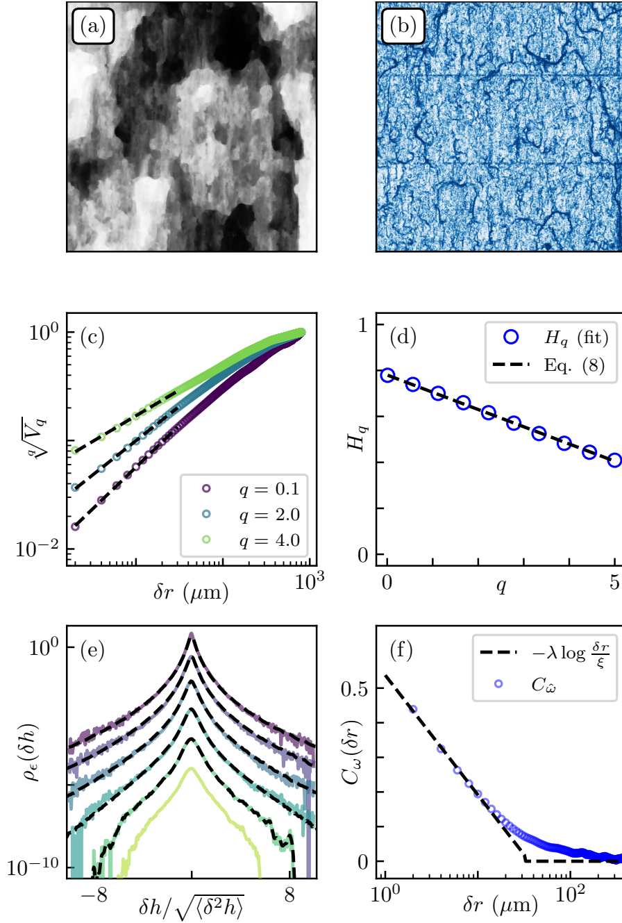
Figure 4.4: Unwrapping of an experimental multi-affine field. (a) Height map h(r) of a fractured metallic alloy of size 2 \times 2 mm 2 with 2 \mu\text{m}/\text{pixel} . (b) \hat{\omega}(r) field, retrieved from Eq. (4.9). (c) Rescaled variograms. (d) Comparison of the exponents H_q = \zeta_q/q with the prediction of Eq. (4.8) using H = 0.63 and \lambda = 0.15 . (e) Distribution of fluctuations computed at scales \epsilon/\zeta = 1/16, 1/8, 1/4, 1/2, 1 and 2 and their comparison with the distributions computed from Eq. (4.10) using L = \zeta . (f) Correlations of \hat{\omega} and comparison with the expected correlations using \lambda = 0.15 and \zeta = 33 \mu\text{m} .
