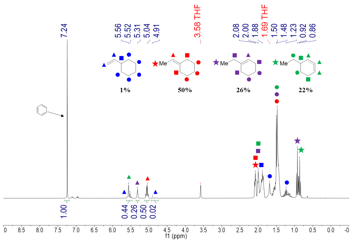
Figure A17. ^1\text{H} NMR spectrum in \text{thf-}d_8 of the isomerization of D by 1 mol% of 1 at 60\text{ }^\circ\text{C} , t=5.5 days. Relevant peaks are assigned and benzene served as an internal reference.
