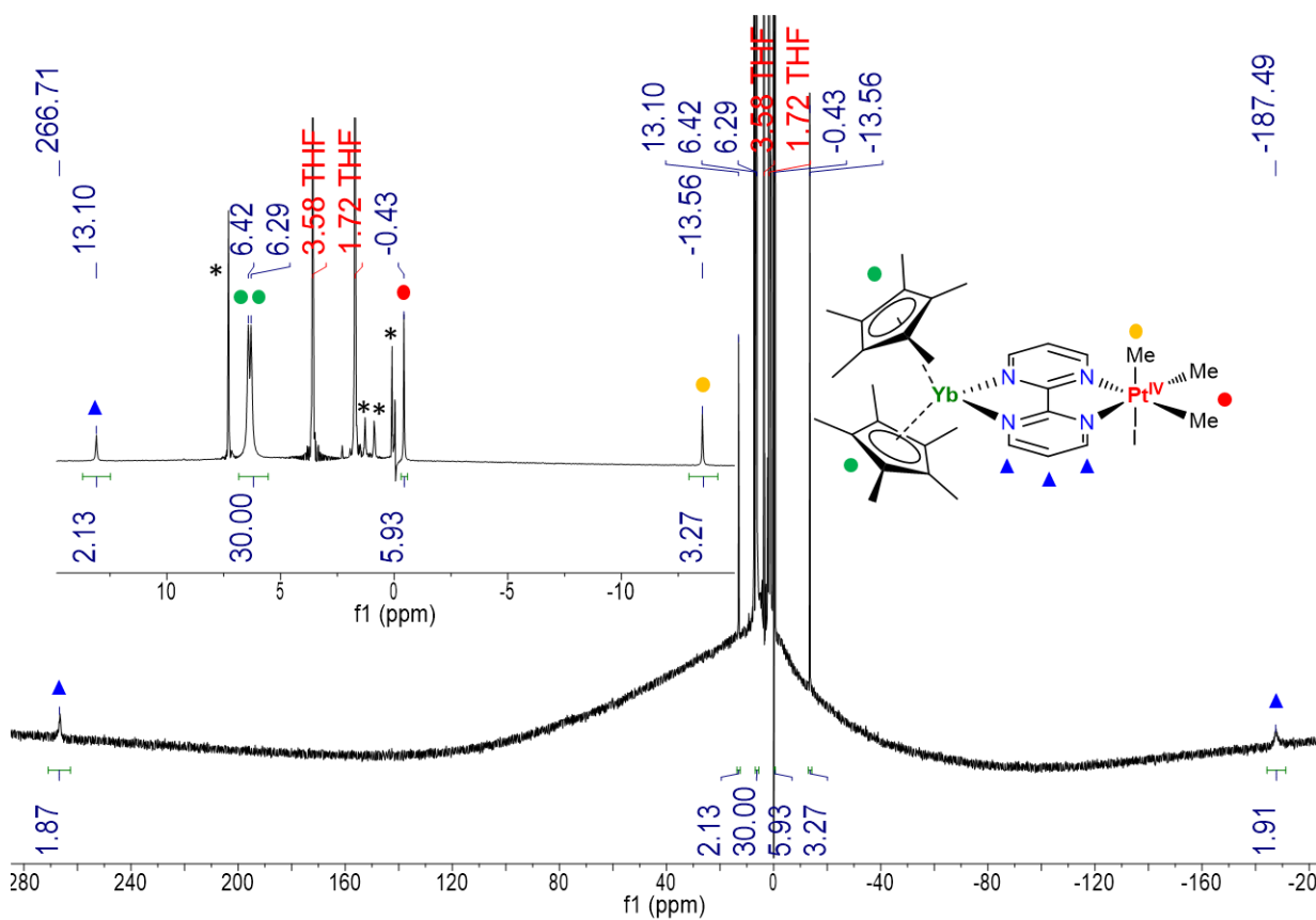
Figure II.4. ^1\text{H} NMR spectrum of 3 recorded at 20 °C in \text{thf-}d_8 . Asterisks are labeling benzene, pentane and silicon grease impurities from left to right respectively.
