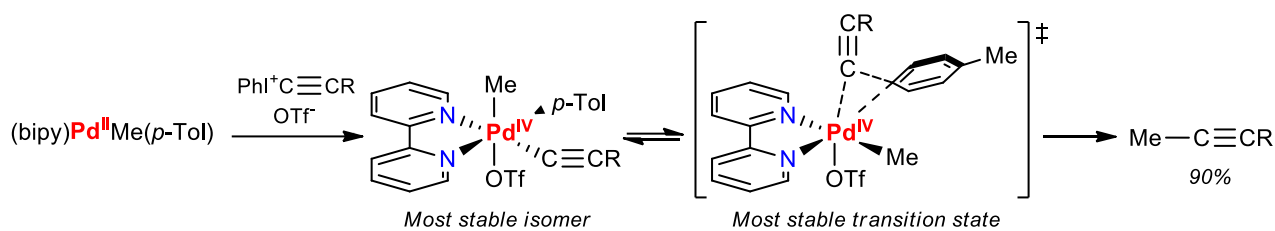
Figure I.7. Preference for the formation of the alkyne-alkyl product due to the most stable intermediate.
