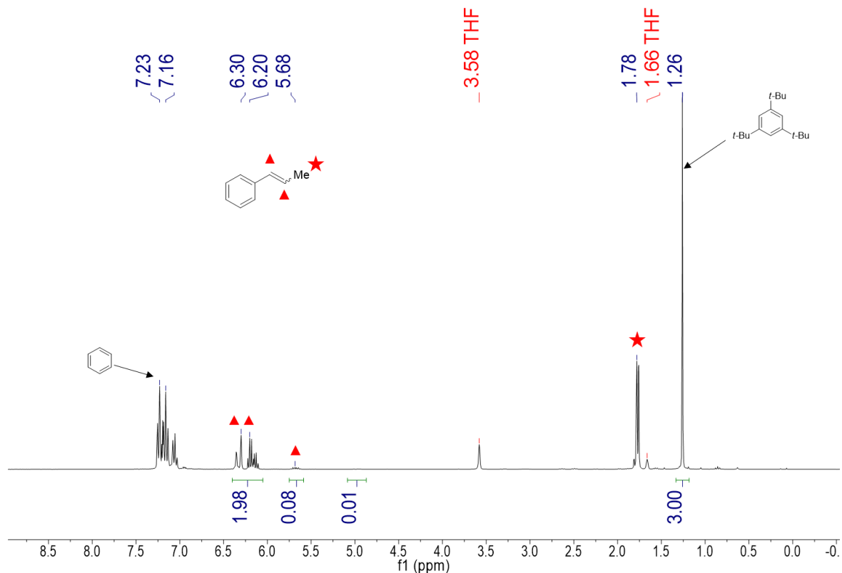
Figure A5. ^1\text{H} NMR spectrum in \text{thf-}d_8 of the isomerization of A by 1 mol% of 1 at 60\text{ }^\circ\text{C} , t=16\text{ h} . Relevant peaks are assigned and (t\text{Bu})_3\text{benzene} served as an internal reference.
