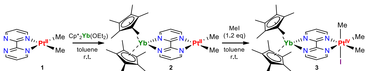
Figure II.1. Synthesis of Cp* 2 Yb(bipym)PtMe 2 , 2 and Cp* 2 Yb(bipym)PtMe 3 I, 3 .
