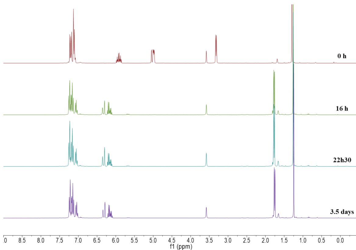
Figure A6. ^1\text{H} NMR spectrum in \text{thf-}d_8 of the isomerization of A by 1 mol% of 1 at 60^\circ\text{C} , t=3.5 days. Relevant peaks are assigned and (t\text{Bu})_3\text{benzene} served as an internal reference.
