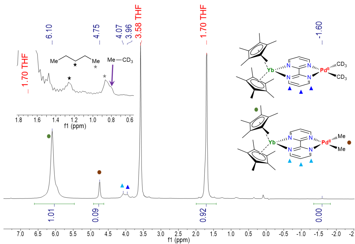
Figure III.7. Ligand exchange between the 2\text{-}d_{12} and \text{Cp}^*_2\text{Yb}(\text{bipym})\text{PdMe}_2 complexes, t = 4.5 days.
