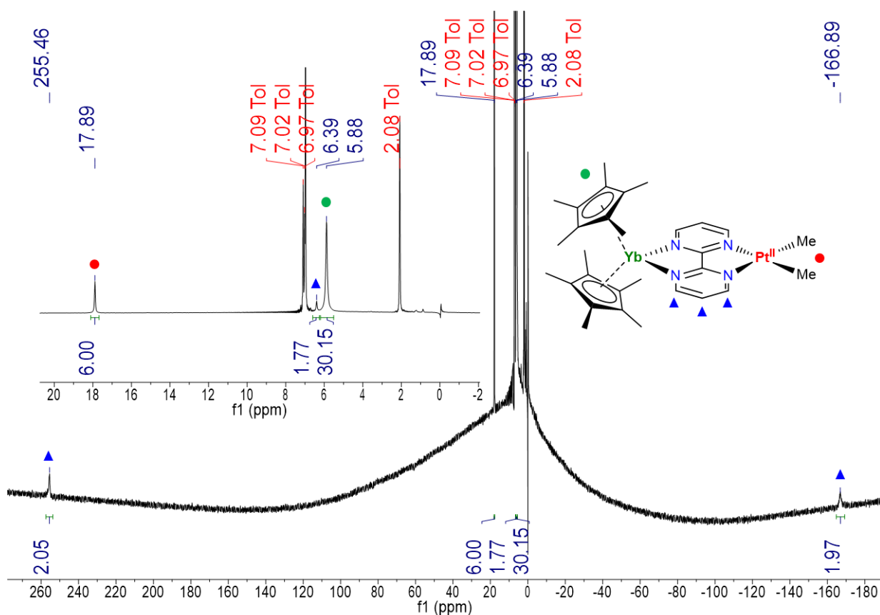
Figure II.3. ^1\text{H} NMR spectrum of 2 recorded at 20 °C in \text{tol-}d_8 .
