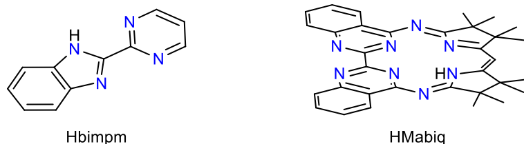
Figure III.8. The Hbimpm and HMabiq ligands recently used to synthesize heterobimetallic complexes.
