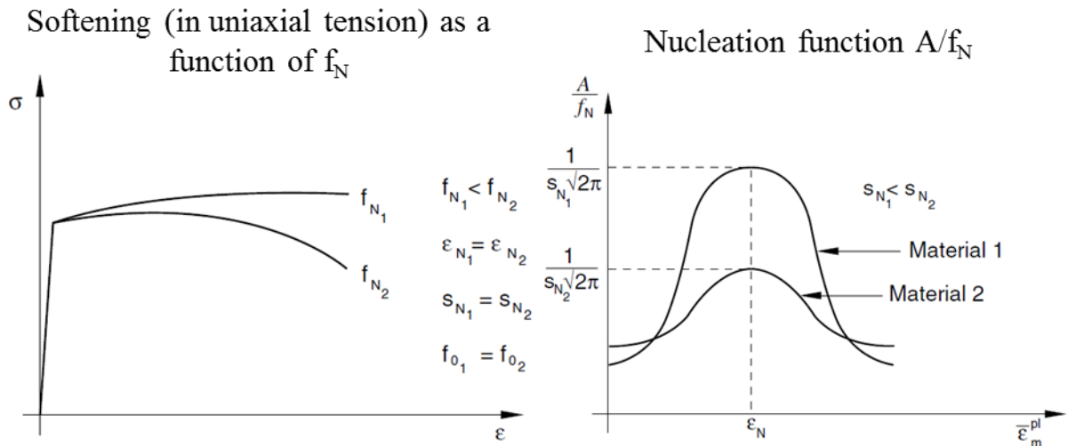
Figure III–78 Material's behaviour according to the GTN model in function of its parameters [58].
