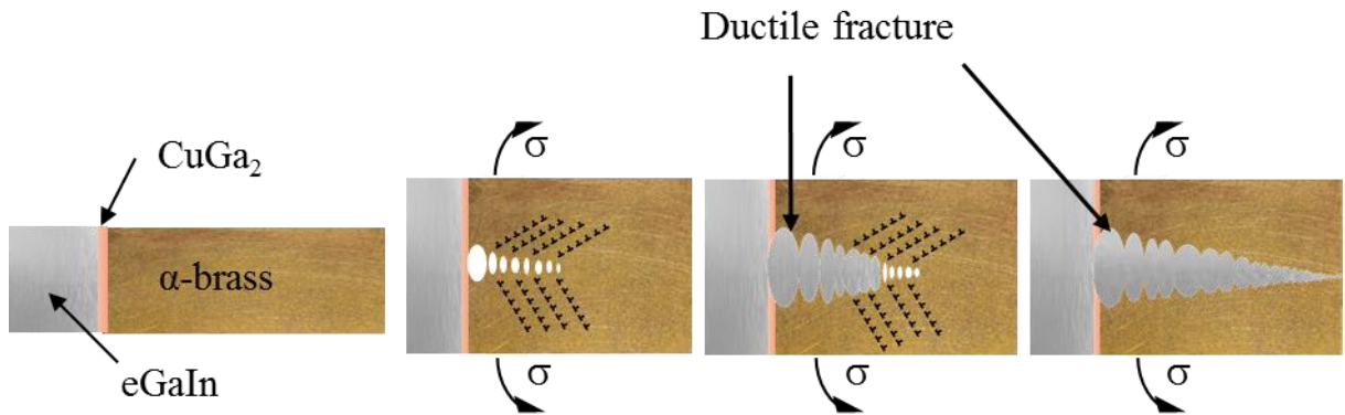
Figure III-74 Schema of the situation of non-LME of the alpha brass in contact with the liquid EGaIn.
