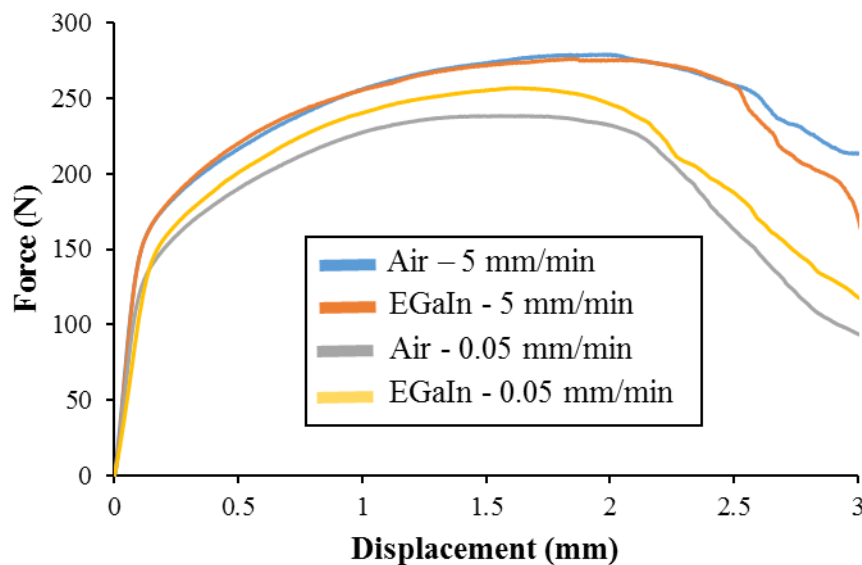
Figure III–64 Force-displacement curves of 3-point bending tests at 5 and 0.05 mm/min for annealed Cu-20%Zn samples tested in air and in contact with the EGaIn.
