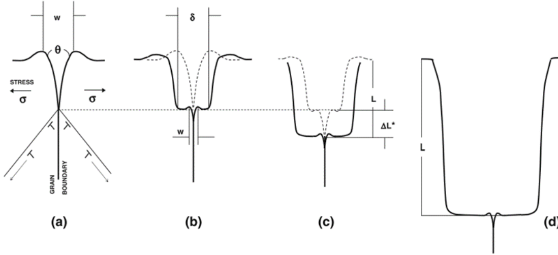
Figure I-10 GALOP mechanism of grain boundary LME [49].
