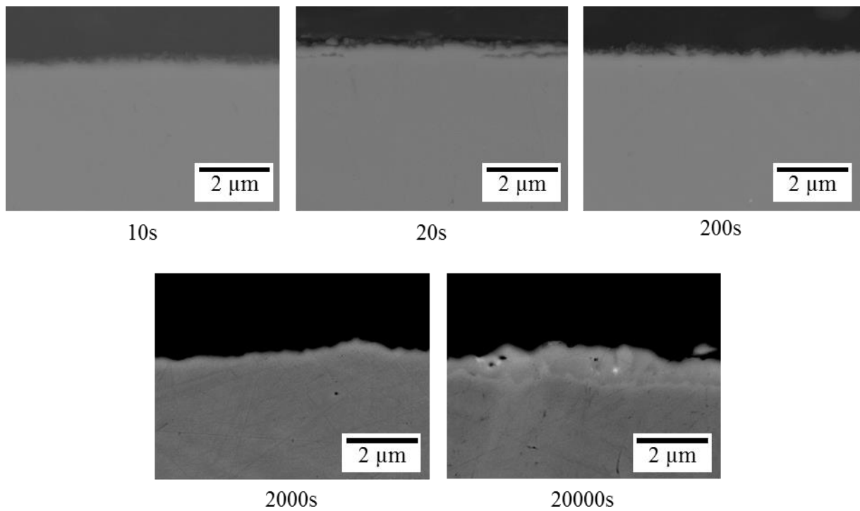
Figure II-18 Transversal cut of the intermetallic formation at different times.
