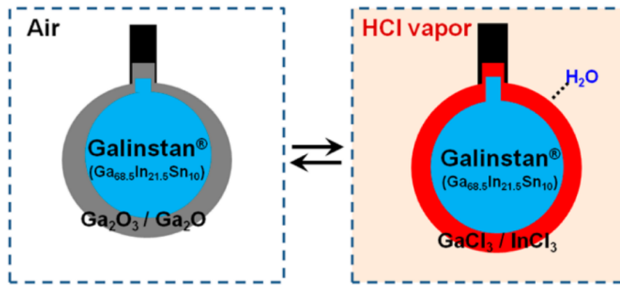
Figure I–19 Schematic diagram of the chemical reaction with HCl vapour. The phase of oxides ( \text{Ga}_2\text{O}_3/\text{Ga}_2\text{O} ), chlorides ( \text{GaCl}_3/\text{InCl}_3 ), and water is solid, aqueous, and liquid, respectively [90].
