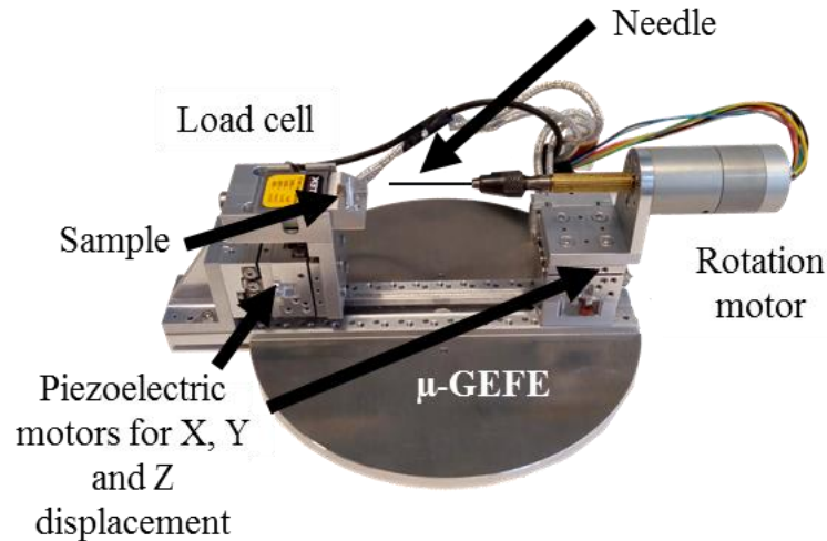
Figure IV–6 In-situ machine used for micromechanical testing [15].
