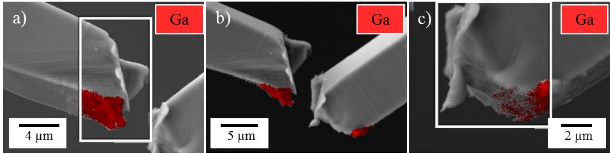
Figure IV–34 EDS analysis on the fracture of the clamped beam bending test sample.
