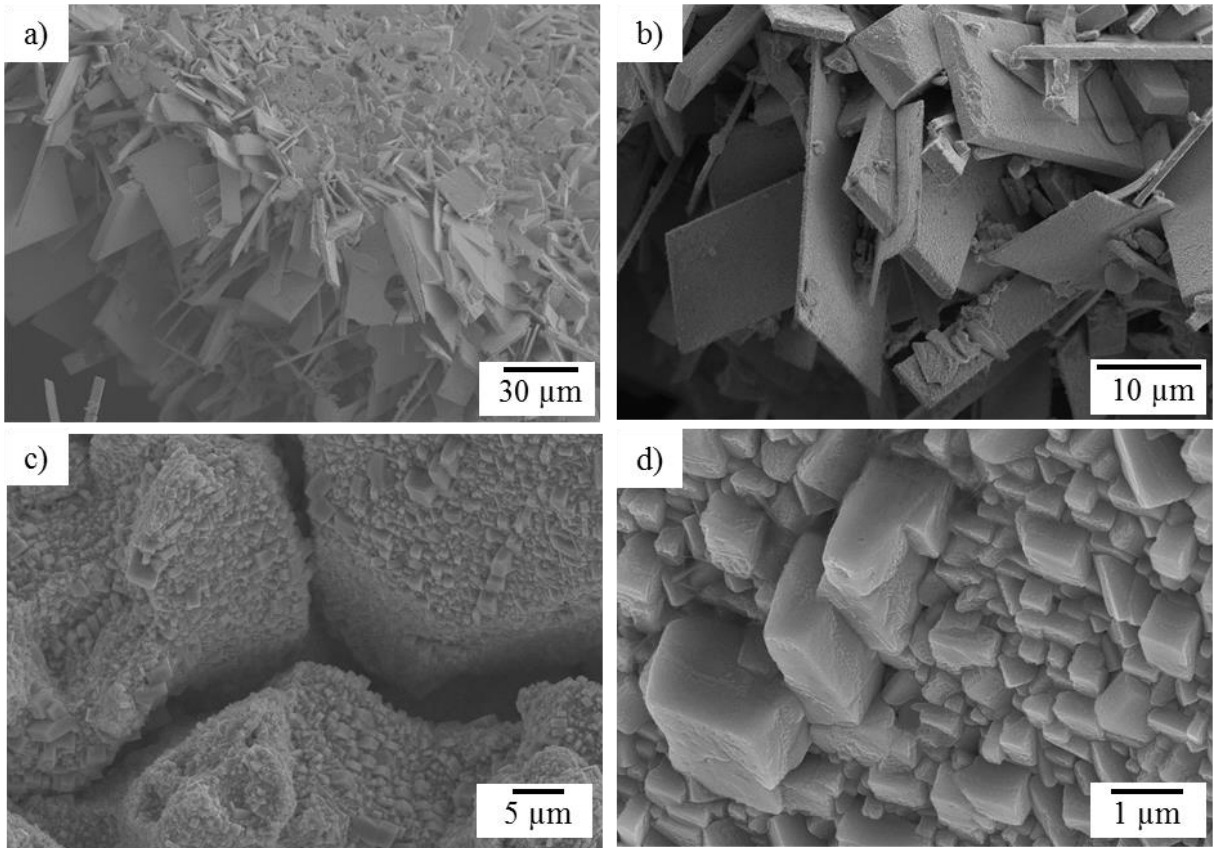
Figure II–15 Intermetallic formed between EGaln and Cu-30%Zn samples. b) Is a zoom of a), and d) is a zoom of c).
