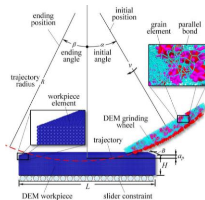
Figure 34. Configuration of the grinding simulation [96]
