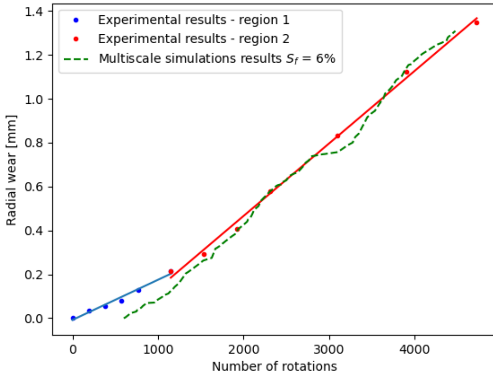
Figure 79. Experimentally measured and simulated radial wear for a shape factor value of S_f=6\% .
