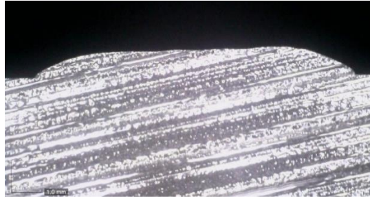
Figure 50. Loss of geometry as measured on the graphite workpiece at the center of the wheel ( V'_w=900.12 \text{ mm}^3/\text{mm} )
