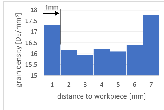
Figure 66. Surface grain density in \mu\text{SM} . Effect of element pile-up from numerical sintering.
