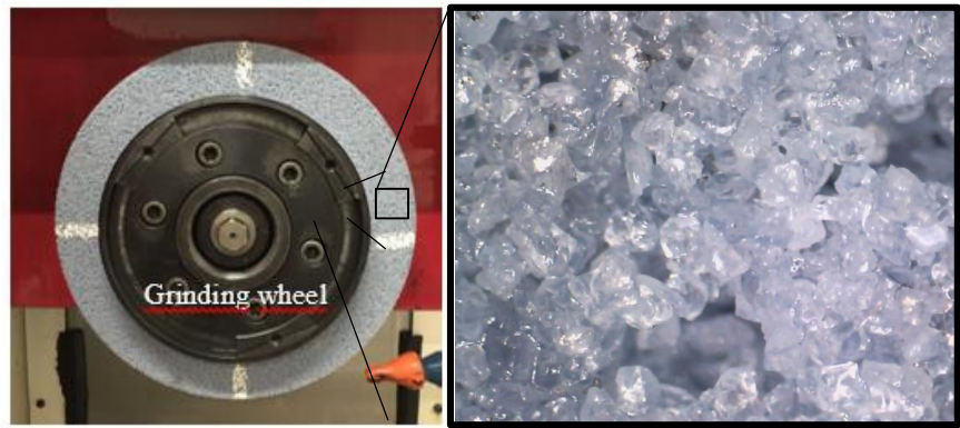
Figure 36. Vitrified alumina grinding wheel 100% monocrystalline
