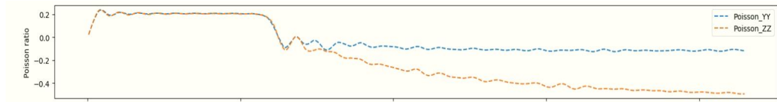
Figure 64. Results of the initial tensile test showing the calibration process for obtaining a stable value of macro Poisson ratio ( \nu_s ).
