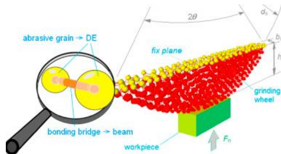
Figure 35. Schematic representation of the grinding wheel model [143]
