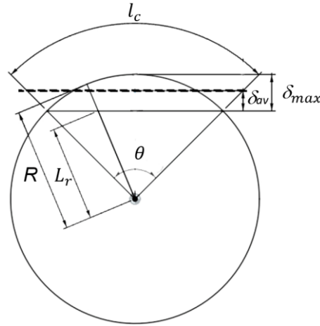
Figure 60. Schematic diagram for calculation of \delta_{av} .
