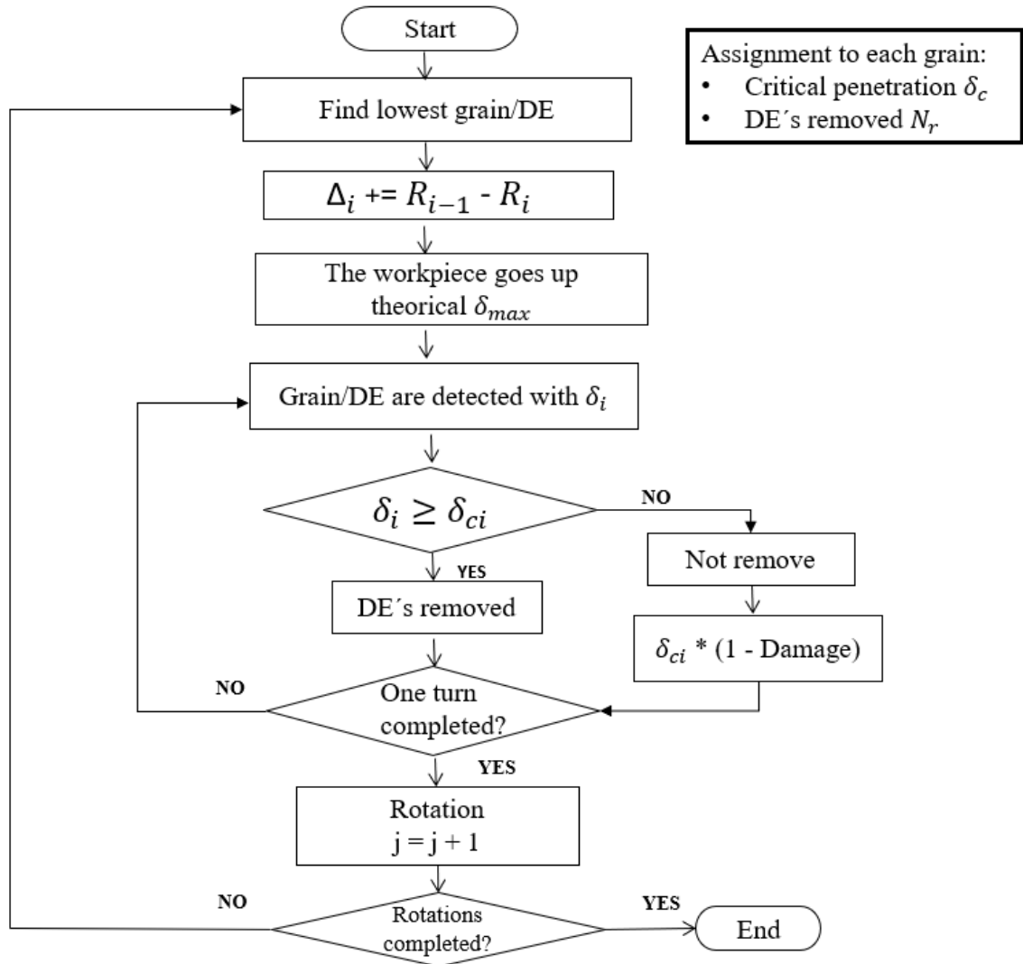
Figure 71. Flow chart showing the algorithm of the RμSM in Hypothesis 2.
