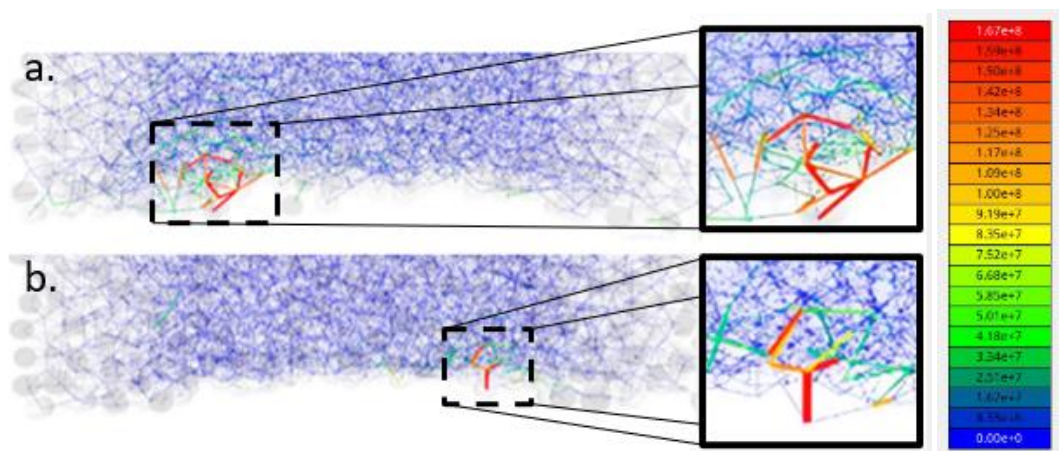
Figure 77. Beam Stress Analysis in the Cut Plane B-B' of \mu SM at different workpiece positions. (a) Workpiece position 0.36 mm. (b) Workpiece position 1.05 mm.
