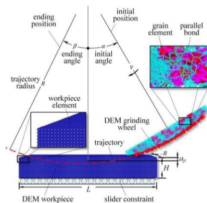
Figure 34. Configuration of the grinding simulation [96]
