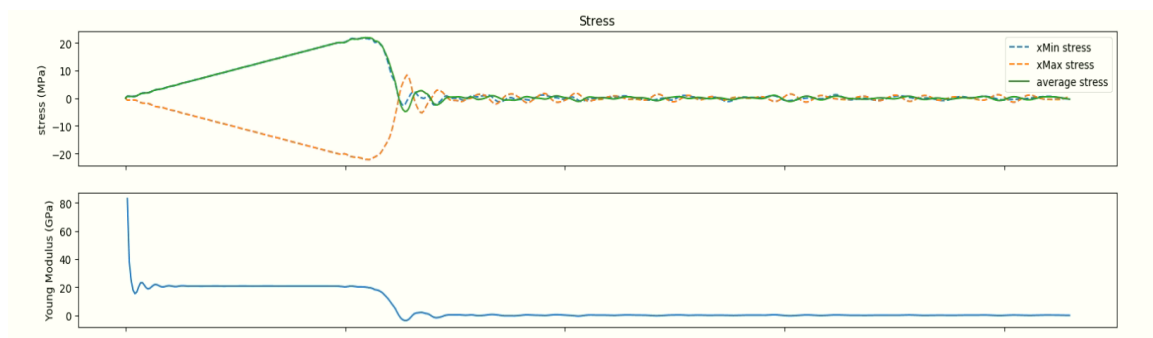
Figure 65. Results of the second tensile test showing the calibration process for obtaining a stable value of macro Young modulus ( E_s ) and reach the macro failure stress ( \sigma_f ).
