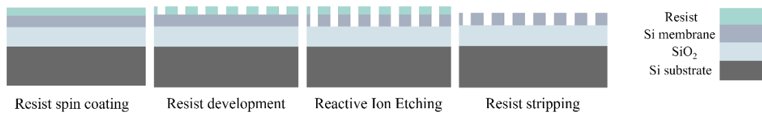
Figure 3-17: Phononic engineering patterning steps.
