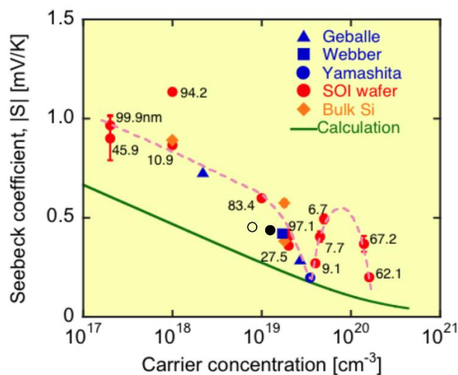
Figure 4-13: Seebeck coefficient of ultrathin SOI layers as a function of carrier concentration [93]. Our experimental data is represented by black circles, where filled circles denote p-type Si membranes and open circles represent n-type Si membranes.
