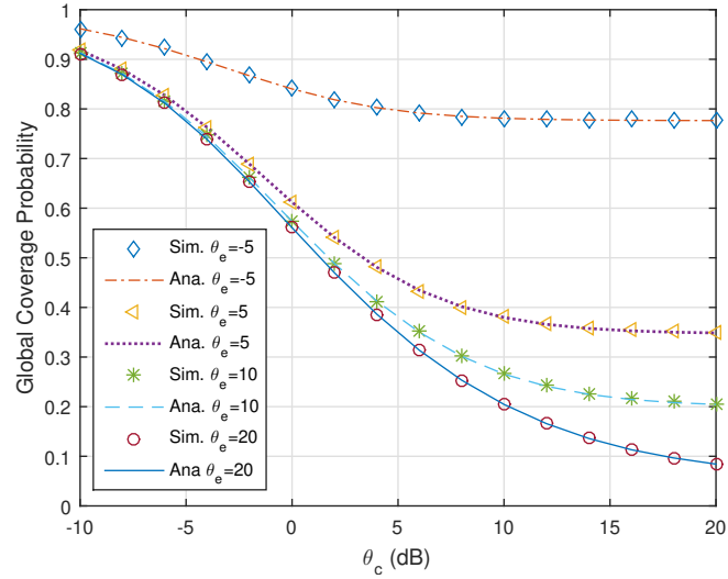
Figure 4.6 – Comparison of the coverage probability results versus \theta_c for various \theta_e .
