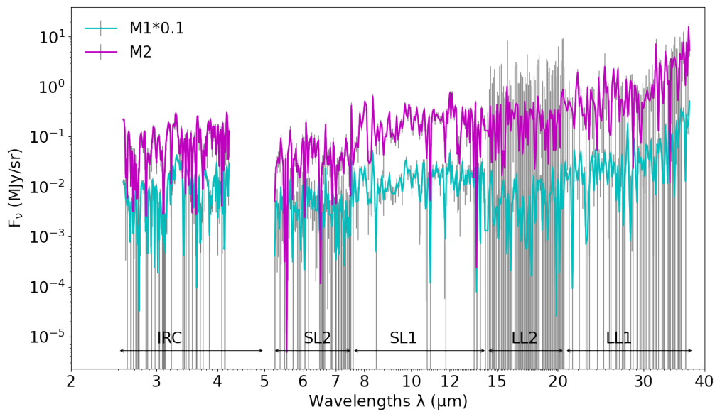
Figure 2.24 – Combined spectra of M 82 (slit M; northern wind cap).
