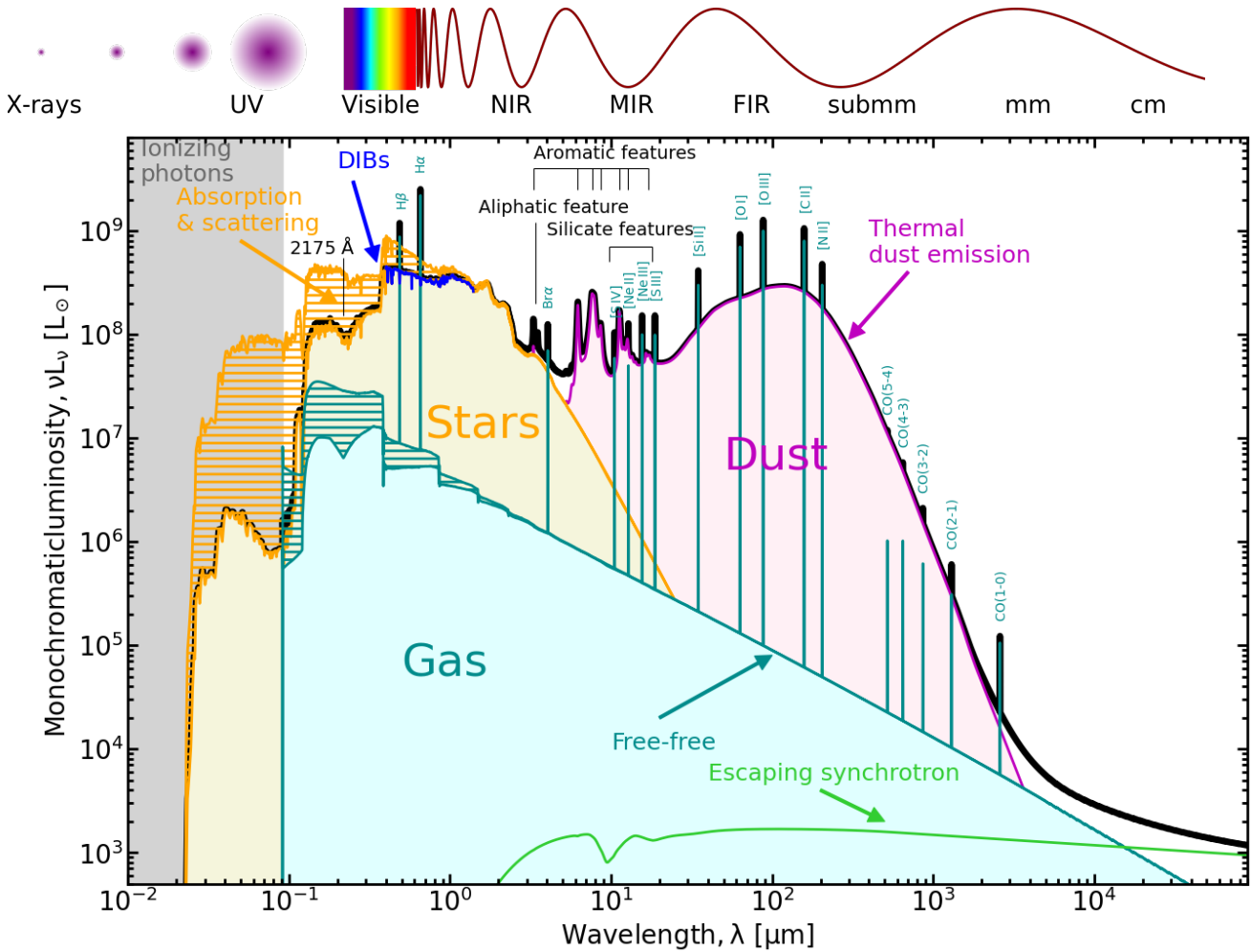
Figure 1.4 – Panchromatic spectral energy distribution (SED) of a synthetic typical late-type galaxy. On the top, we have schematically represented the different spectral regimes. On the main panel, the total simulated spectrum (black) is the sum of the escaping stellar emission (orange), the thermal dust continuum (magenta), the gas lines, the free-free continuum (dark cyan) and the synchrotron continuum (green). The hatched area shows the power absorbed by the dust. We have indicated the 2175 Å extinction bump, as well as the Diffuse Interstellar Bands (DIBs) ; blue; Herbig, 1995). We have also indicated the prominent emission and absorption features in the mid-infrared. The figure originates from Figure 1 of Galliano et al. (2018) and is modified with the author’s permission.
