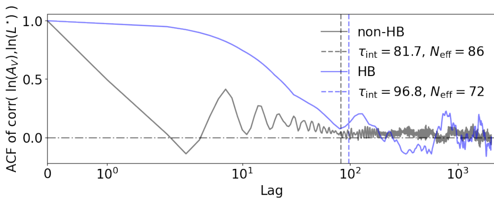
Figure D.9 – ACFs of the correlation coefficients with reduced sampling (after burn-in).
