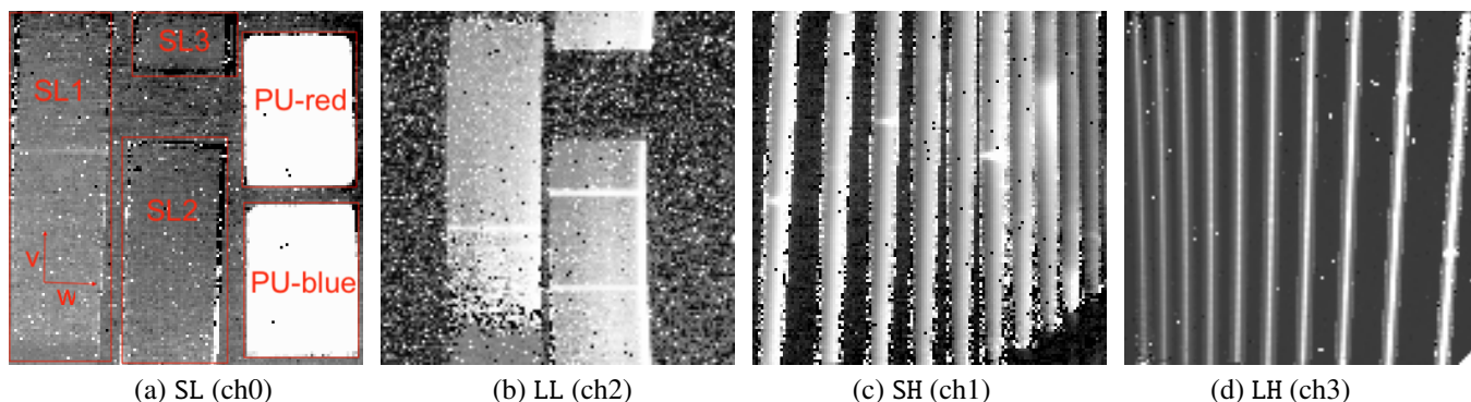
Figure 2.7 – IRS basic calibrated data (BCDs).
