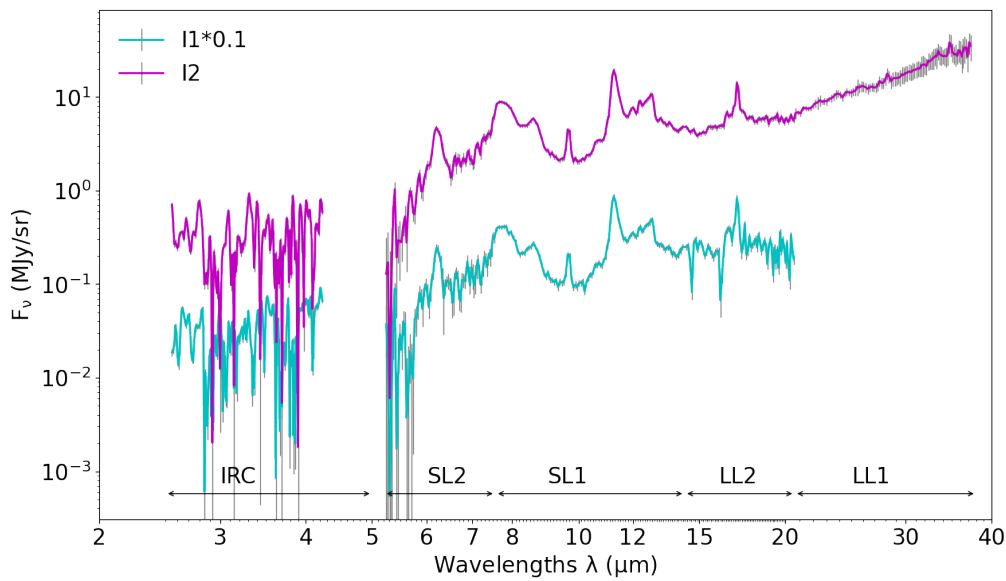
Figure D.17 – Combined spectra of M 82 (slit I; southern wind).
