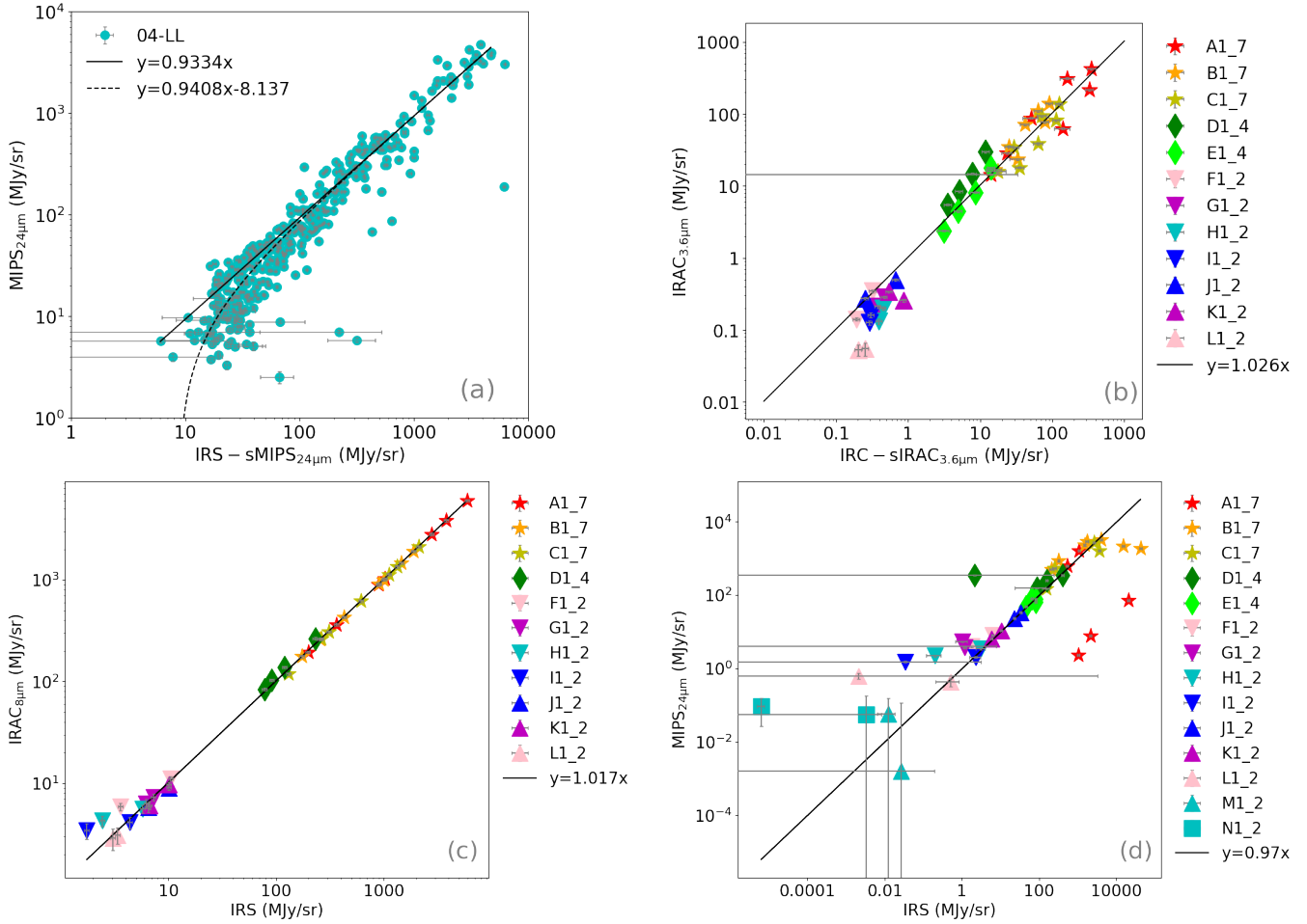
Figure 2.21 – Inter-calibration diagrams.
