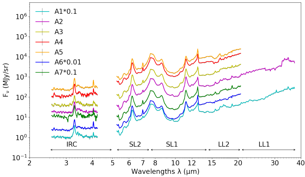
Figure 2.22 – Combined spectra of M 82 (slit A; central disk).
