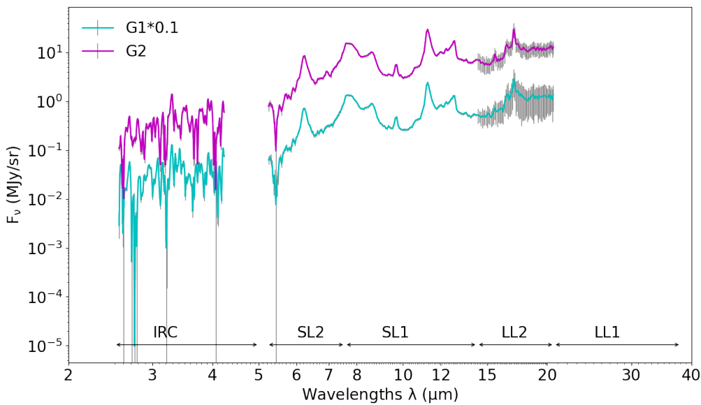
Figure 2.23 – Combined spectra of M 82 (slit G; southern wind).
