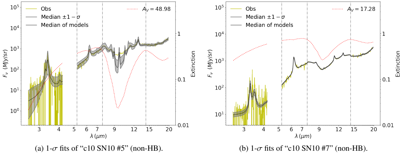
Figure D.2 – Median models fitted with the non-HB method.
