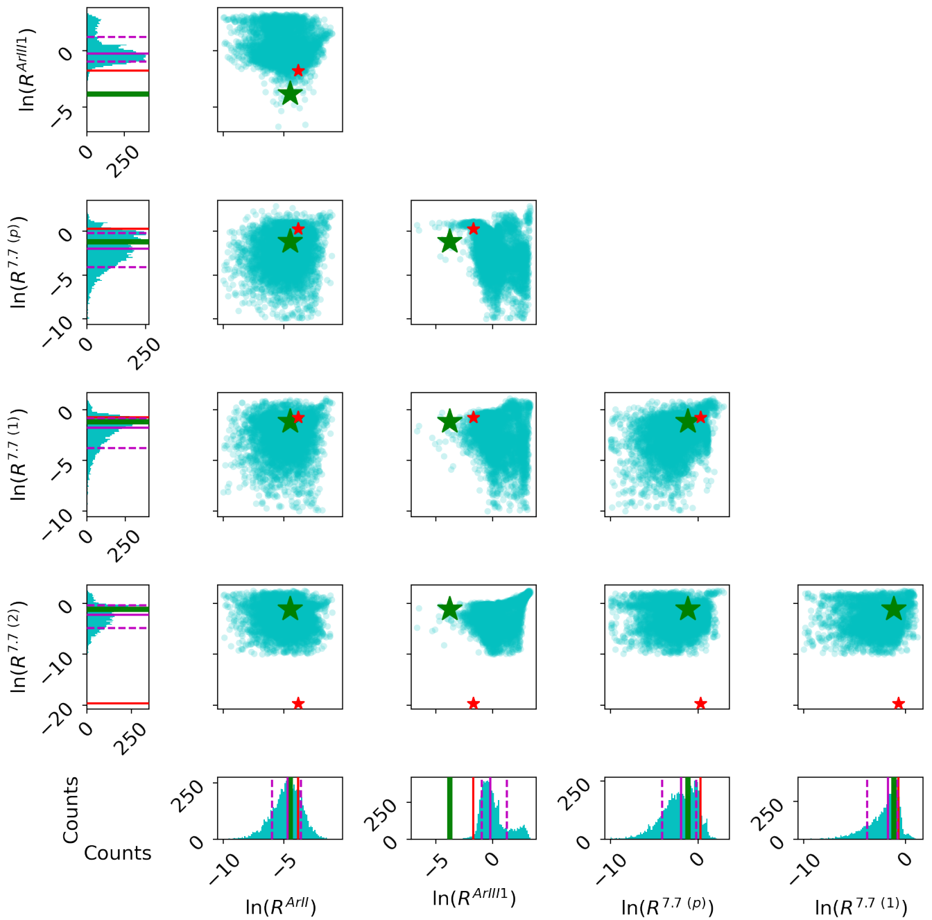
Figure D.6 – Multivariate distributions between emission line and band intensity ratios.
