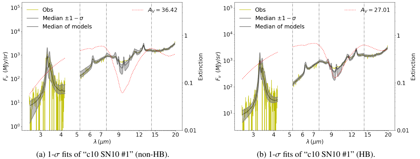
Figure 3.7 – Median models fitted with Bayesian methods. Panels (a) and (b) show the total models calculated at each wavelength in MCMC after burn-in within the 1-\sigma interval (gray shadowed; see text) distributed on both sides of the median values (black). The extinction curve (red dotted) is also overlaid.
