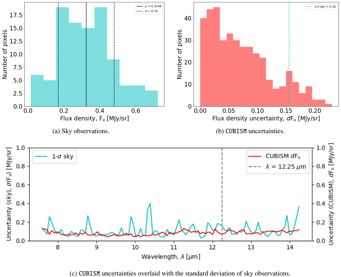
Figure 2.11 – Comparison of the uncertainties derived from the sky and from CUBISM.
