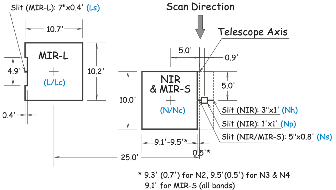
Figure 2.2 – Relative field-of-view location and size of the three channels of AKARI/IRC.
