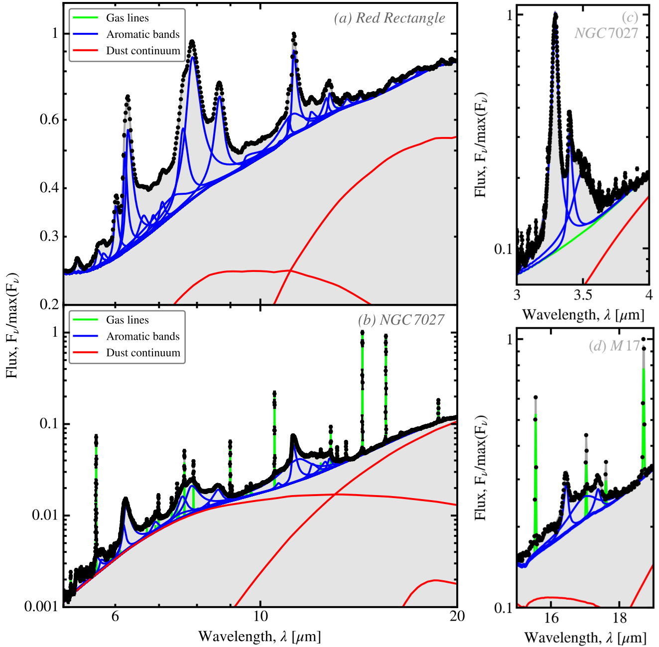
Figure 3.2 – Empirical calibration of UIB profiles.
