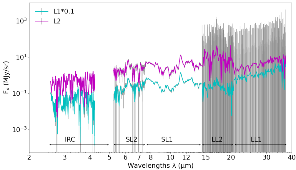
Figure D.20 – Combined spectra of M 82 (slit L; northern outer wind).
