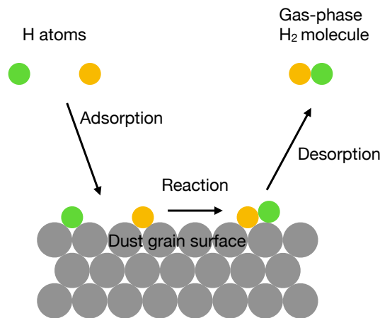
Figure 1.2 – Mechanism of \text{H}_2 formation on grain surfaces.
