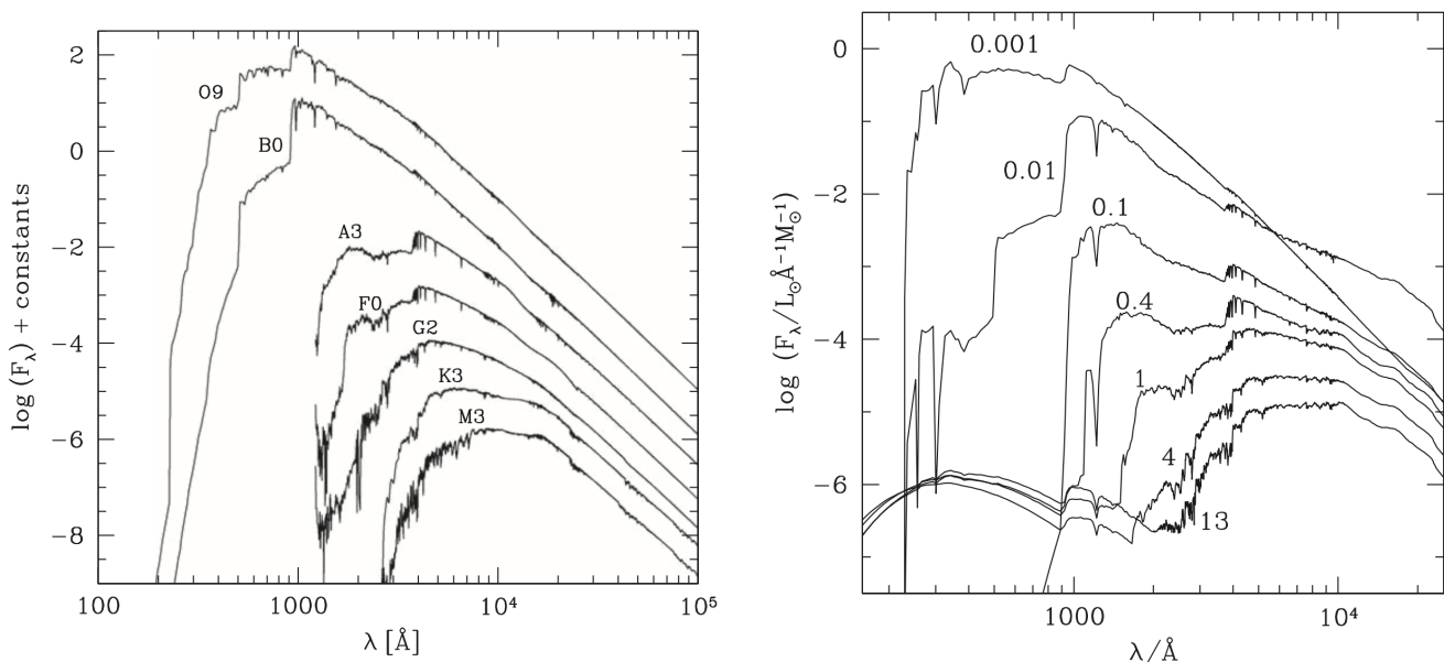
Figure 1.9 – Synthetic stellar spectra.
