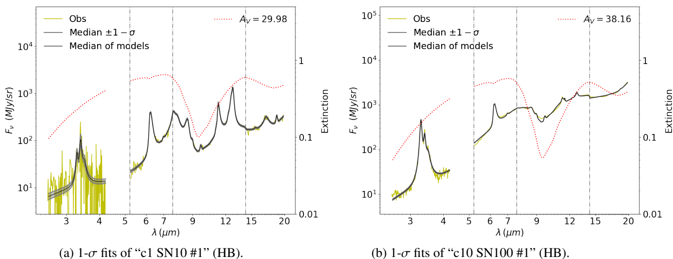
Figure D.1 – Median models fitted with the HB method.
