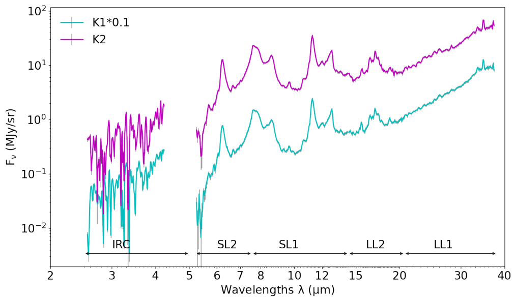
Figure D.19 – Combined spectra of M 82 (slit K; northern wind).
