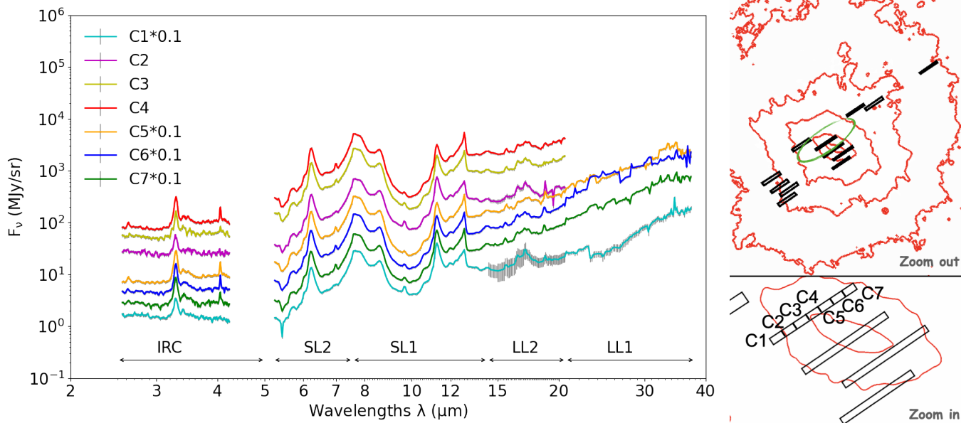
Figure D.12 – Combined spectra of M 82 (slit C; central disk).
