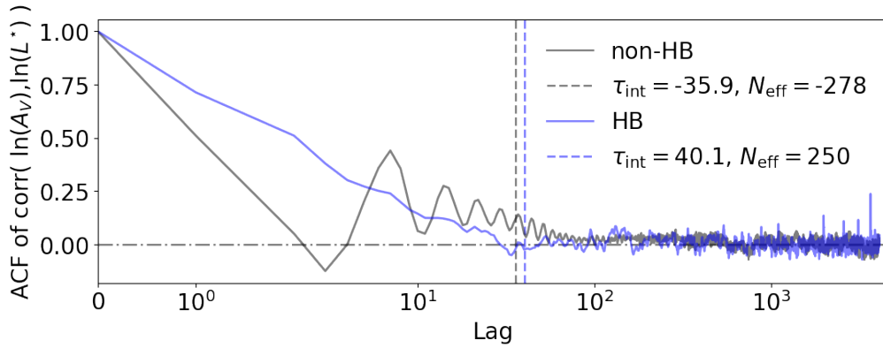
Figure D.8 – ACFs of the correlation coefficients of two parameter (without burn-in).
