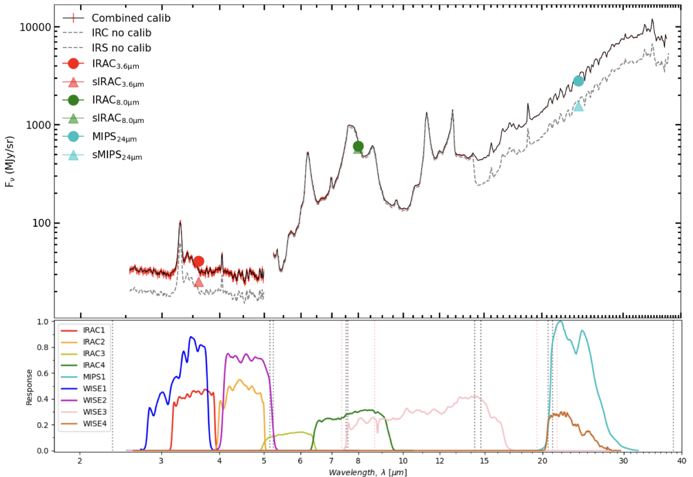
Figure 2.16 – Example of inter-calibration.
