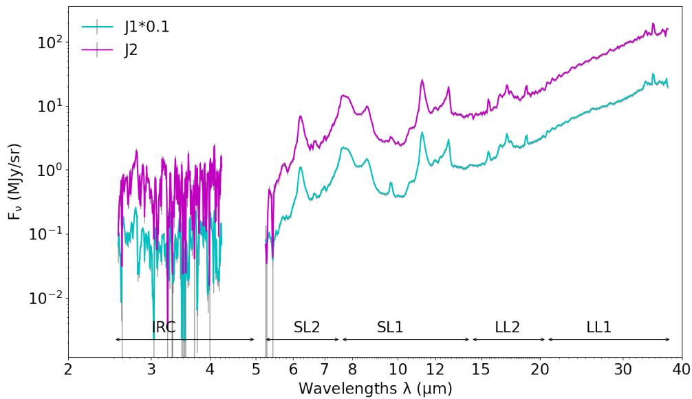
Figure D.18 – Combined spectra of M 82 (slit J; northern wind).
