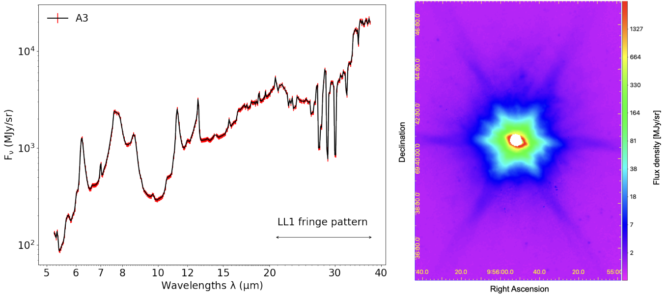
Figure 2.20 – Saturation effect in Spitzer observations.
