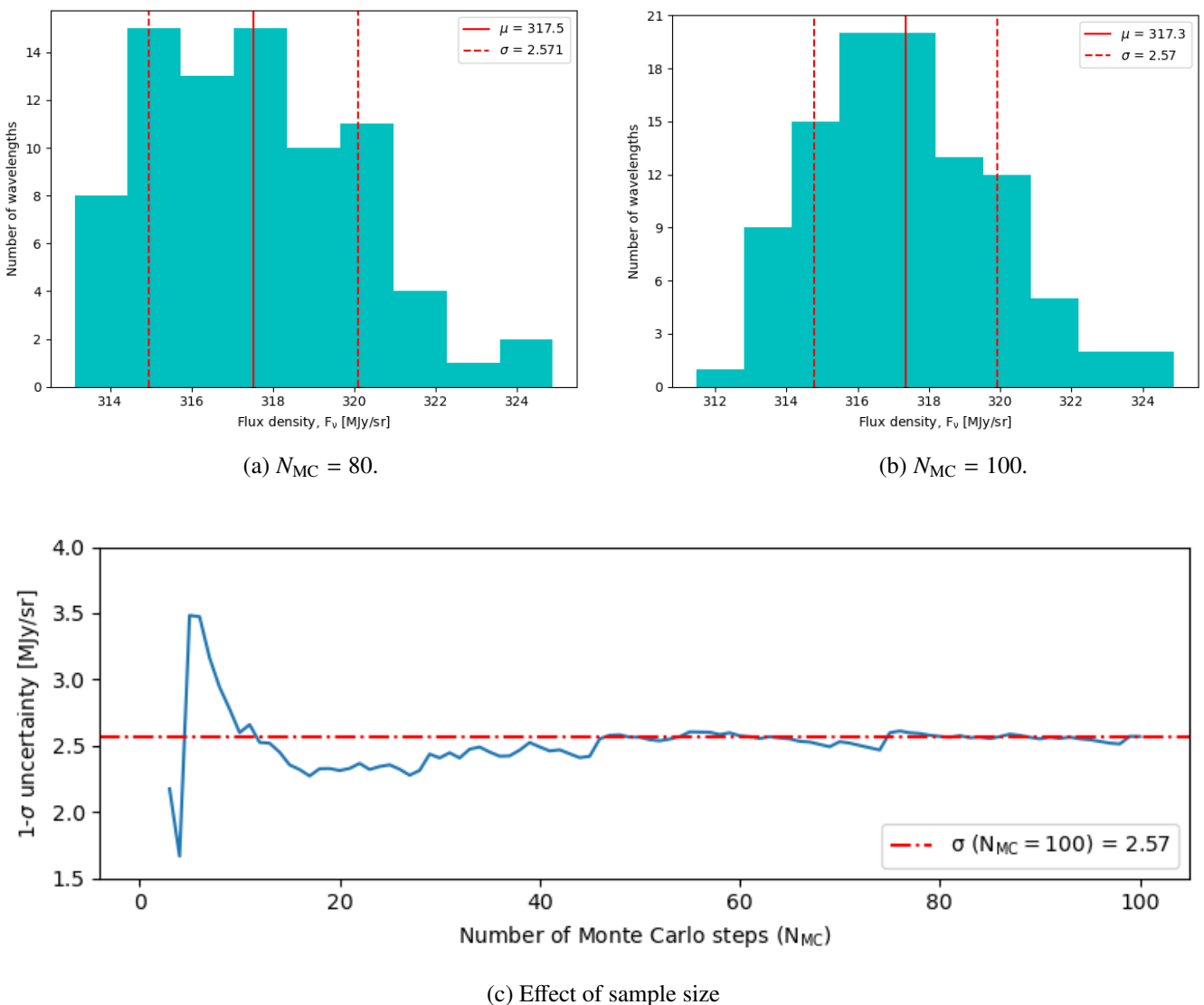
Figure 2.3 – Demonstration of the bootstrapping method to propagate the uncertainties. Panels (a) & (b) show the flux density distribution of a Spitzer /IRS pixel within the M 82 spectral map at \lambda = 7.29 \mu\text{m} , with the number of Monte Carlo steps N_{MC} = 80 and N_{MC} = 100 , respectively. Panel (c) shows the standard deviation of the above distribution as a function of N_{MC} , where the 1-\sigma uncertainty for N_{MC} = 100 is marked with a red dash-dotted line.
