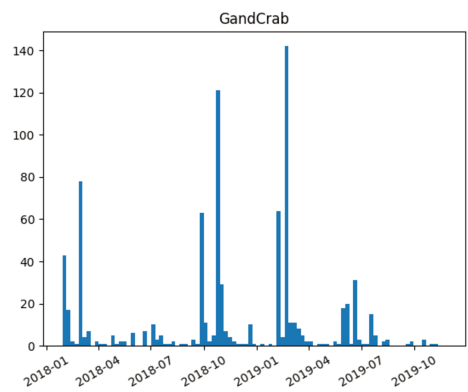
d) GandCrab
