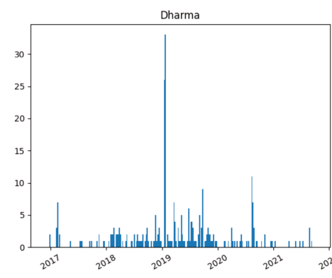
d) Dharma
