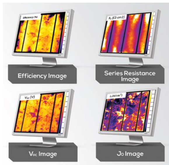
Figure 3-5: Example of results output from a WCT-120 manufactured by Sinton instruments using they curve theory
