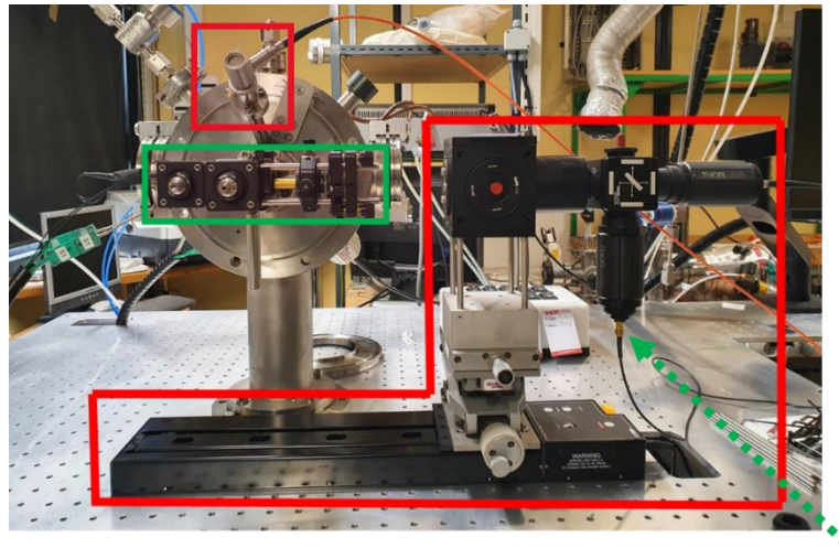
Figure 2-4: Both previous and new in-situ optics systems mounted onto the PECVD reactor.
