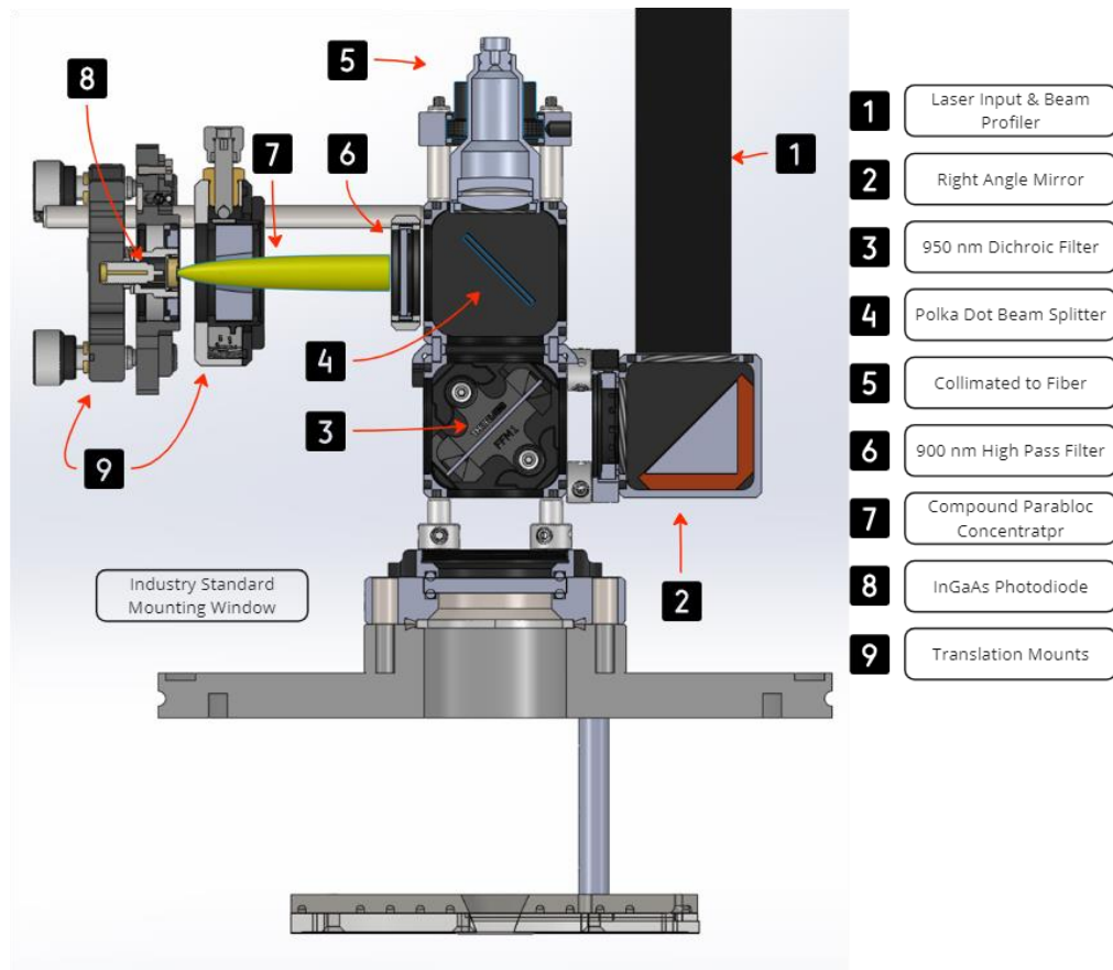
Figure 2-21: Schematic layout of the new optical design using non-imaging optics for \tau_{\text{eff}} and PL.
