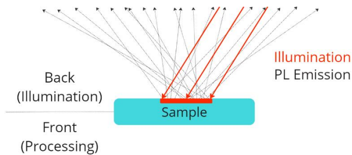
Figure 2-1: Basic working principle for in-situ \tau_{\text{eff}} and PL measurement techniques in [34].
