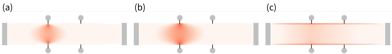
Figure 1.21: Current dissipation in a Hall bar geometry ( n_L = 111, n_W = 21 ) in the non-local configuration. The calculation of the current dissipation is calculated for three different cases: (a) G_{\text{edge}} = G_{\text{bulk}}/100 , (b) G_{\text{edge}} = G_{\text{bulk}} , and (c) G_{\text{edge}} = 100G_{\text{bulk}} .
