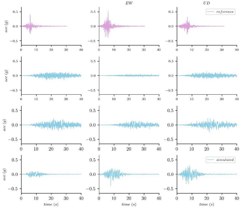
Figure 4.7. Comparison of reference and simulated time histories for one of the replicated scenarios ( M_w = 6.50, R_{hypocentral} = 27.96\text{km}, Z = 9.20\text{km} ).
