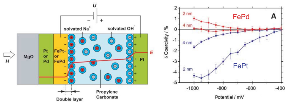
Figure 1.6: A schematic of the electrolytic gating of FePt or FePd film showing the formation of an electric double layer under an applied potential U (on the left). Changes in the coercivity of FePd (red) and FePt (blue) as a function of applied potential for different thicknesses of the films (on the right). Adapted from [27].
