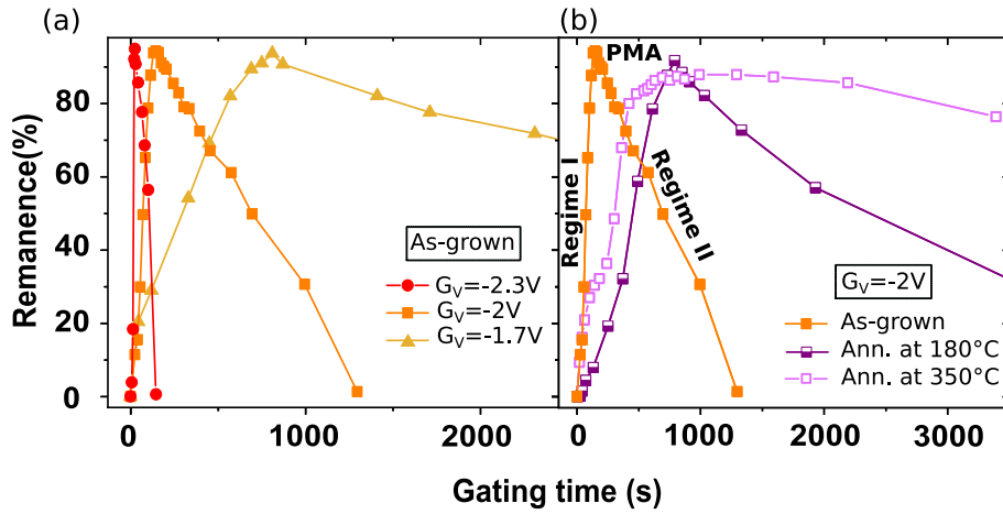
Figure 4.3: Remanence as a function of gating time in (a) as-grown samples under G_V = -2.3\text{V} (circles), G_V = -2\text{V} (squares), and G_V = -1.7\text{V} (triangles). (b) Samples annealed at 180\text{ }^\circ\text{C} (half open squares) and 350\text{ }^\circ\text{C} (open squares) under G_V = -2\text{V} .
