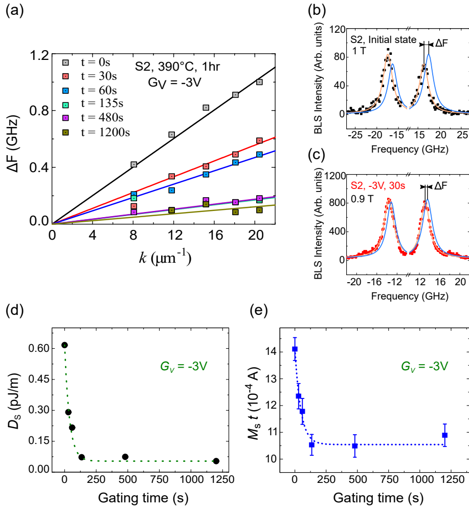
Figure 5.5: (a) Frequency asymmetry ( \Delta F ) as a function of the wave vector ( k ) for S2 samples exposed to different durations of a gate voltage of -3V. BLS spectra at k=20 \mu\text{m}^{-1} of S2 (b) in the initial state, and (c) after applying a gate voltage of -3V for 30s. (d) Surface DMI constant ( D_s ) and (e) M_s \cdot t as a function of the gating time under a gate voltage G_V = -3\text{V} for sample S2. The dotted lines are a guide to the eye.
