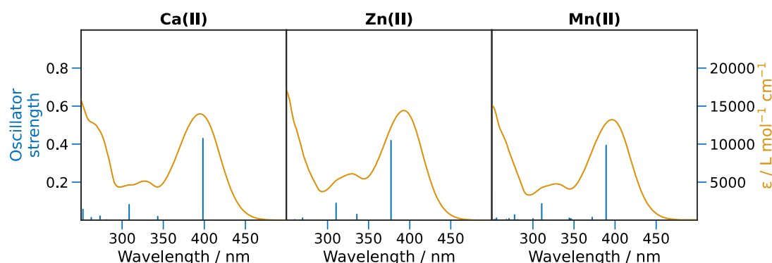
Figure I. 50: Comparison between the experimental absorption spectrum of the 2'3HF-M (Ca(II), Zn(II) or Mn(II)) complex and the computed electronic transitions of the optimized 2'H3H(t) complexes
