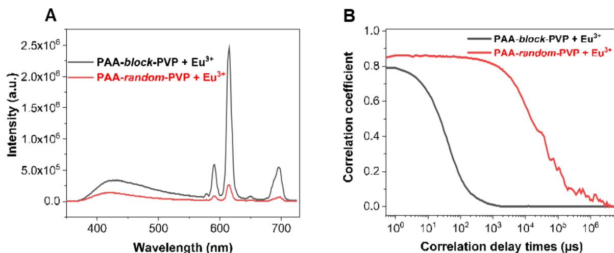
Figure 72. Commercial random \text{PAA}_{416}\text{-}r\text{-PVP}_{270} copolymer vs. block \text{PAA}_{32}\text{-}b\text{-PVP}_{59} copolymer: Comparison of emission spectra (A) ( \lambda_{\text{ex}}=325\text{ nm} ) and (B) DLS correlograms of \text{Eu}^{3+} / \text{PAA}_{32}\text{-}b\text{-PVP}_{59} HPICs and \text{Eu}^{3+} / \text{PAA}_{416}\text{-}r\text{-PVP}_{270} mixture ([polymer]=0.2% wt) for R=1
