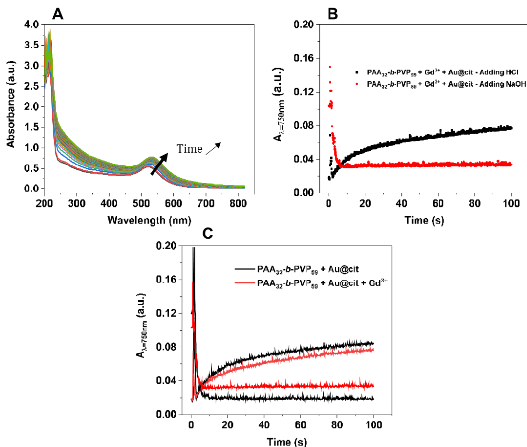
Figure 190. UV-vis spectra (100 scans) of \text{PAA}_{32}\text{-}b\text{-PVP}_{59} (0.014%wt) + \text{Gd}^{3+} ions ( [\text{Gd}] = 0.2\text{mM} ) + \text{Au@citrate} NPs ( [\text{Au}] = 144\mu\text{M} ) solution under pH variation after adding 8 \mu\text{L} of HCl solution (1M) (A) Time evolution of the absorbance measured at \lambda = 750 nm for both assembly and disassembly mechanisms (B) Comparison with the system \text{PAA}_{32}\text{-}b\text{-PVP}_{59} + \text{Au@citrate} NPs (C)
