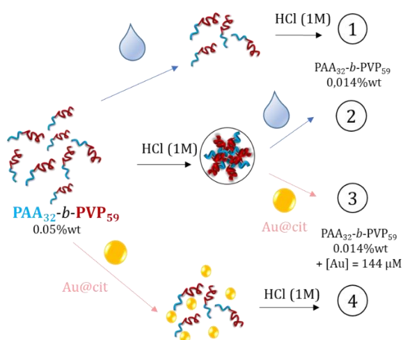
Scheme 11. Sample preparation protocols to obtain nanoassemblies composed of PAA 32 -b-PVP 59 (0.014%wt) with or without Au@citrate ([Au]=144 \mu M): (1) Dilution then lowering pH onto PAA 32 -b-PVP 59 solution; (2) Lowering pH then dilution onto PAA 32 -b-PVP 59 solution; (3) Lowering pH onto PAA 32 -b-PVP 59 then introducing Au@citrate; (4) Introducing Au@citrate into PAA 32 -b-PVP 59 solution at high pH value then lowering pH.
