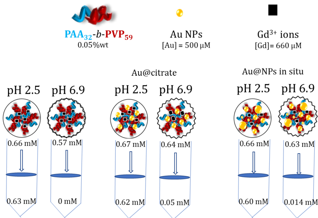
Scheme 14. ICP-MS results introduced in the schematization of the filtration processes for the 6 tested systems comprising PAA 32 - b -PVP 59 (0.05%wt) and Gd 3+ ions ([Gd] = 0.7 mM) without or with gold nanoparticles which are either performed Au@citrate NPs or AuNPs formed in situ ([Au]=500 μM) at varying pH, either pH=2.5 or pH=6.9.
