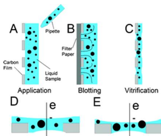
Figure 25. Schematic of cryo-TEM sample preparation: (A) Side view of a liquid containing particles (●) being applied to a perforated carbon TEM grid; (B) removal of excess solution by blotting grid with filter paper; (C) formation of vitrified thin film after rapidly plunging into a suitable cryogen; (D) expanded side view of vitrified grid showing the path of the electron beam when viewed in a TEM column; (E) size segregation may occur during sample preparation, with larger particles at the edges of the holes and smaller particles at the center of the thin film. Large particles may also protrude from the film. (reproduced with permission from 171 )
