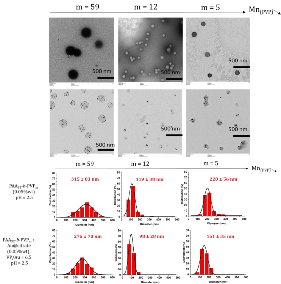
Figure 167. TEM pictures and associated size distribution diagrams of samples containing PAA 32 -b-PVP m (0.05%wt) without (first line) or with (second line) Au@citrate NPs at a fixed VP/Au=6.5, with m corresponding to the DP of PVP, all samples are at pH=2.5 after adding HCl (1M).
