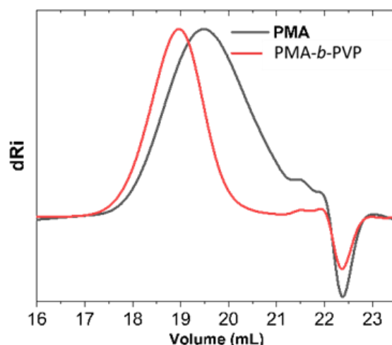
Figure 31. Size exclusion chromatograms (RI traces) in DMF/LiBr 10mM of PMA 32 - b -PVP 59 (red line) and PMA 32 (black line)
