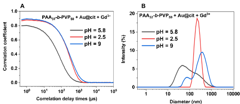
Figure 185. (A) Correlation functions using the NNLS method, (B) Distribution average size in intensity for the sample containing PAA 32 -b-PVP 59 (0.05%wt) + Gd 3+ ions ([Gd] = 0.7mM) + Au@citrate NPs ([Au]=500μM) at varying pH values after adding HCl solution (1M) and then NaOH solution (1M).
