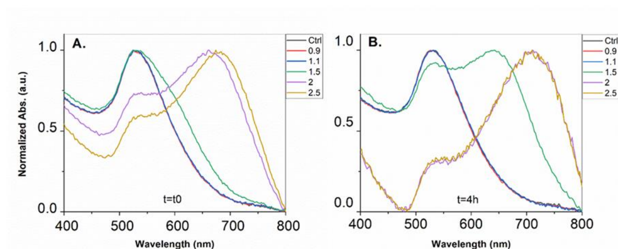
Figure 104. UV-visible spectra of AuNP@BSPP in the presence of the filtrate resulted from the purification of HPICs of different ratios R (positive charges over negative charges) registered at t_0=15\text{min} (A) and at t=4\text{h} (B).
