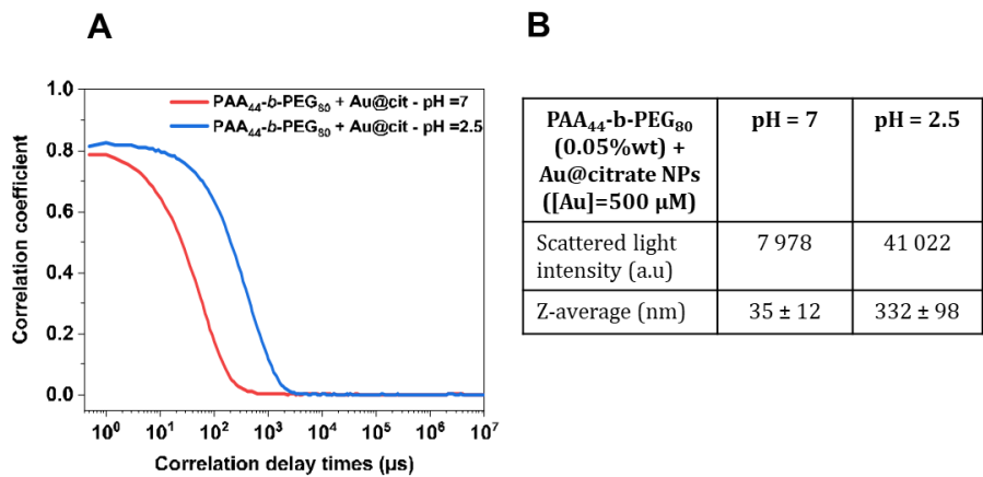
Figure 151. Correlation functions using the NNLS method ( A ) and Scattered light intensity and Z-average size ( B ) of the samples containing PAA 44 -b-PEG 80 (0.05%wt) + Au@citrate ([Au] = 500μM) at two pH values: pH=7 and pH=2.5.
