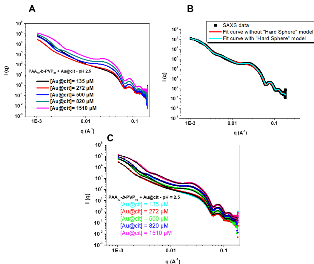
Figure 165. (A) SAXS curves for the samples containing PAA 32 -b-PVP 59 (0.05%wt) and varying Au@citrate NPs concentration: 135, 272, 500, 820, 1510 μM at pH=2.5 (B) SAXS data (black squares) and fit curves applied according to two models considering hard sphere model (cyan curve) or not (red curve) (C) SAXS curves for the samples containing PAA 32 -b-PVP 59 (0.05%wt) and varying Au@citrate NPs concentration: 135, 272, 500, 820, 1510 μM at pH=2.5 with associated fitting curves applied according to the best adapted model.
