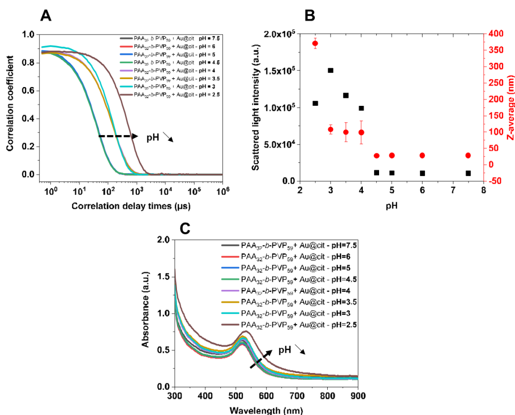
Figure 143. (A) Correlation functions using NNLS method, (B) typical evolutions of the scattered light intensity (black squares) and Z-average diameter (red dots) and (C) UV-vis spectra of the samples containing PAA 32 - b -PVP 59 (0.05%wt) and Au@citrate ([Au]=500μM), adjusted at varying pH values with HCl solution (1M). Arrows are indicating the progressive decrease of the pH value.
