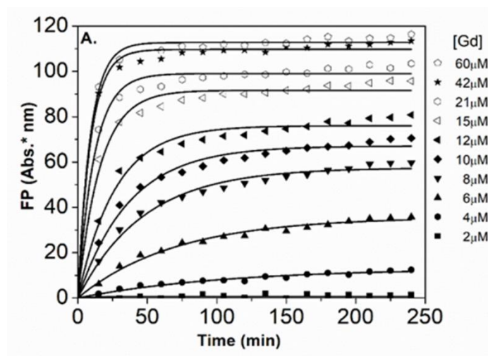
Figure 87. Time dependence of the FP of AuNP@BSPP plotted for increasing concentrations in \text{Gd}^{3+} together with the best fit to eq. 1
