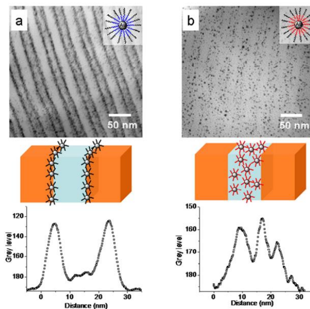
Figure 15. (a) TEM image together with the image analysis of the composites consisting of PS- b P2VP block copolymer (199 kg/mol, fp2vp ~ 0.48) and 20 wt.% of GNPs (PS23- b -PNBA9S-Au). (b) The GNPs were exposed to UV (365 nm) light before mixing with the PS- b -P2VP block copolymer (reproduced with permission from 149 )
