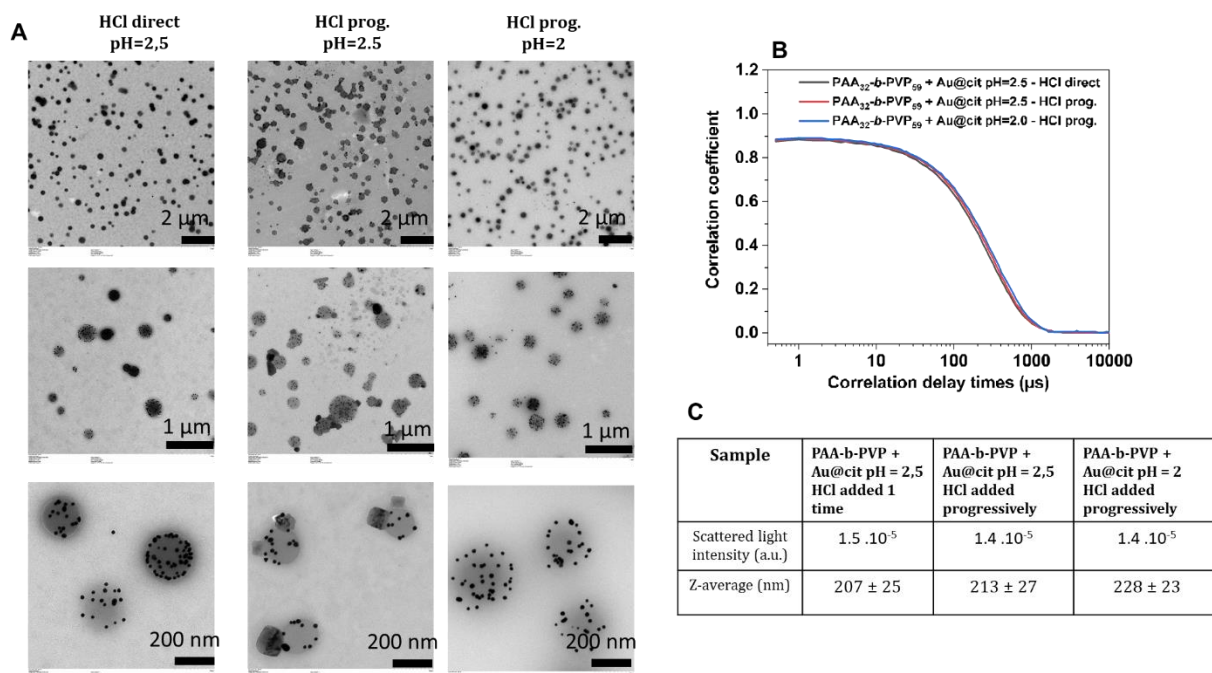
Figure 145. (A) TEM pictures of the samples containing PAA 32 -b-PVP 59 (0.05%wt) and Au@citrate ([Au]=500 \mu M) adjusted at pH=2.5 by adding HCl solution (1M) through 2 ways: only one direct add ("HCl direct") or several add ("HCl prog.") and this second way is used to decrease until pH=2 (B) Corresponding correlation functions using NNLS method and (C) Table showing the data from DLS measurements: Scattered light intensity and Z-average size.
