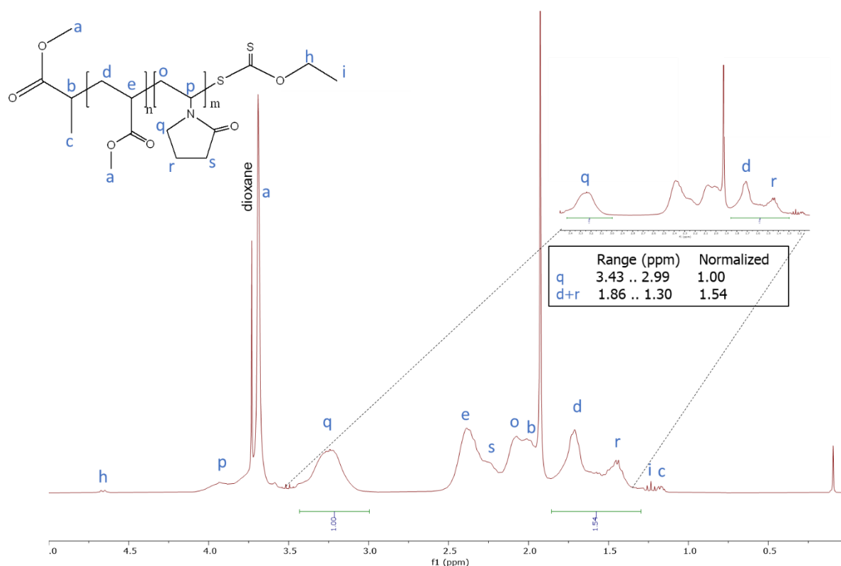
Figure 30. ^1\text{H} NMR Spectra ( \text{CDCl}_3 ) of the synthesized Poly(Methyl Acrylate)-block-Poly(vinylpyrrolidone) copolymer (PMA 32 - b -PVP 59 ). Degree of polymerization of N-VP (DP = 59) can be evaluated by directly comparing the ratio of the integrals of signals of PVP (q signal) to the one of PVP plus PMA (r and d signals) assuming a degree of polymerization of PMA block of 32, using the following equation: \text{DP}_{\text{PVP}} = (\text{DP}_{\text{PMA}} * q) / (r + d - q)
