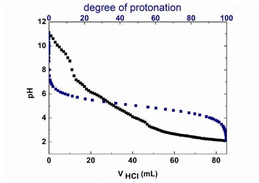
Figure 57. Titration curve of PAA 32 - b -PVP 59 copolymer ( 0.1% wt ) on which it was added a 0.1M HCl solution. pH values were recorded at each add of HCl (black curve) and the corresponding protonation degree curve (blue curve)
