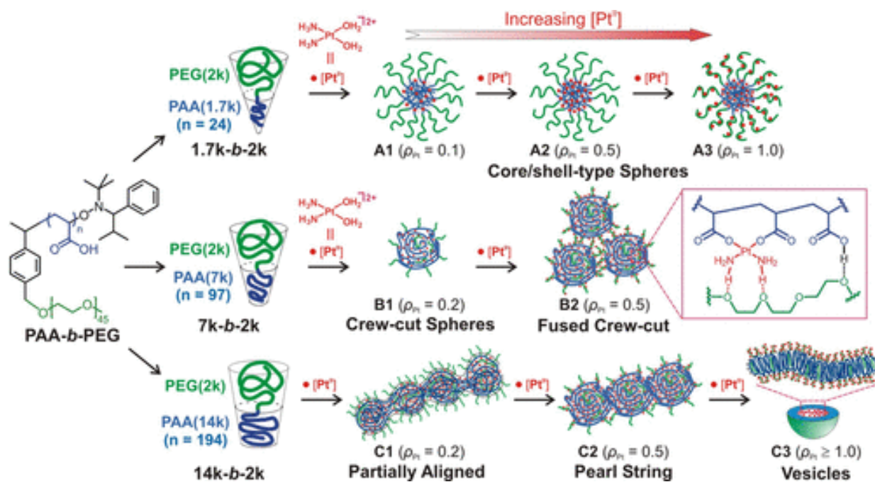
Figure 6. Schematic Illustration Showing the Morphology Transition of Pt II -Incorporated Nanostructures, depending on the Length of Chelating PAA Blocks and Pt II Feeding Ratio ( \rho_{Pt} ). (reproduced with permission from 71 )
