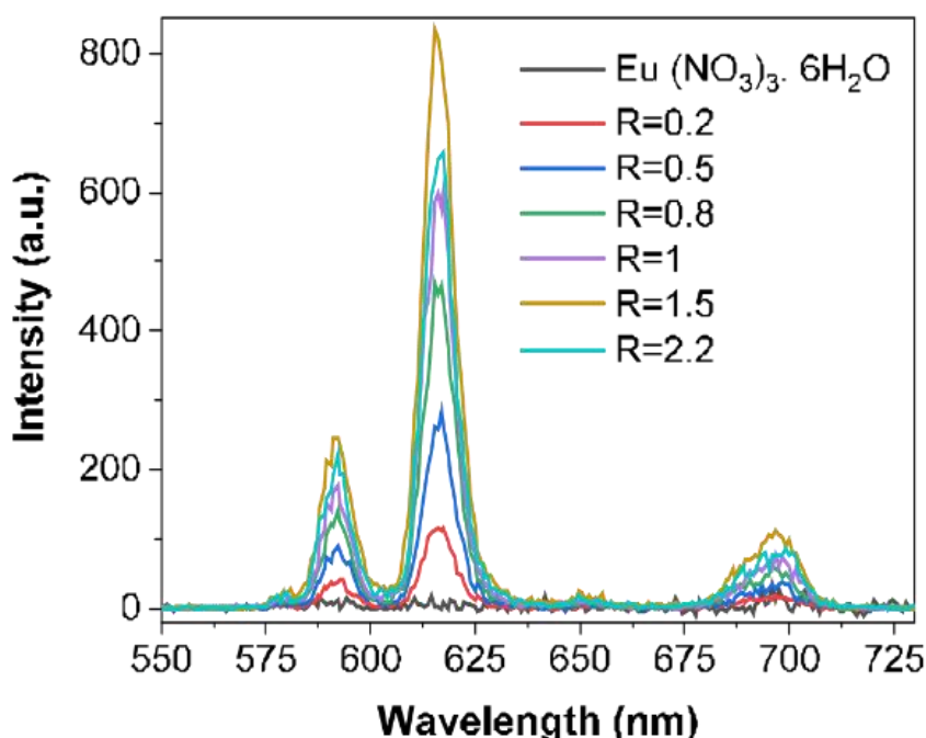
Figure 53. Emission spectra ( \lambda_{\text{ex}}=256 nm) of \text{Eu}^{3+}/\text{PAA}_{32}\text{-b-PVP}_{59} HPICs at different R ratios. [\text{PAA}_{32}\text{-b-PVP}_{59}] = 0.1\% wt in water solvent
