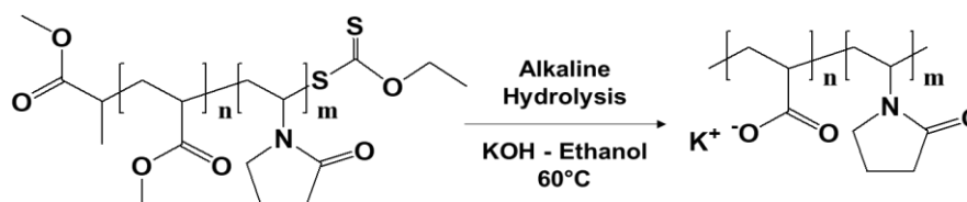
Scheme 7. Final hydrolysis step of the block copolymer synthesis protocol realized in ethanol with a concentration of potassium hydroxide (KOH) salt of 3.4 M and at 60°C to perform the ester cleavage and remove xanthate end-chain.
