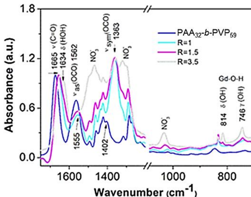
Figure 43. ATR-FTIR spectra of \text{PAA}_{32}\text{-}b\text{-PVP}_{59} and the respective \text{Gd}^{3+}/\text{PAA}_{32}\text{-}b\text{-PVP}_{59} HPICs for ratio R \geq 1
