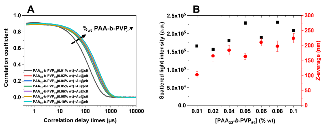
Figure 139. Correlation functions using the NNLS method ( A ) and typical evolutions of the scattered light intensity (black squares) and Z-average diameter (red dots) ( B ), measured by a mono-angle DLS instrument for samples containing varying PAA 32 - b -PVP 59 concentration (0.01 – 0.1%wt) at pH=2.5 after adding HCl (1M)
