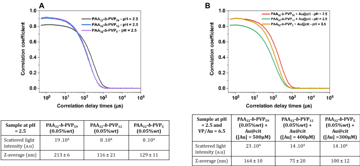
Figure 166. Correlation functions using the NNLS method and associated scattered light intensity measured by a mono-angle DLS instrument for samples containing PAA 32 -b-PVP m (0.05%wt) without (A) or with (B) Au@citrate NPs at a fixed VP/Au=6.5, with m corresponding to the DP of PVP, all samples are at pH=2.5 after adding HCl (1M).
