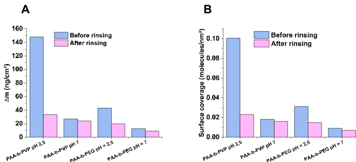
Figure 134. Adsorbed mass per surface unit \Delta m (ng/cm 2 ) (A) and surface coverage (molecules/nm 2 ) (B) calculated values for each polymer system with associated pH, before and after rinsing step in the QCM-D experiments.
