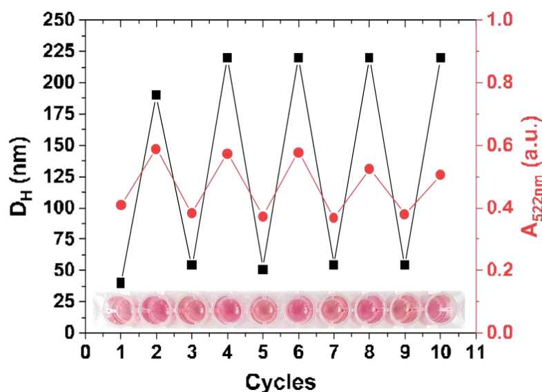
Figure 142. Reversibility study based on D H measurements from DLS (black square) and absorbance values at \lambda = 522 nm from UV-vis spectroscopy analysis (red circles) realized during 5 cycles of assembly and disassembly of PAA 32 -b-PVP 59 + Au@citrate sample at pH=9 and pH=2.5. [PAA 32 -b-PVP 59 ] = 0.05%wt; [Au] = 500 \mu M.
