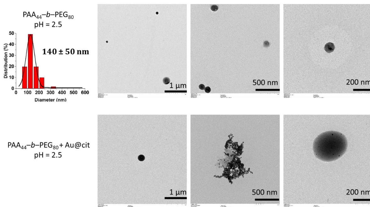
Figure 153. TEM pictures of the samples containing \text{PAA}_{44}\text{-}b\text{-PEG}_{80} (0.05%wt) without (first line) and with Au@citrate NPs (second line) ( [\text{Au}]=500 \mu\text{M} ). Distribution size analysis for the sample \text{PAA}_{44}\text{-}b\text{-PEG}_{80} (0.05%wt).
