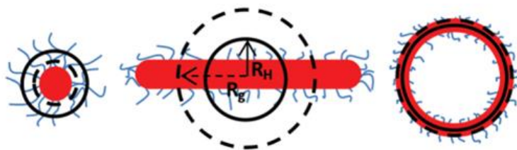
Figure 23. Schematic depicting how different morphologies would display a different R_g/R_H ratio where R_g is the radius indicated by the dashed black line and R_H is the radius indicated by the solid black line
