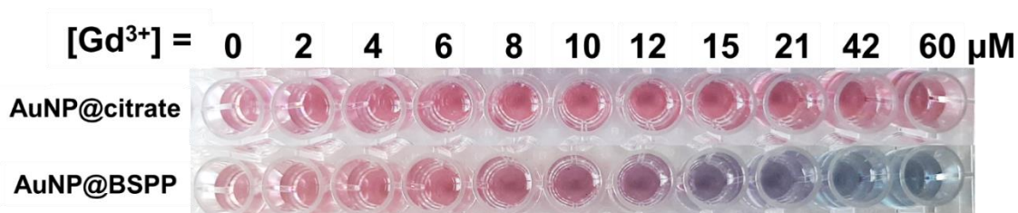
Figure 82. Photographs showing the color response of AuNP@citrate (first line) and of AuNP@BSPP (second line) solutions after incubation with increasing concentrations of Gd^{3+} . Both AuNPs solutions were used at the same concentration of 0.14 mM gold ions or circa 1 nM AuNPs of 17 nm in size.
