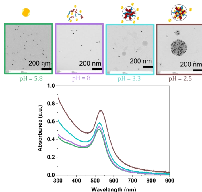
Figure 148. UV-vis spectra of the samples containing Au@citrate: Au@citrate alone, mixed with PAA 32 - b -PVP 59 at pH=8, mixed with self-assembled PAA 32 - b -PVP 59 at pH=3.3 and mixed with PAA 32 - b -PVP 59 at pH=2.5 with associated TEM pictures and schematic representation of the systems.
