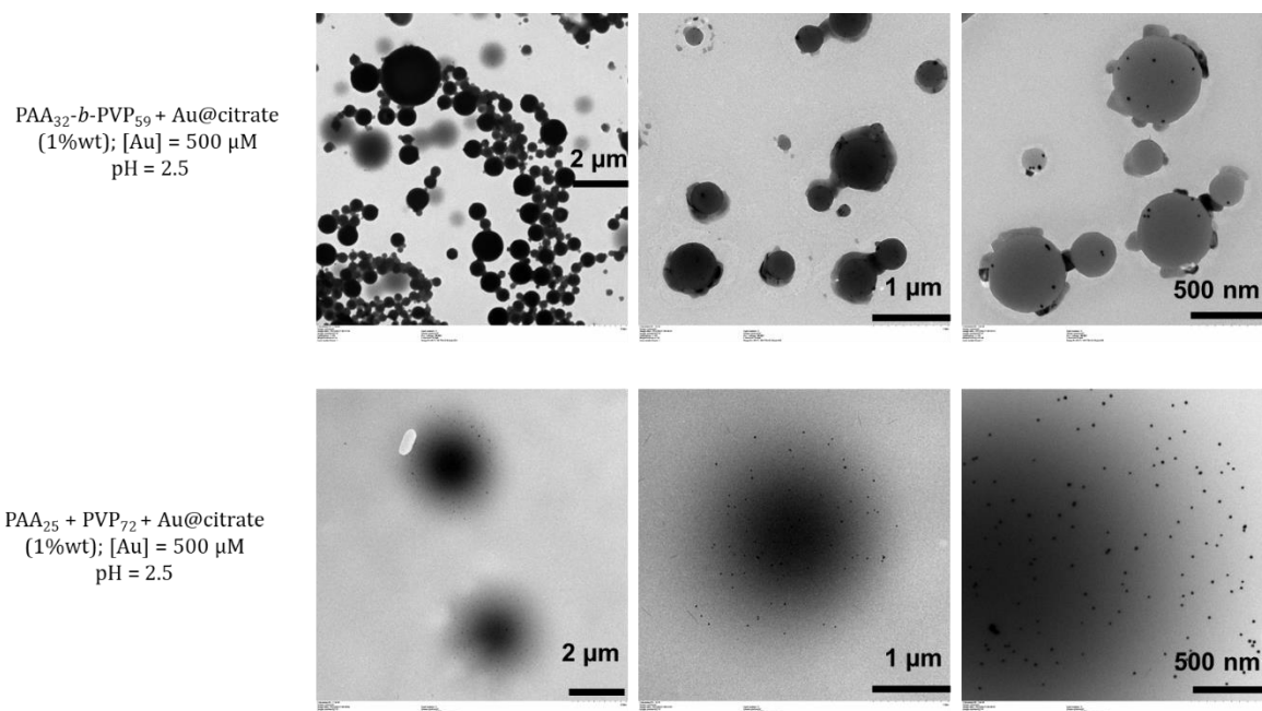
Figure 162. TEM pictures of the samples containing \text{PAA}_{32}\text{-}b\text{-PVP}_{59} (1%wt) (A) or \text{PAA}_{25} + \text{PVP}_{72} (1%wt) (B) and Au@citrate NPs ( [\text{Au}] = 500 \mu\text{M} ) at pH=2.5 after adding HCl solution (1M)
