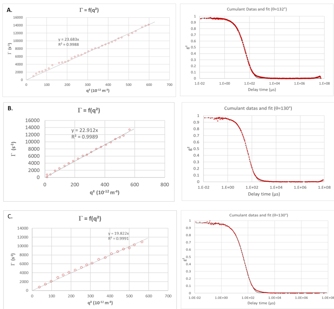
Figure 37. Multi-angle DLS of (A) \text{Gd}^{3+}/\text{PAA}_{32}\text{-}b\text{-PVP}_{59} , (B) \text{Eu}^{3+}/\text{PAA}_{32}\text{-}b\text{-PVP}_{59} and (C) \text{Y}^{3+}/\text{PAA}_{32}\text{-}b\text{-PVP}_{59} HPICs ( R=1 ). Left: Decay rate \Gamma versus the scattering vector q obtained with cumulant method (second order) Right: Typical g^2 correlogram (red circles) obtained for a defined angle. In black, best fit using the NNLS with the M-STORMS software
