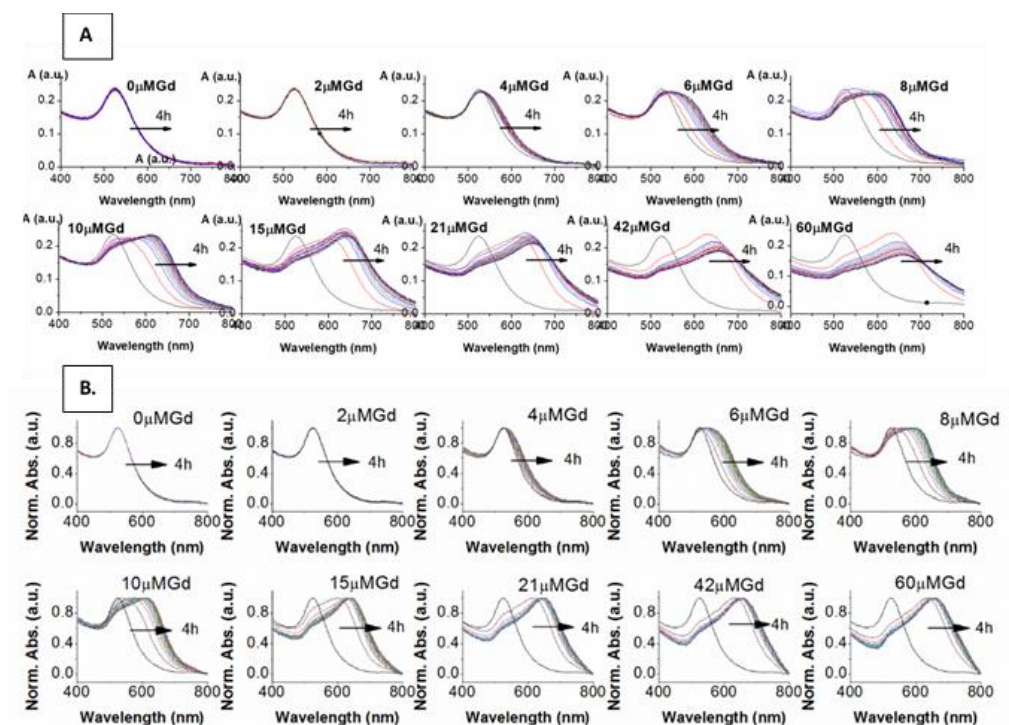
Figure 85. Evolution of the UV-vis spectra as a function of time for AuNP@BSPP upon addition of increasing concentration of Gd^{3+} (measurement time interval 15 minutes for a period of 4h). Gold concentration of ca. 0.14 mM estimated in gold ions. (A) Brut absorbance spectra and (B) Normalized absorbance spectra.
