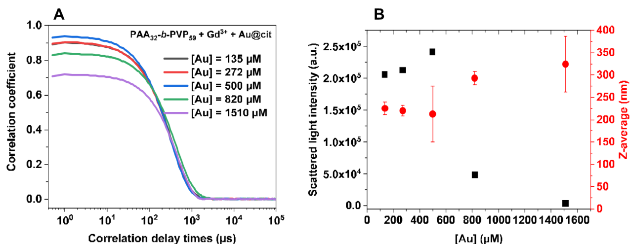
Figure 192. (A) Correlation functions using the NNLS method, (inset) Distribution average size in intensity and (B) Typical evolutions of the scattered light intensity (black squares) and Z-average diameter (red dots) for the sample containing PAA 32 -b-PVP 59 (0.05%wt) + Gd 3+ ions and varying concentrations of Au@citrate NPs: 135; 272; 500; 820; 1510 \mu M at pH=2.5 after adding HCl solution (1M).
