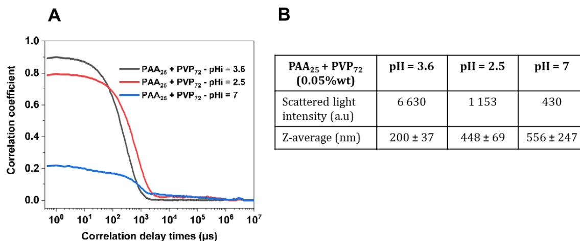
Figure 154. Correlation functions using the NNLS method (A) and Scattered light intensity and Z-average size (B) of the samples containing PAA 25 +PVP 72 (0.05%wt) at three pH values: 3.6; 2.5; 7.
