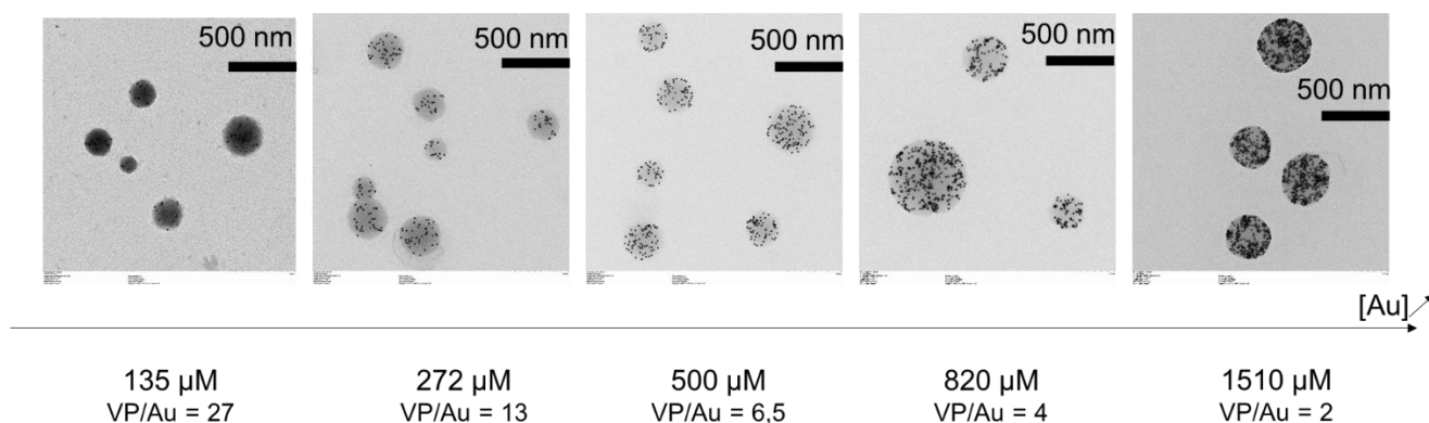
Figure 191. TEM pictures samples containing PAA 32 -b-PVP 59 (0.05%wt) + Gd 3+ ions and varying concentrations of Au@citrate NPs: 135; 272; 500; 820; 1510 \mu M at pH=2.5 after adding HCl solution (1M).
