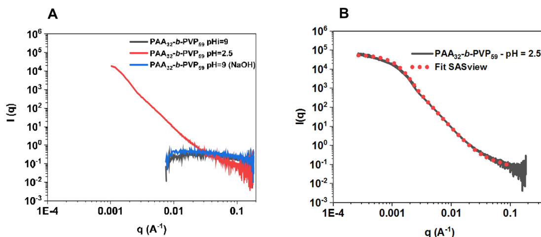
Figure 114. SAXS analysis of PAA 32 -b-PVP 59 block copolymer solution (0.05%wt) at different pH values; pH=9 (black), pH = 2.5 after adding HCl (1M) solution (red) and pH=9 after adding HCl (1M) and then NaOH (1M) solutions (blue) (A) SAXS and SLS analysis combined onto one graph for PAA 32 -b-PVP 59 block copolymer solution (0.05%wt) at pH = 2.5 and fit of the curve (red dots) (B)
