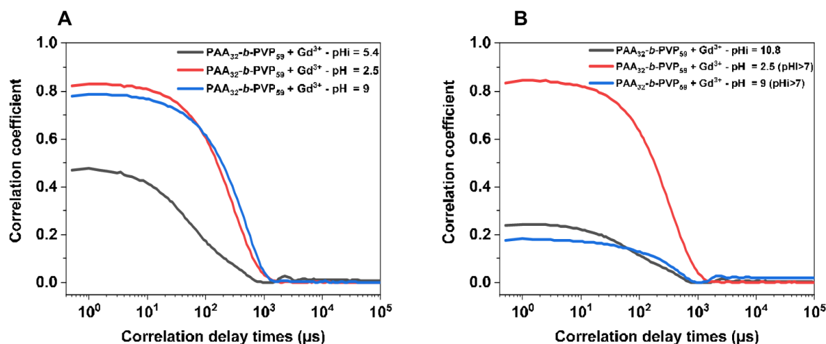
Figure 183. Correlation functions using the NNLS method for the sample containing PAA 32 - b -PVP 59 (0.014%wt) + Gd 3+ ions ([Gd] = 0.2mM) with initial pH of 5.4 (A) 10.8 (B) at varying pH values after adding HCl solution (1M) and then NaOH solution (1M).
