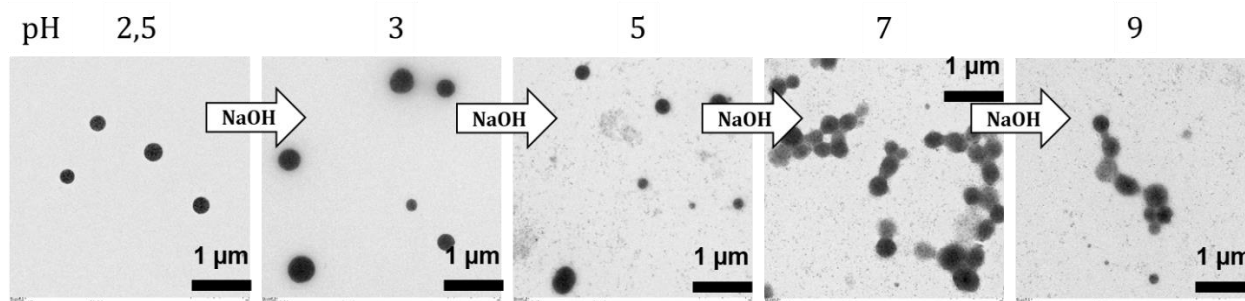
Figure 189. TEM pictures of the sample containing PAA 32 - b -PVP 59 (0.05%wt), Gd 3+ ions (0.7 mM) and in situ AuNPs ([Au]=500 \mu M) at varying pH after adding NaOH solution (1M).
