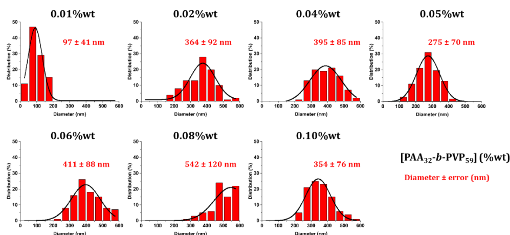
Figure 138. Size distribution diagrams associated to the TEM pictures of the samples with varying PAA 32 - b -PVP 59 concentrations from 0.01 to 0.1 %wt and a fixed [Au]=500 μM at pH=2.5 after adding HCl (1M)
