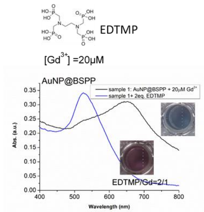
Figure 99. UV-visible spectra of AuNP@BSPP containing 20 \mu M of Gd^{3+} (black curve) and of the same sample after addition of 2 equivalents of EDTMP compared to Gd^{3+} (blue curve)
