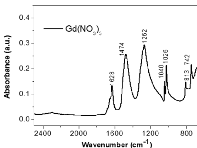
Figure 44. ATR FTIR spectra of \text{Gd}(\text{NO}_3)_3 salt
