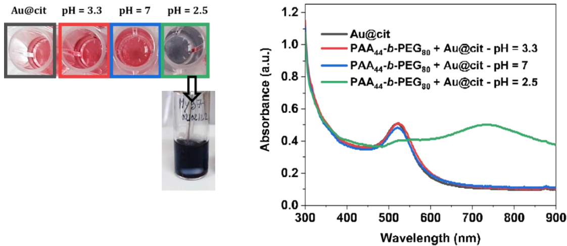
Figure 152. Photos of the wells containing different samples: Au@citrate NPs alone (as a reference) and PAA 44 -b-PEG 80 (0.05%wt) + Au@citrate NPs ([Au]=500 μM) at different pH values: 3.3; 7; 2.5 and corresponding UV-vis spectra.
