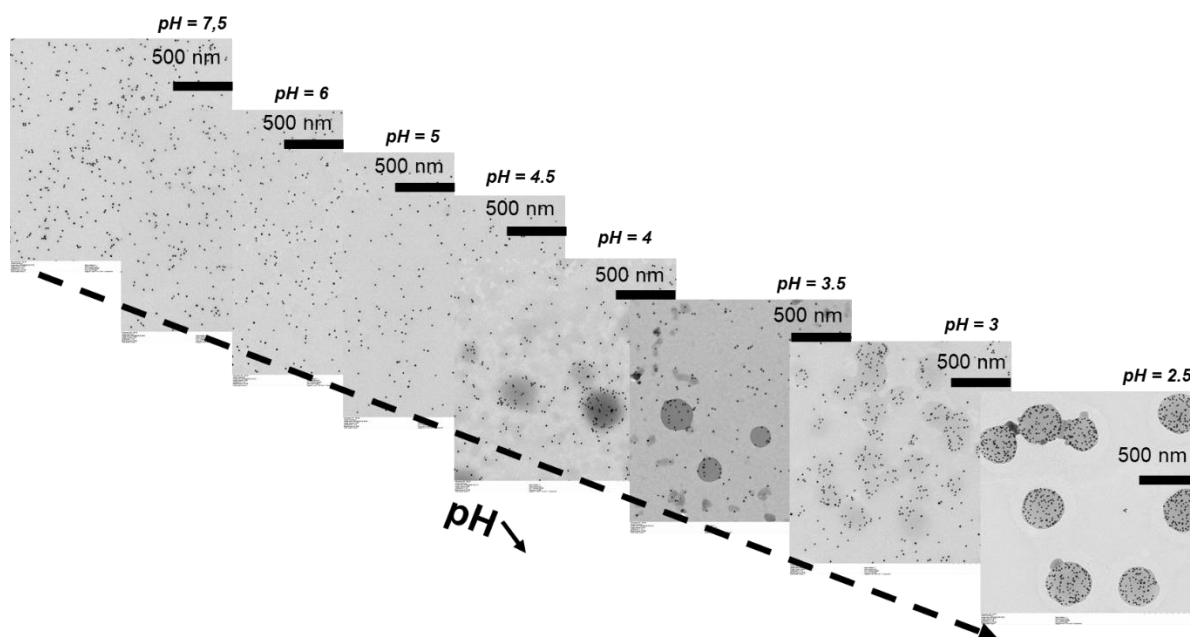
Figure 144. TEM pictures of samples containing PAA 32 - b -PVP 59 (0.05%wt) and Au@citrate ([Au]=500 \mu M) at varying pH after adding progressively HCl solution (1M).
