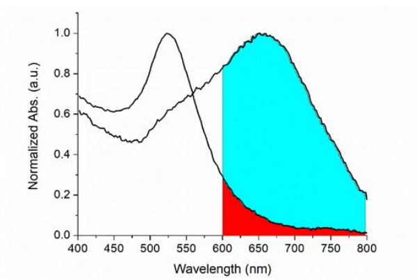
Figure 86. Normalized UV-visible spectra of AuNP@BSPP after and before the incubation with 60 \mu\text{M} of \text{Gd}^{3+} and the representation of the corresponding integrated areas for the subsequent calculation of the flocculation parameter. The blue part corresponds to the flocculation parameter.
