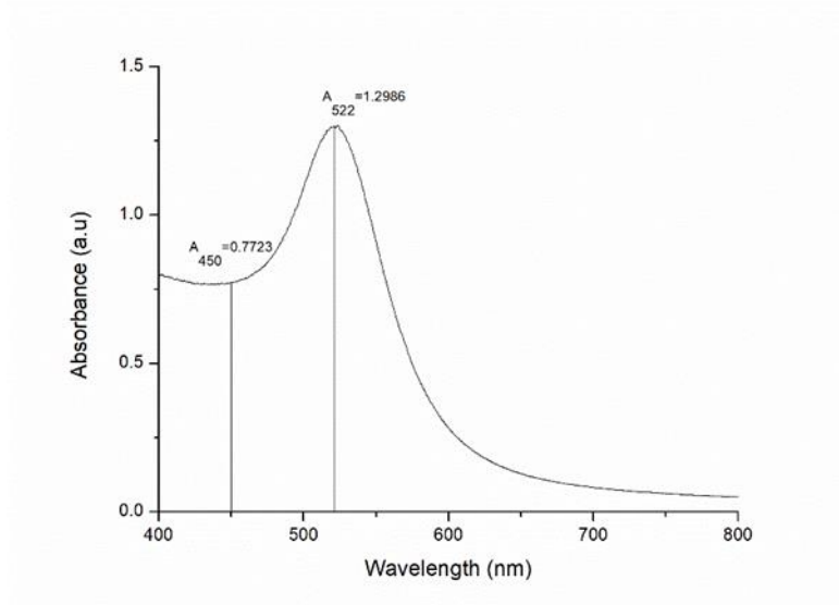
Figure 75. UV-visible Spectra of AuNP@citrate ([Au]=0.28mM)
