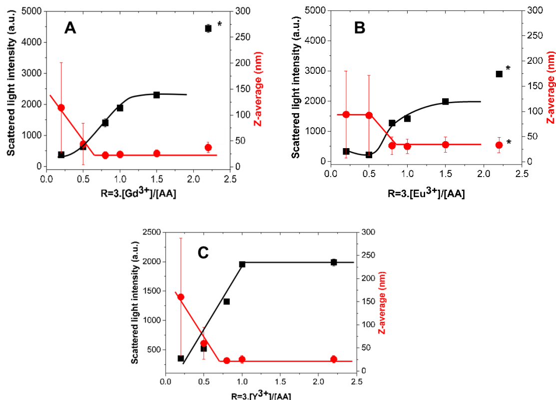
Figure 35. Typical evolutions of the scattered light intensity (black squares) and Z-average diameter (red dots), measured by a mono-angle DLS instrument for \text{Gd}^{3+} (A), \text{Eu}^{3+} (B), \text{Y}^{3+} (C) added to \text{PAA}_{32}\text{-}b\text{-PVP}_{59} as a function of the ratio R . The lines are just guide for the eyes. [\text{PAA-}b\text{-PVP}] = 0.1\% \text{wt} ; \text{pH} = 7
