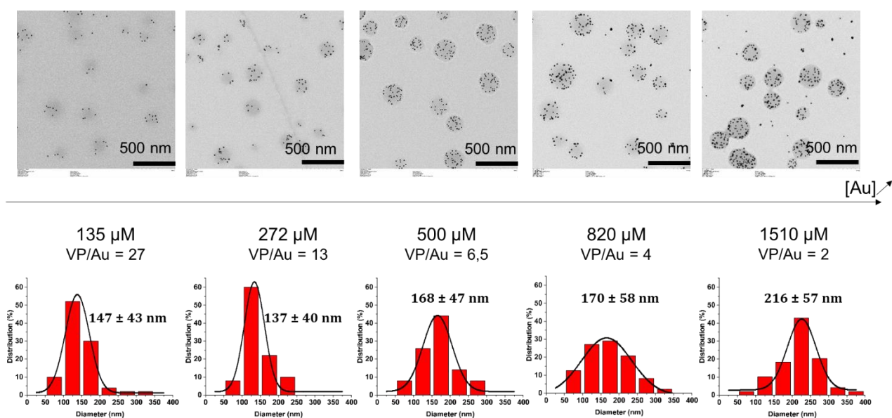
Figure 164. TEM pictures and associated distribution size analysis of samples containing PAA 32 -b-PVP 59 (0.05%wt) and varying concentrations of Au@citrate NPs: 135; 272; 500; 820; 1510 μM at pH=2.5 after adding HCl solution (1M).
