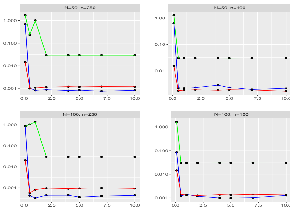
Figure 2: Calibration of the constant \kappa \in \mathcal{V} of the penalty function
