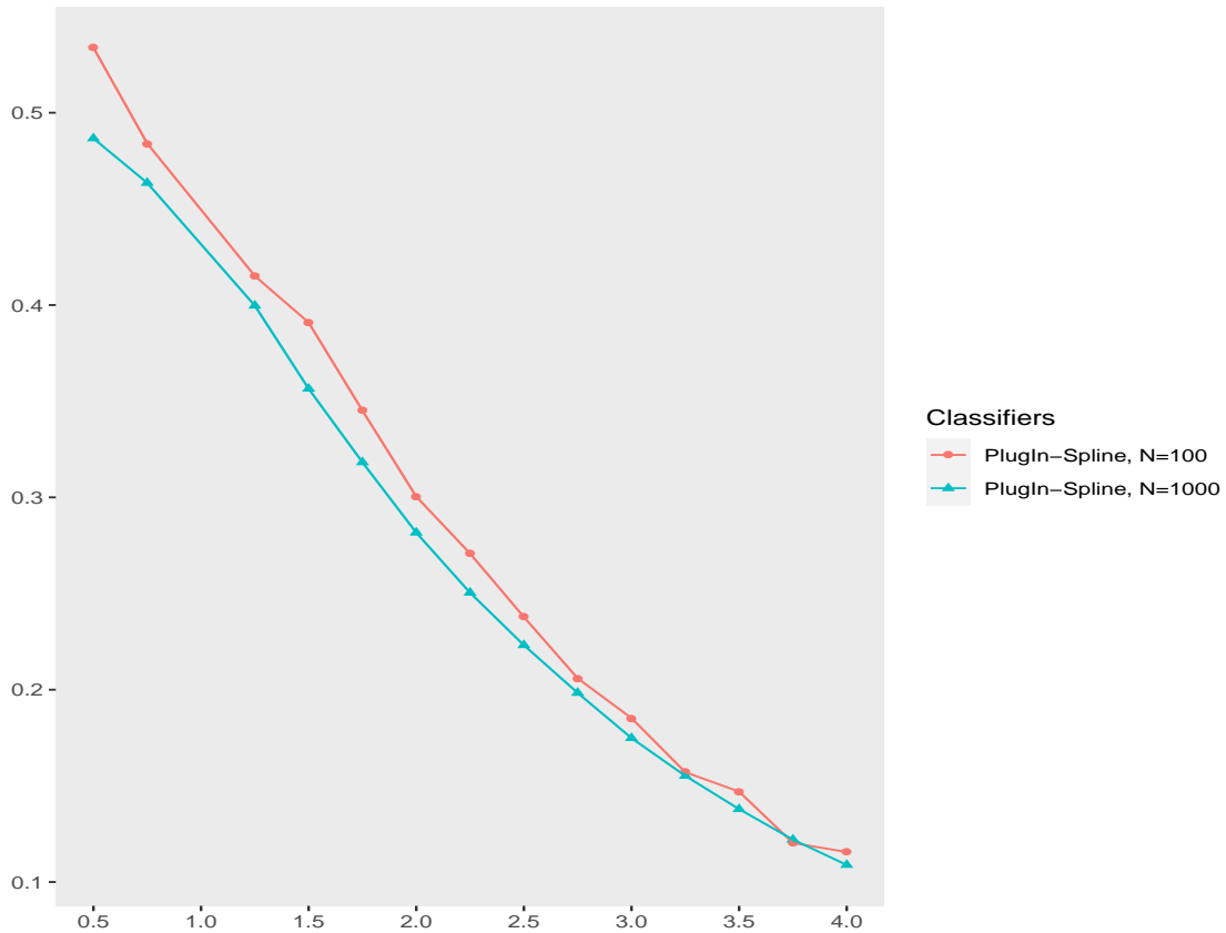
Figure A.2: Risks of the plug-in classifier w.r.t values of the minimum gap \theta between the drift functions
