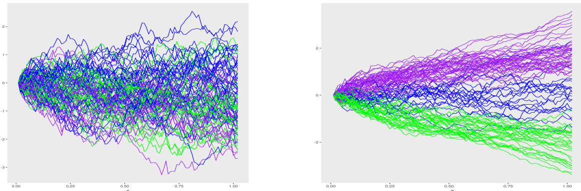
Figure A.1: Dispersion of diffusion paths from model given in Table A.1. Left: \theta = 1/2 , right: \theta = 4 (blue lines K = 1 , purple lines K = 2 , green lines K = 3 ); with N = 100 and n = 100 .
