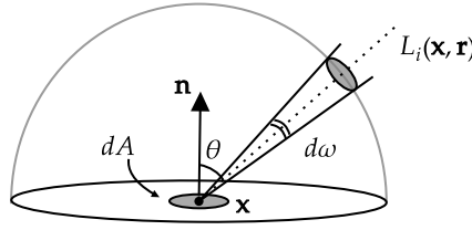
Figure 2.7: Irradiance at a point \mathbf{x} is given by the integral over the hemisphere of radiance multiplied by the cosine of the incident direction angle \theta .
