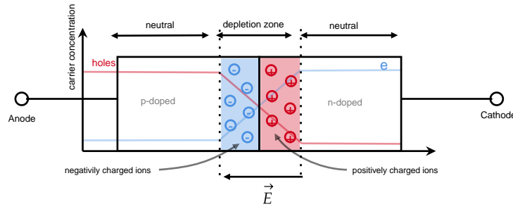
Figure 2.26: PN junction schematic view.
