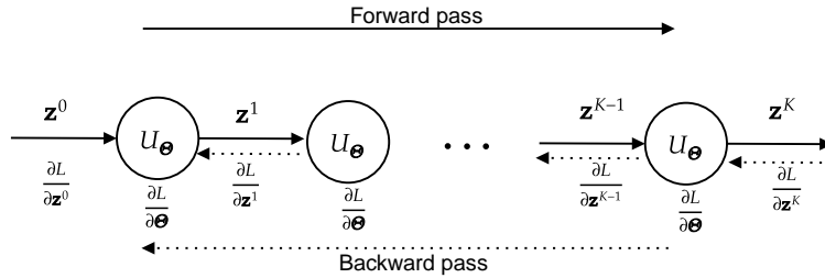
Figure 2.36: Unrolled optimization. Intermediate values need to be accumulated in memory for the backward pass. Therefore, memory consumption grows linearly with the number of unrolled iterations.
