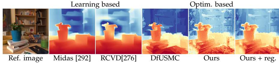
Figure 7.3: Depth estimation from real bursts. We compare the learning-based method and optimization. We present ours result w/o regularisation ( Ours ) and with determinant penalization 7.3 ( Ours + reg. ).
