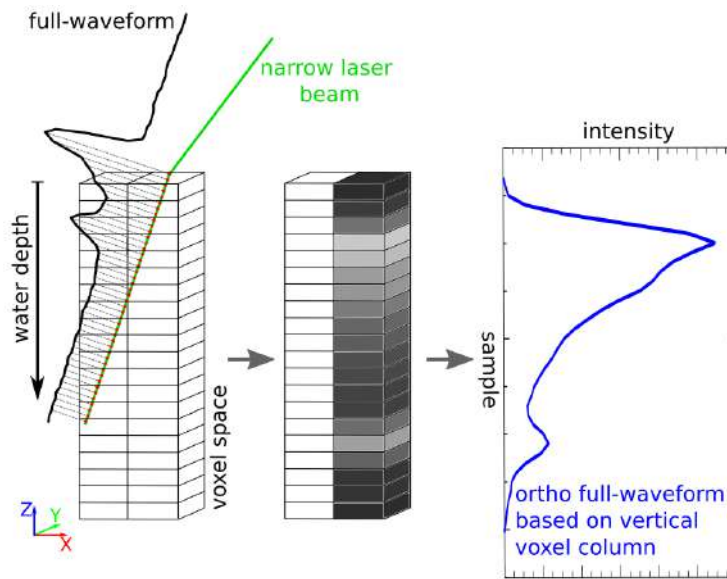
Figure 2.8: Principle of ortho full-waveforms generation, extracted from Richter et al., 2022.
