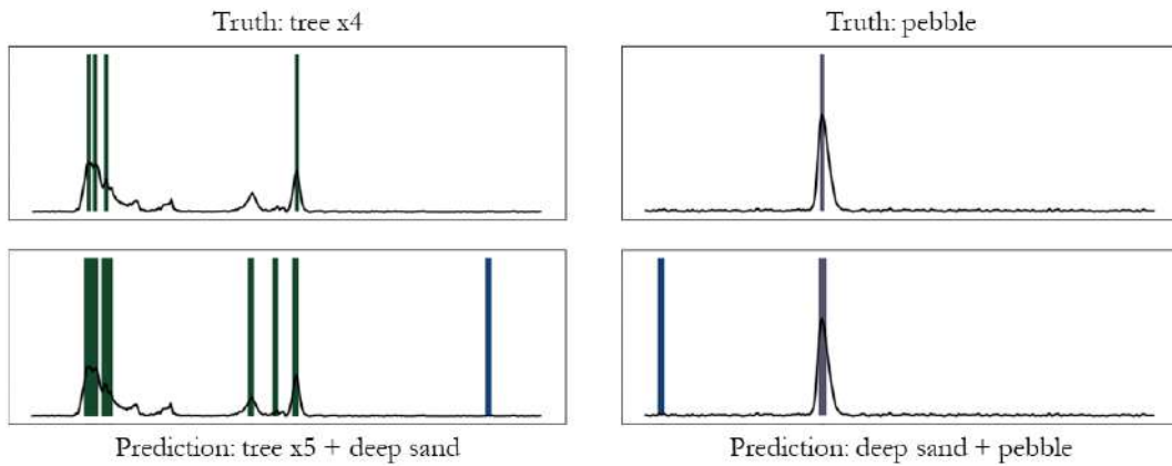
Figure 4.17: Examples of false predictions made by the green waveforms-based U-time. The black signal corresponds to the green waveform. Each coloured vertical line refers to a predicted peak.
