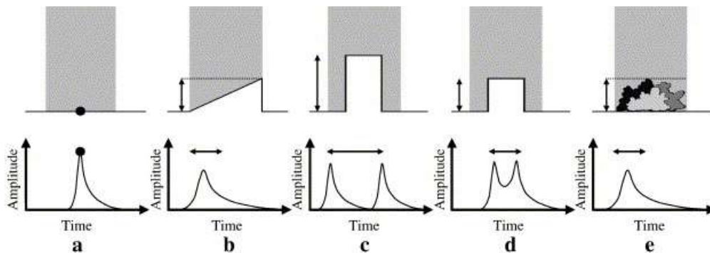
Figure 1.13: Impact of the intercepted surface's geometry on the resulting waveform shape, extract of Jutzi et al., 2006: a) Plane surface, b) sloped surface, c) two significantly different elevated areas, d) two slightly different elevated areas, e) randomly distributed small objects.
