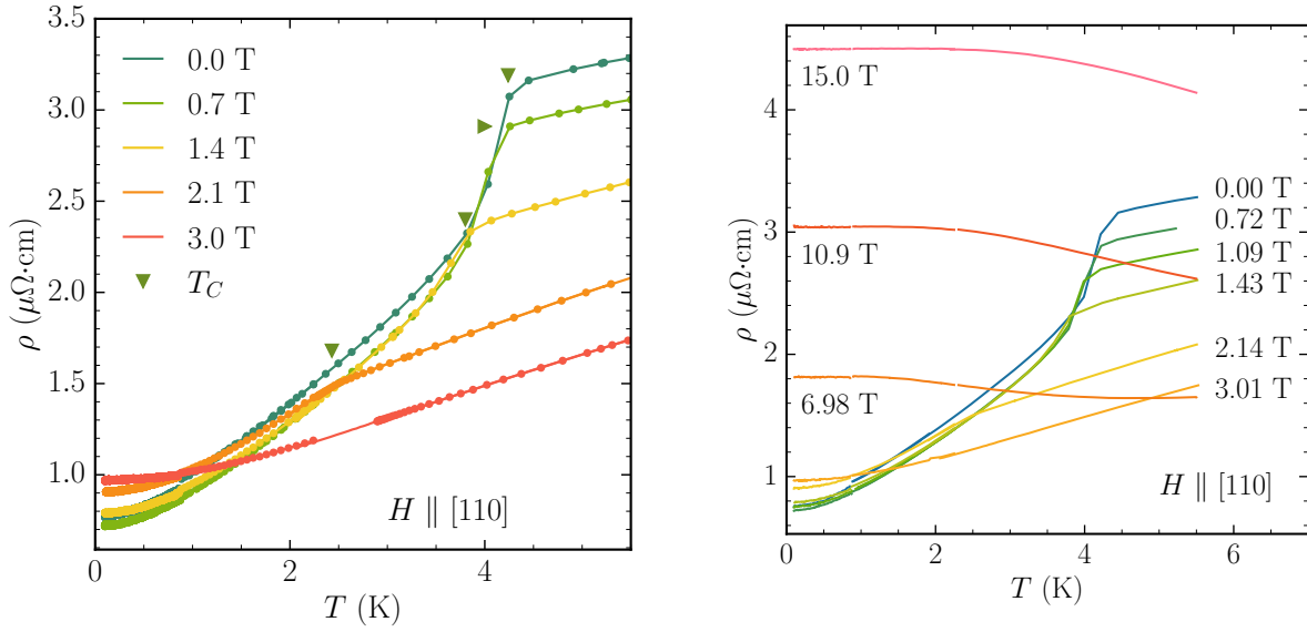
Figure 3.16: Temperature dependence of \rho for fields H \parallel [110] between 0 and 3 T (left) and between 0 and 15 T (right), up to 5.5 K. Green arrows on the left panel indicate the T_C \equiv H_C conical/PM transition. At 0 T, T_C = T_N = 4.1 K.
