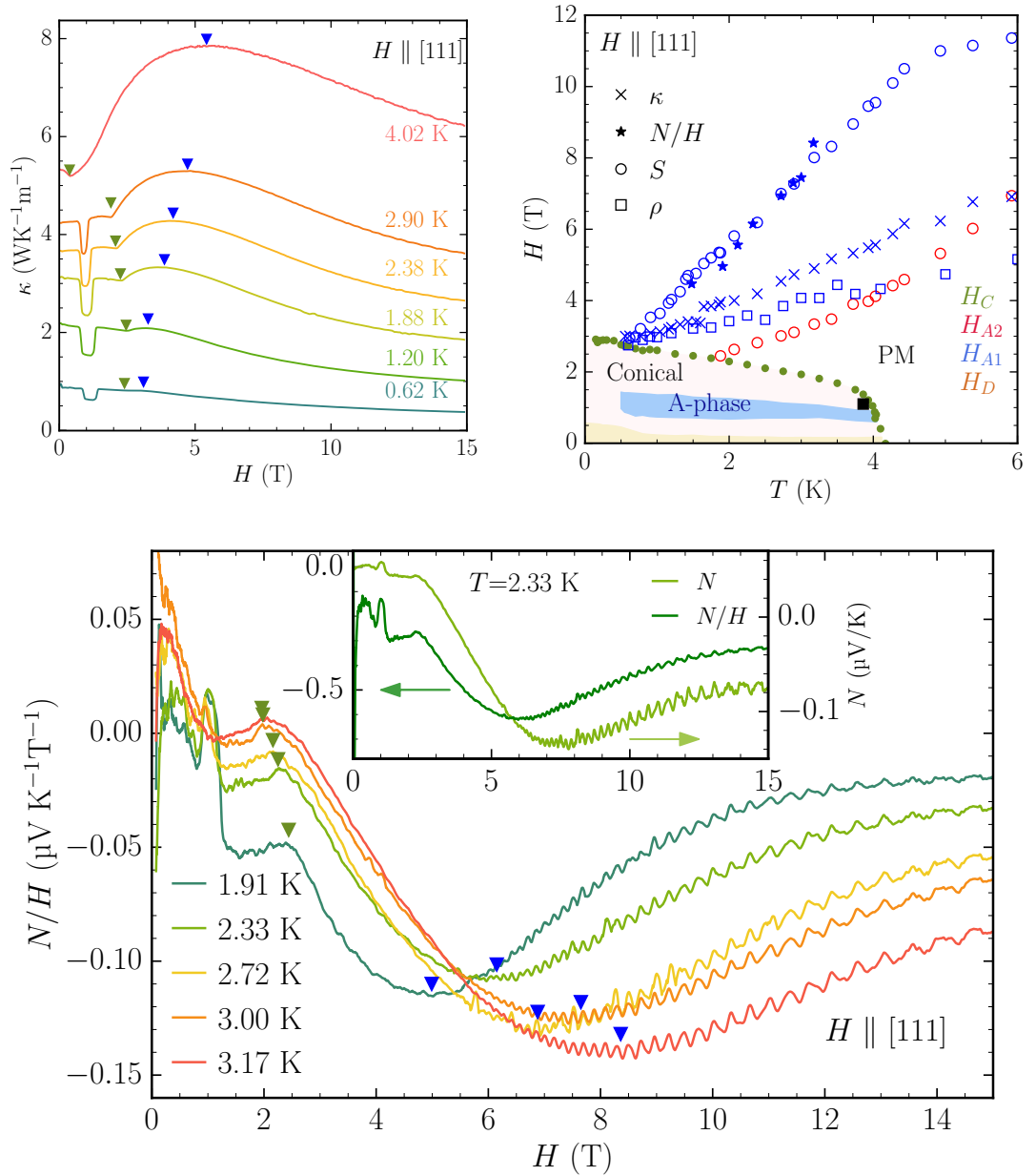
Figure 3.26: Top left: \kappa(H) between 0.6 and 4 K up to 15 T, measured on sample #2. Green arrows indicate the H_C transition and blue arrows indicate the local extrema. Right: H - T phase diagram from \rho (full dots) extended to 6 K and 12 T, with extrema from \kappa (crosses), N (stars), S (circles) and \rho (squares). The black square is the tricritical point determined in [81]. Bottom: N/H field dependence between 1.9 and 3.2 K up to 15 T, for sample #1. Inset: comparison between N (right axis) and N/H (left axis) at 2.33 K.
