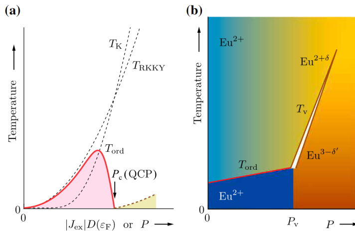
Figure 3.1: (a) Doniach phase diagram showing the suppression of the magnetic ordering temperature T_{\text{ord}} with pressure P . Below T_{\text{ord}} (shaded in pink) is the magnetic ordered region. T_K and T_{\text{RKKY}} are the Kondo and the Ruderman-Kittel-Kasuya-Yosida temperatures, respectively. P_C is the critical pressure corresponding to the quantum critical point (QCP). Above P_C is the quantum critical region (shaded). (b) P - T phase diagram representing the valence transition in Eu compounds. T_V is the first-order valence transition temperature and P_V is the pressure at which the first-order valence transition appears. From [39].
