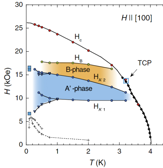
Figure 3.8: H - T phase diagram for the H \parallel [100] direction obtained by magnetization measurements, with the colored A'- and B-phases. TCP indicates the tricritical point. From [4].
