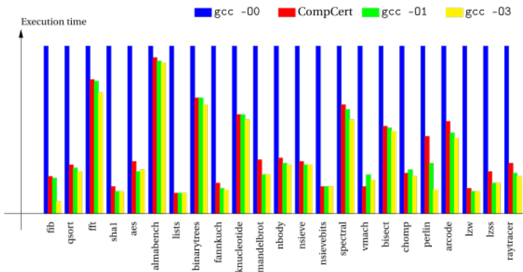
Figure 2.3 – Performance of CompCert-generated code relative to GCC 4.1.2-generated code on a Power7 processor. Shorter is better. The baseline, in blue, is GCC without optimizations. CompCert is in red.
