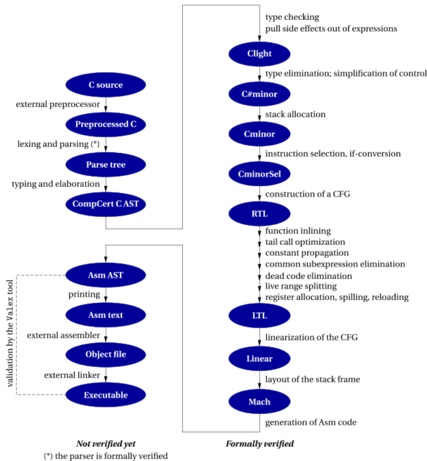
Figure 2.2 – General structure of the CompCert C compiler
