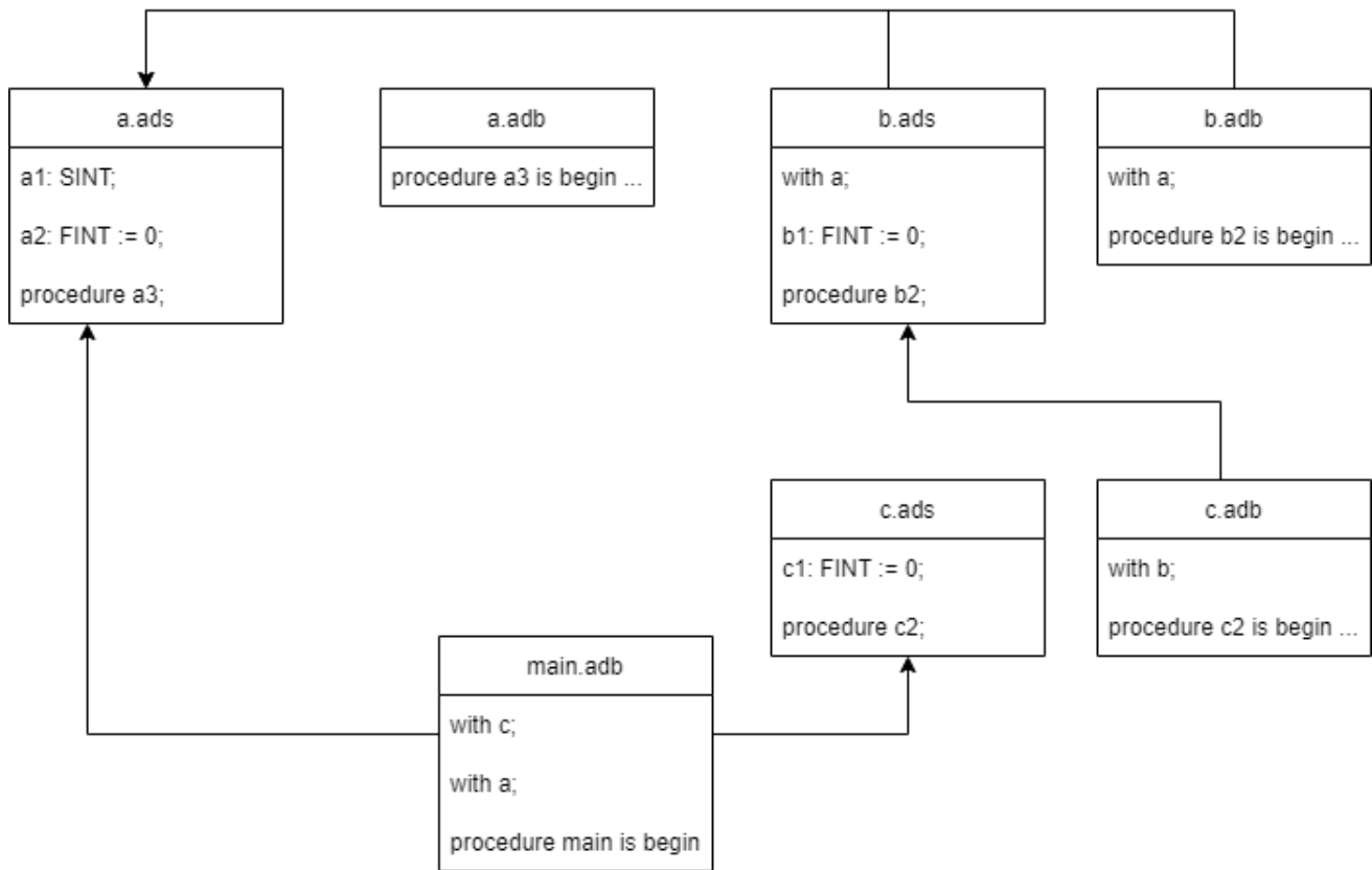
Figure 6.1 – Example of a VCP Ada program structure
