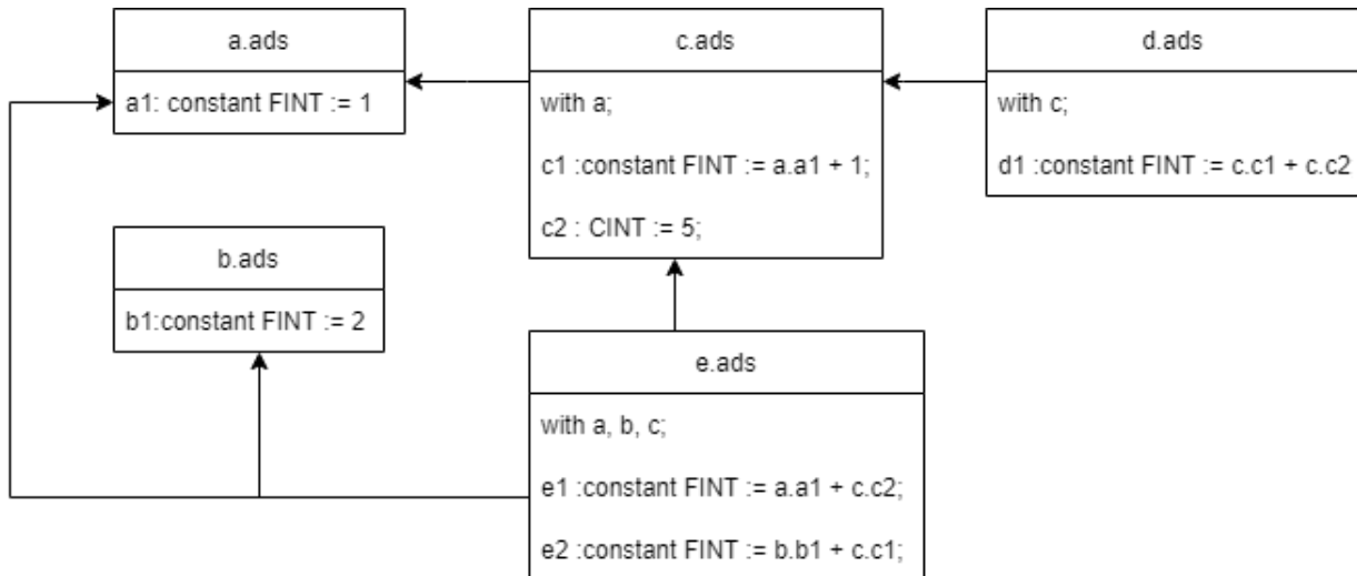
Figure 8.1 – Example of a VCP Ada program structure
