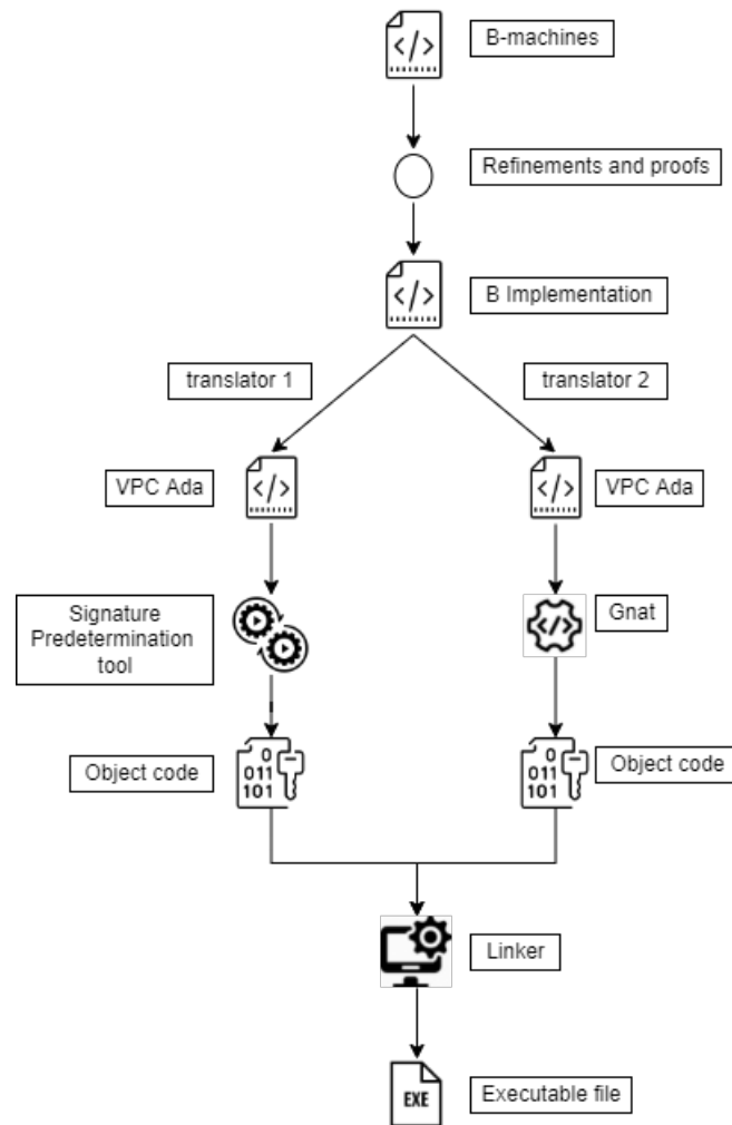
Figure 3.3 – DigiSafe® Development process
