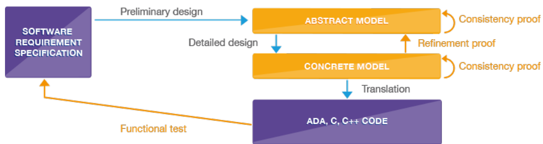
Figure 2.1 – B-method software design
