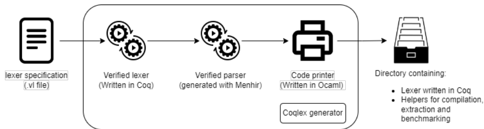
Figure 5.5 – General structure of the Coqlex lexer generator.
