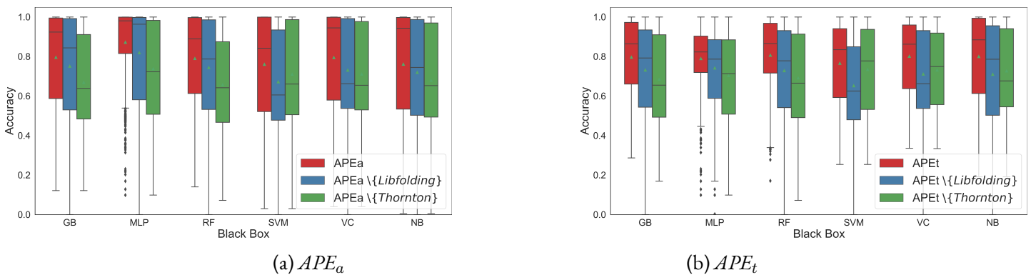
Figure 3.11 – Average accuracy per black box computed on 100 instances of the tabular datasets for APE_a in (a) and for APE_t in (b) when we remove the Libfolding unimodality and linear separability tests from the APE Oracle.
