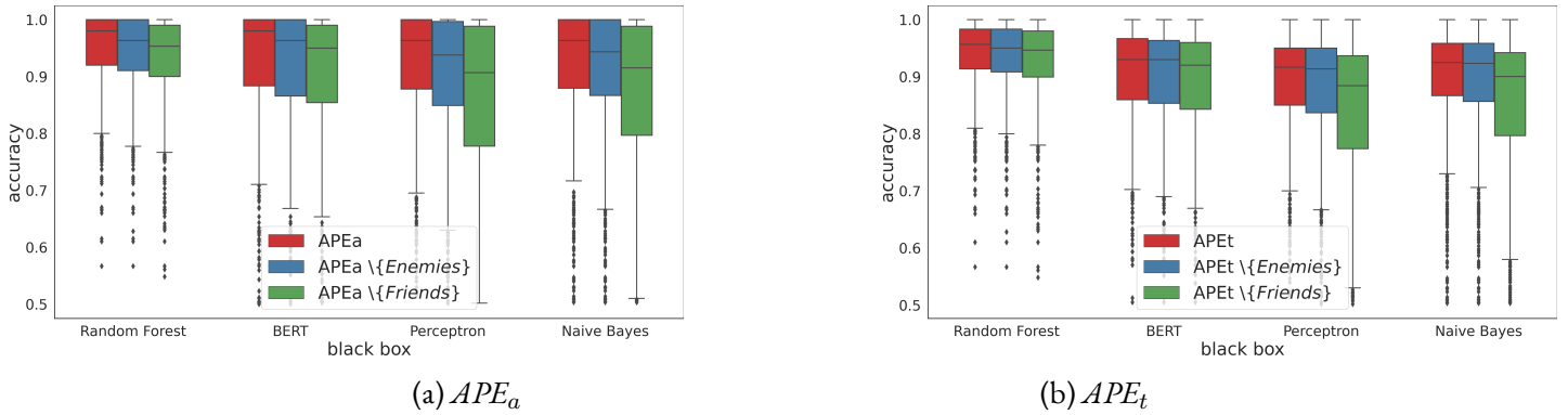
Figure 3.12 – Average accuracy attained by APE_a in (a) and for APE_t in (b) across different black-box models and textual datasets. The computation is based on 100 instances sampled from the experimental datasets. The results are displayed for both methods using the Libfolding unimodality test from the APE Oracle, on the friends or enemies instances.
