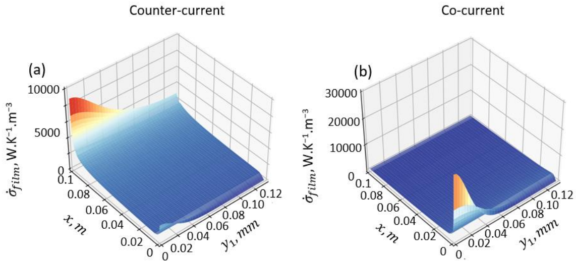
Figure 2.7: Thermal entropy generation through the film for both co and counter-current configurations, Re_{htf} = 1000 , Re_f = 49.8 , e_{htf} = 2mm and \Delta T = 0 K
