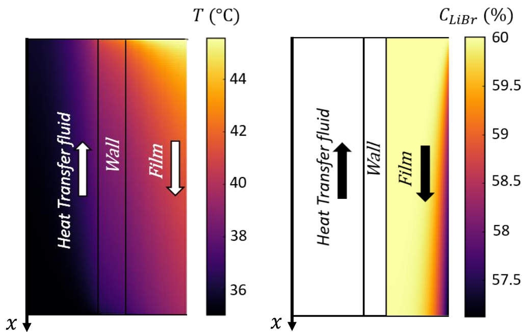
Figure 3.5: Local temperature and concentration profiles for Re_{\text{htf}} = 2000
