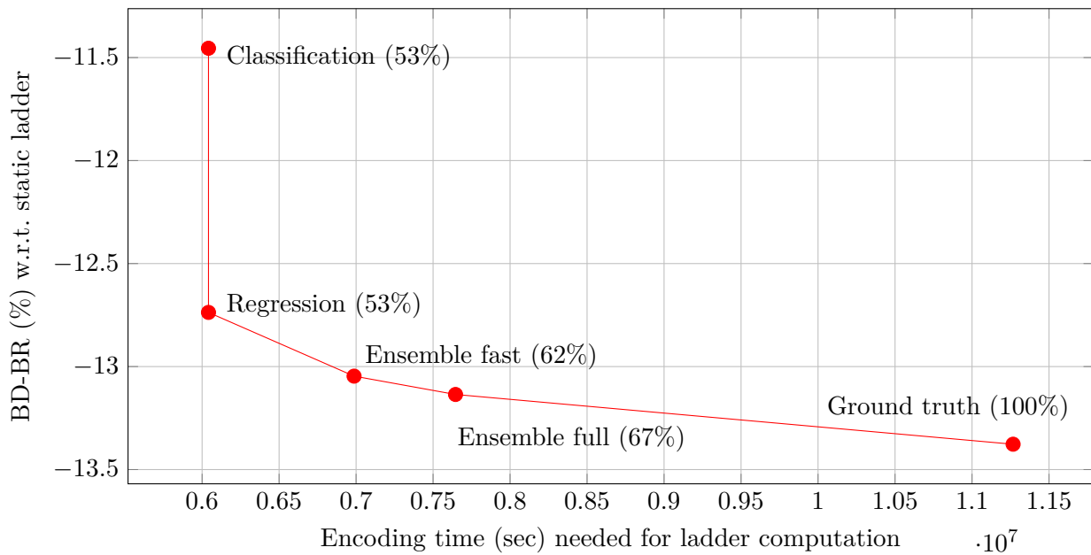
Figure 4.16 – BD-BR vs. complexity evolution of different methods. The numbers in parenthesis indicate the overhead in terms of encoding time with respect to the GT method as a reference.
