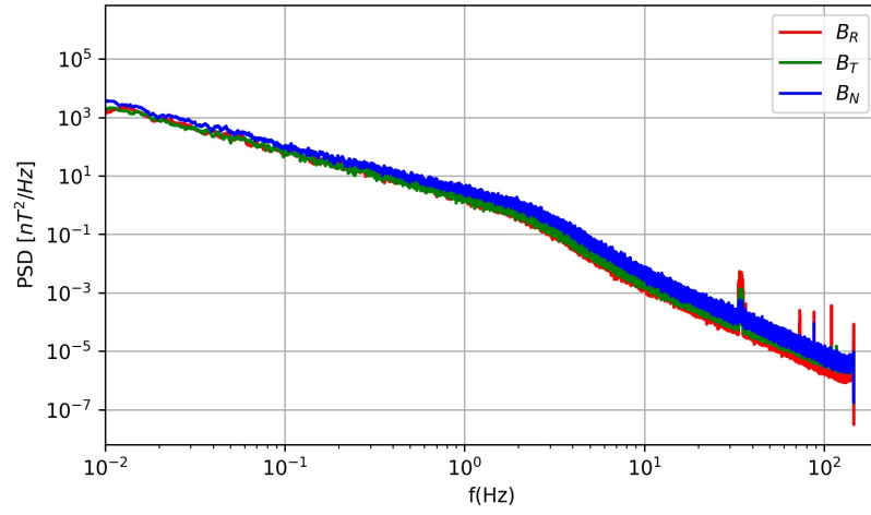
Figure 2.7: Power spectral density of magnetic field components ( B_R, B_T, B_N ) for the analysed time interval of 5h during the E1 of PSP. At high frequencies (corresponding to sub-ion scales) the power spectral density of B_R (red line) is less energetic than for the other two components.
