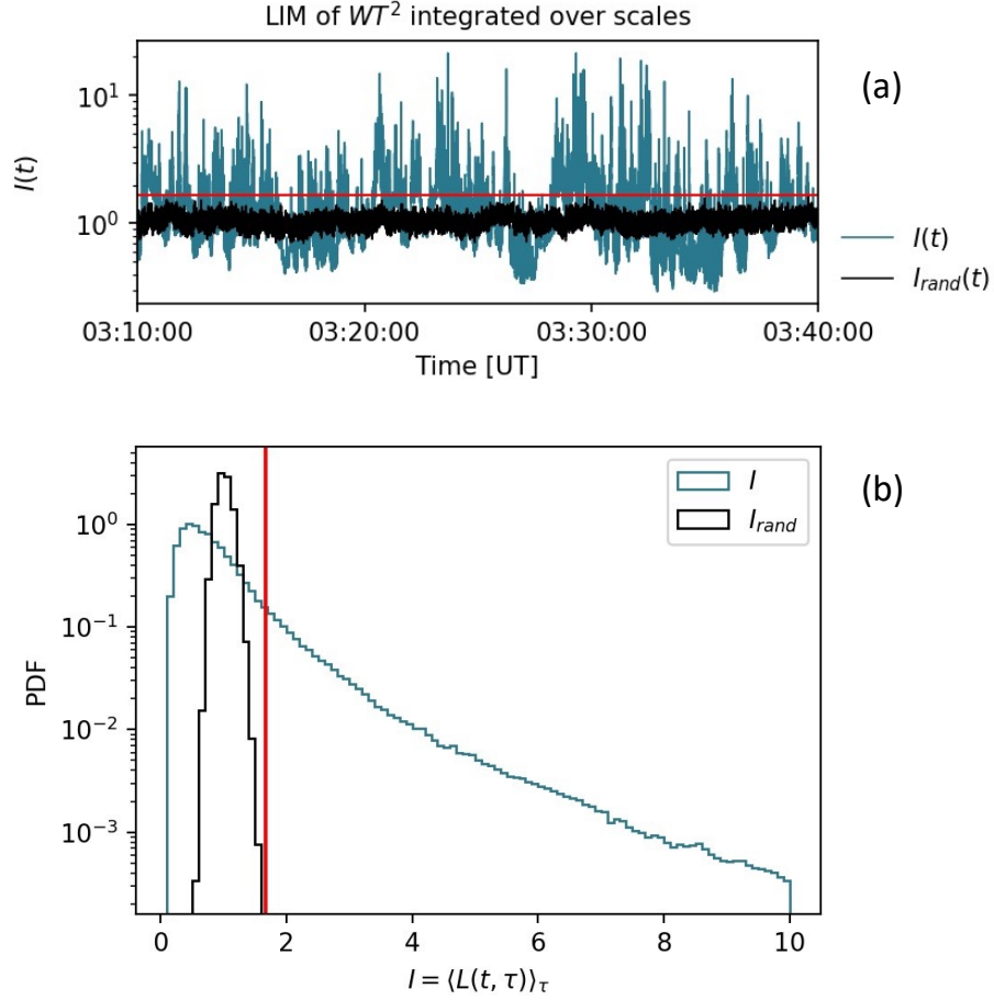
Figure 4.2: (a) the comparison of the integrated LIMs I(t) = \langle L(t, \tau) \rangle_{\tau \in [10^{-2}, 10^3] \text{ s}} (blue), and the I_{rand}(t) = \langle L_{rand}(t, \tau) \rangle_{\tau \in [10^{-2}, 10^3] \text{ s}} (black). The horizontal red line shows I_{threshold} = \max(I_{rand}(t)) as defined in panel (b) with a red vertical line. (b) Histograms of the integrated LIM I(t) and the random phased integrated LIM I_{rand}(t) .
