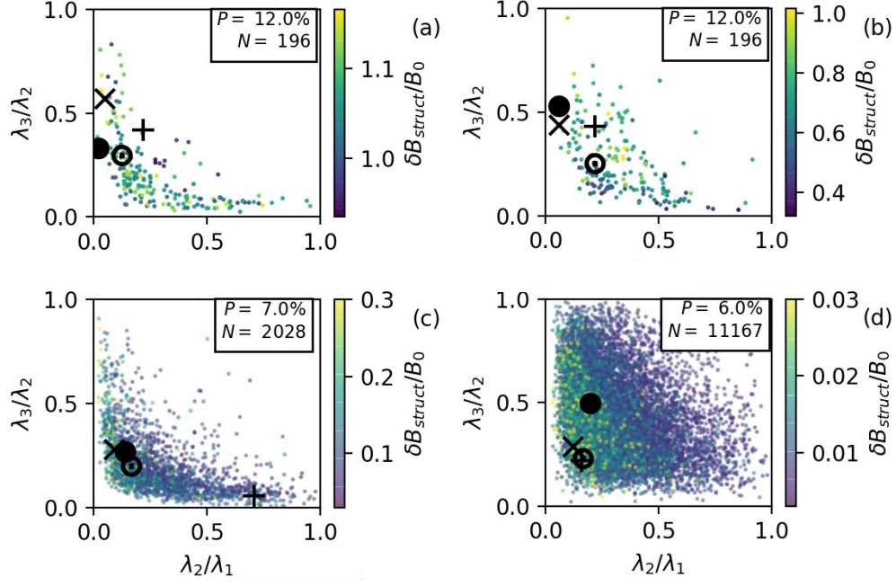
Figure 4.6: Minimum variance analysis eigenvalues ratios plane ( \lambda_2/\lambda_1, \lambda_3/\lambda_2 ): each dot corresponds to an observed coherent structure, the color gives its amplitude \delta B_{struct}/B_0 . Panels (a,b) correspond to the raw data and MHD scales, respectively. They include 196 structures found at MHD scales. Panel (c) provides the eigenvalues ratios for 2028 structures at ion scales and panel (d) for 11167 events at sub-ion scales. The filling factor P and the number of detected coherent structures N at different frequency ranges are shown in the panel legends. The eigenvalue ratios of the example structures from Figures 4.3 and 4.4 are shown by the black marks: "circle", "cross", "plus" and "odot", respectively. They correspond to the example structures 1-4, respectively.
