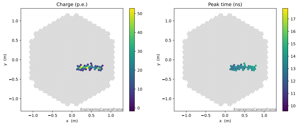
Figure 12.4: The integrated charge and peak time images for one simulated gamma after cleaning
