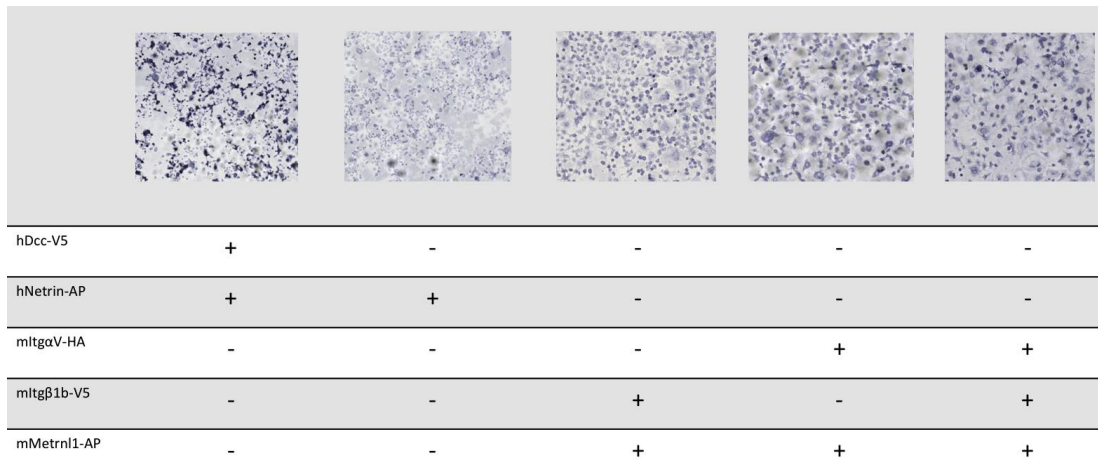
Figure 25: Via an AP-binding assay no positive interaction between Metrn1 and Integrin \alpha V/Integrin \beta 1b could be detected: An example of an AP-binding assay showing positive interaction (dark colored cells) in the control between the Dcc receptor expressed in COS7 cells and Netrin-AP. No interaction (just light blue colored cells) could be detected between Integrin \alpha V and/or Integrin \beta 1b and Metrn1.
