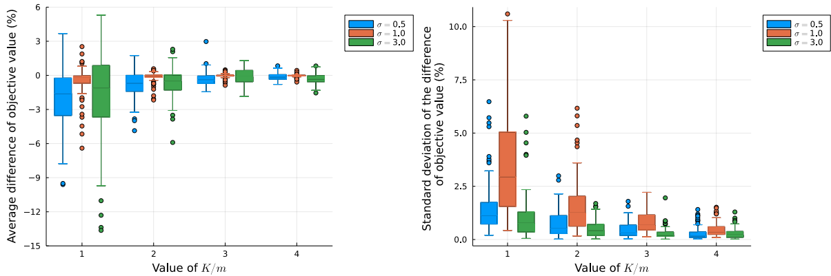
Figure 3.10 – Average (left) and standard deviation (right) of the relative difference between the objective values z_{SVC} and z_{AC} for the robust lot sizing problem.
