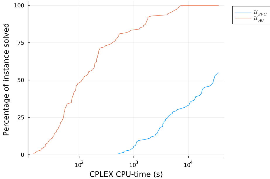
Figure 3.12 – Proportion of TSP instances solved for \mathcal{U}_{SVC} and \mathcal{U}_{AC} K/m = 3
