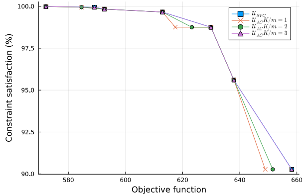
Figure 3.8 – Trade-off between objective value and constraint satisfaction of \mathcal{U}_{SVC} and \mathcal{U}_{AC} for different values of K/m
