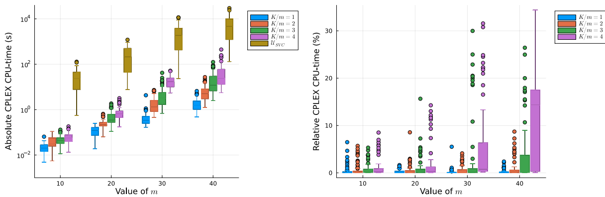
Figure 3.7 – Absolute (left) and relative (right) solving time of \mathcal{U}_{AC} as a function of m for the robust knapsack problem with different values of the ratio K/m
