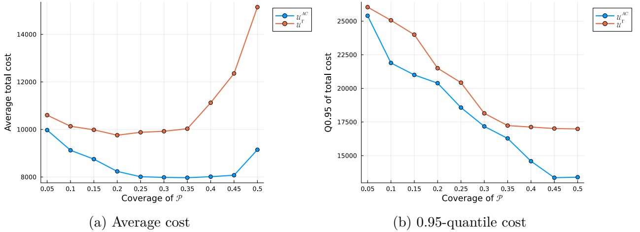
Figure 4.2 – Evolution of the average cost and 0.95-quantile obtained with \mathcal{U}^{\Gamma} and \mathcal{U}^{AC} on an instance with 5 components 10 products and planning horizon T = 14 periods.
