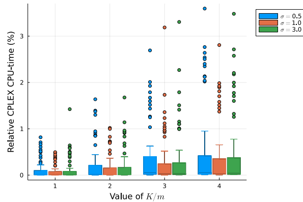
Figure 3.11 – Solving time of \mathcal{U}_{AC} in percent of the solving time of \mathcal{U}_{SVC} as a function of K/m for different values of \sigma (Robust lot sizing problem)
