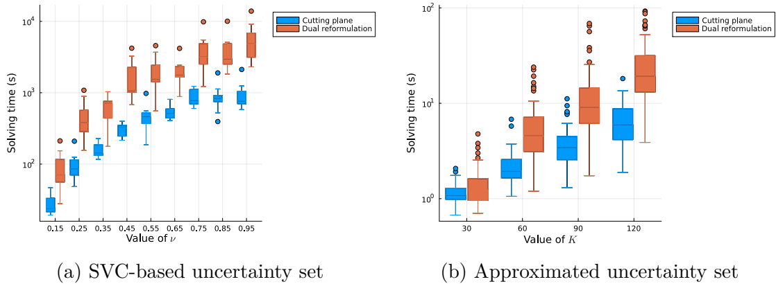
Figure 6.1 – Computation time of dual reformulation and cutting plane method for the binary knapsack problem with 30 items using the SVC-based uncertainty set and our approximation.
