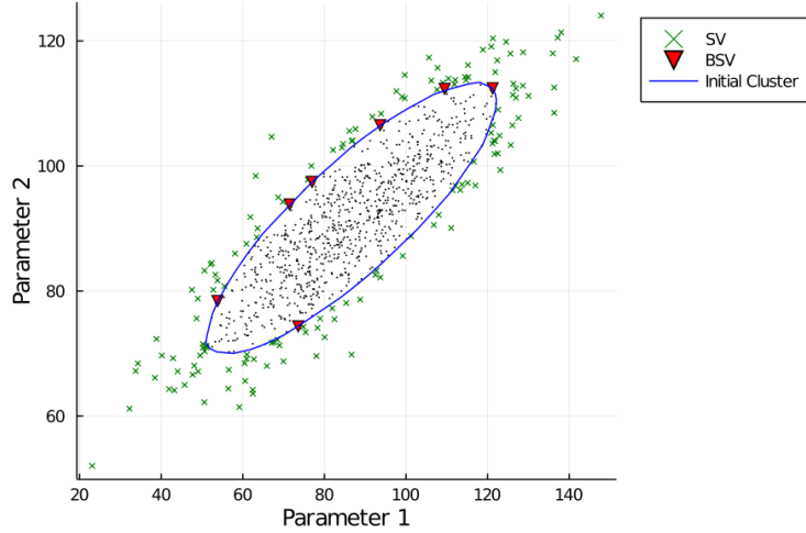
Figure 3.2 – Representation of \mathcal{S} and \mathcal{B} for a bivariate gaussian distribution when \nu = 0.15
