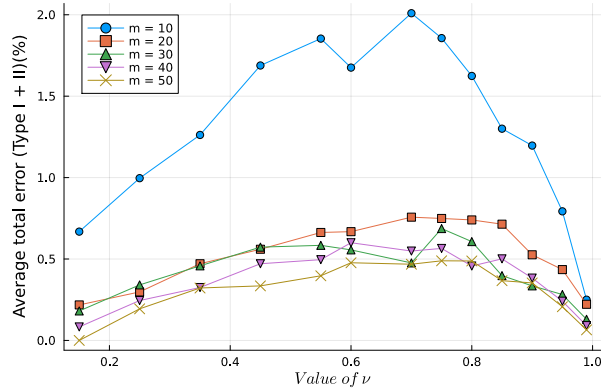
Figure 3.5 – Evolution of the cumulative error as a function of \nu for a multivariate Gamma distribution when N = 1000, K/m = 3
