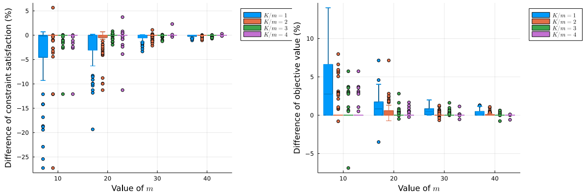
Figure 3.6 – Relative constraint satisfaction (left) and objective function (right) difference in percent for the knapsack problem
