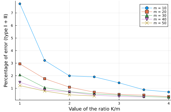
Figure 3.4 – Evolution of the out-of-sample cumulative error as a function of the ratio K/m for a multivariate Gamma distribution when N = 1000
