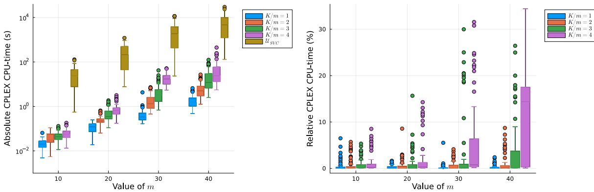
Figure 3.7 – Absolute (left) and relative (right) solving time of \mathcal{U}_{AC} as a function of m for the robust knapsack problem with different values of the ratio K/m
