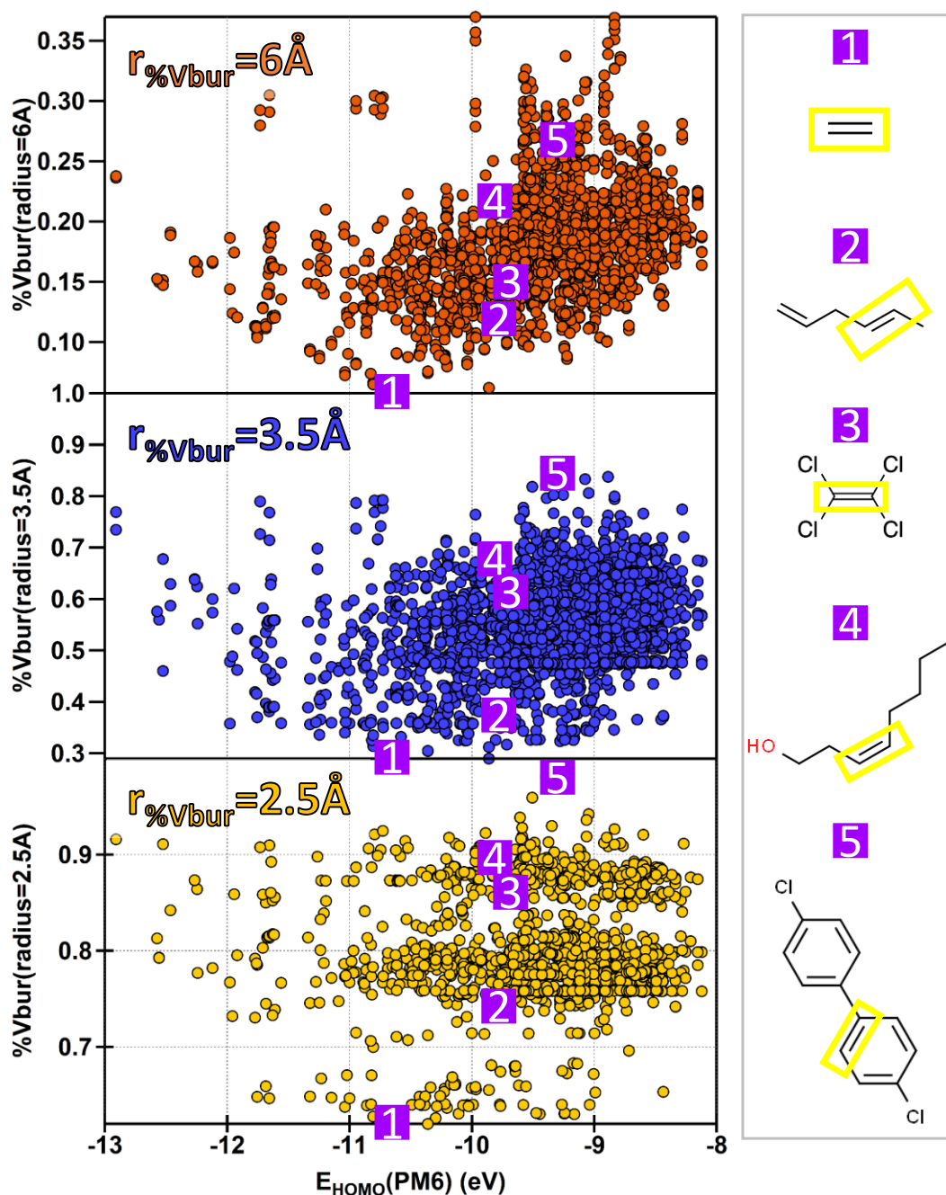
Figure App-IV-1 : Buried volumes for different r_{\%V_{\text{bur}}} (2.5, 3.5, and 6 Å) as a function of E_{\text{HOMO}} calculated using PM6. Example molecules are located on each of the panels and were chosen for their structure (short/long chain, alkyl substituted or chlorinated) to assess the bulkiness of the substituents attached to the olefinic bond. Additionally, these molecules have a similar E_{\text{HOMO}} , which allows us to assess the impact of the different values of buried volumes since the other main variable of the multivariate linear regression ( E_{\text{HOMO}} ) will be approximately constant. From the simplest UVOC, ethene (compound 1), to tetrachloroethene (compound 2) substituted with bulky chlorine atoms, and longer chain alkenes and benzenoids. These plots highlight how larger r_{\%V_{\text{bur}}} can distinguish longer chain alkenes, while smaller r_{\%V_{\text{bur}}} includes mostly the alkyl groups and close neighbors (e.g., difference of values for compounds 3 and 4 that are very similar for r_{\%V_{\text{bur}}} 2.5 Å and 3.5 Å and starts to be distinct for r_{\%V_{\text{bur}}} 6 Å). We chose the r_{\%V_{\text{bur}}} accordingly, for \text{O}_3 and \text{NO}_3 a larger r_{\%V_{\text{bur}}} is more adapted, while for OH and Cl a smaller r_{\%V_{\text{bur}}} is better. This highlights the
