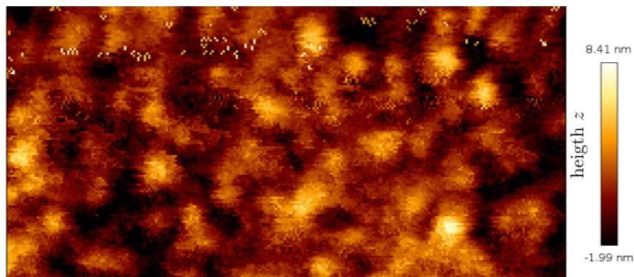
Figure 9.10: 250 \times 500 \text{ nm} AFM map of the surface of a sphere after gold deposition. The structure of the gold layer can be seen. The measured roughness is \sqrt{\langle z^2 \rangle} = 2.5 \text{ nm} rms.
