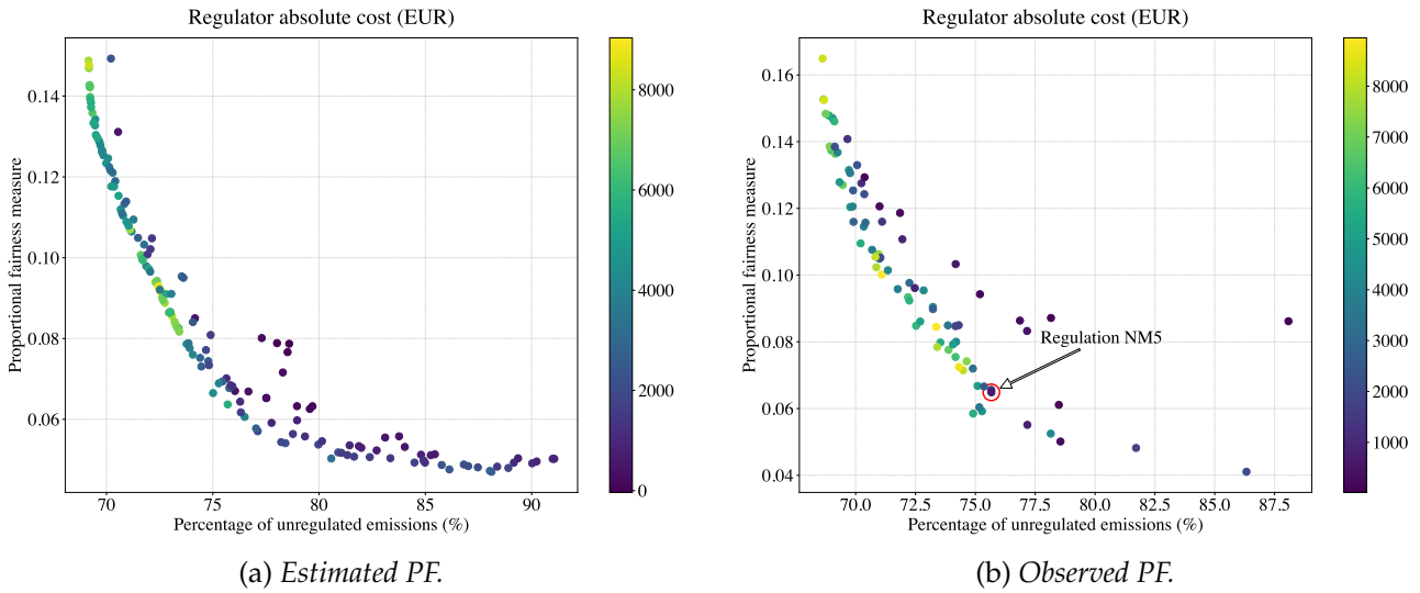
FIGURE 5.17 – Estimated and observed PF for the three objectives of the regulator on the non-motorized demand scenario.
